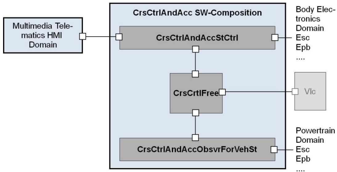
Figure 4.3: Example of SW-Composition CrsCtrlAndAcc in case of stand-alone free cruise control
