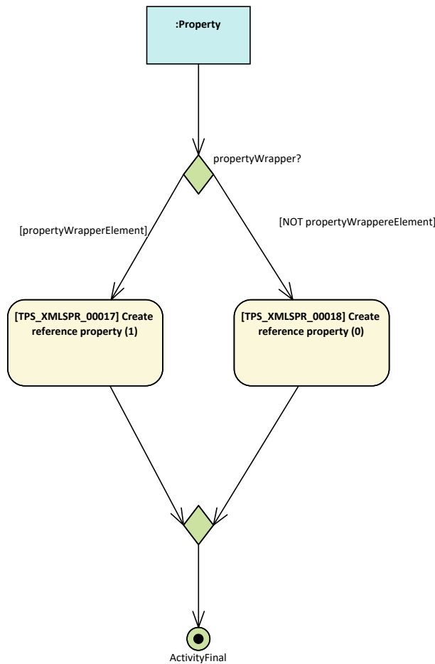
Figure 4.15: Property representation (aggregation = none)
