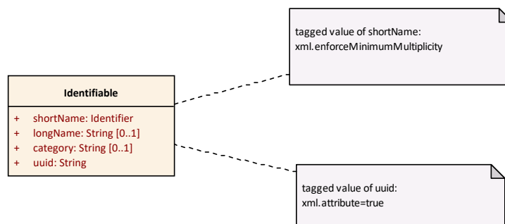
Figure 4.3: UML example - Create xsd:group
