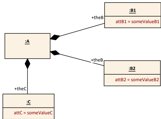
Figure 4.14: Example instance of composite property
