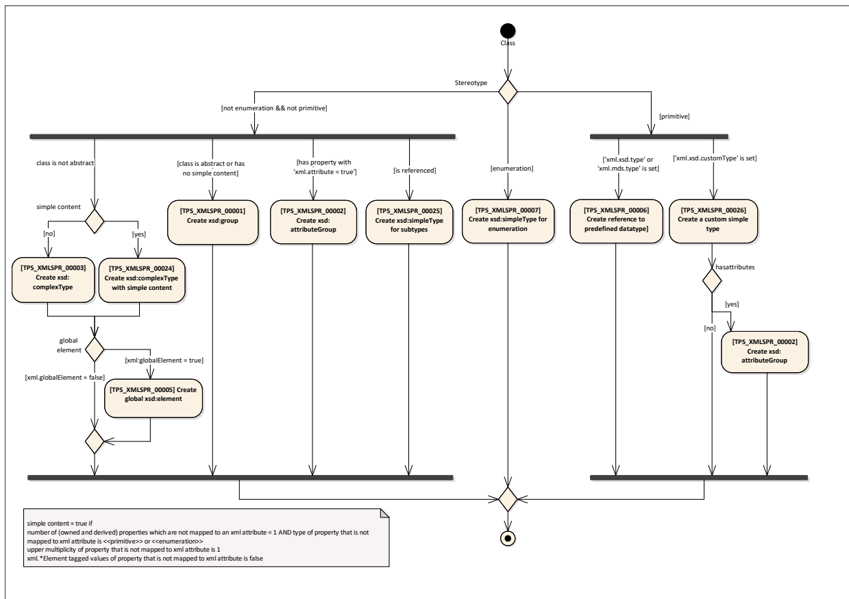
Figure 4.2: Class representation
