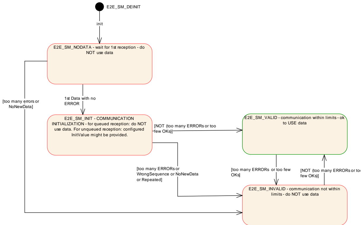
Figure 6.130: E2E state machine overview - [TransitToInvalid == 1]
