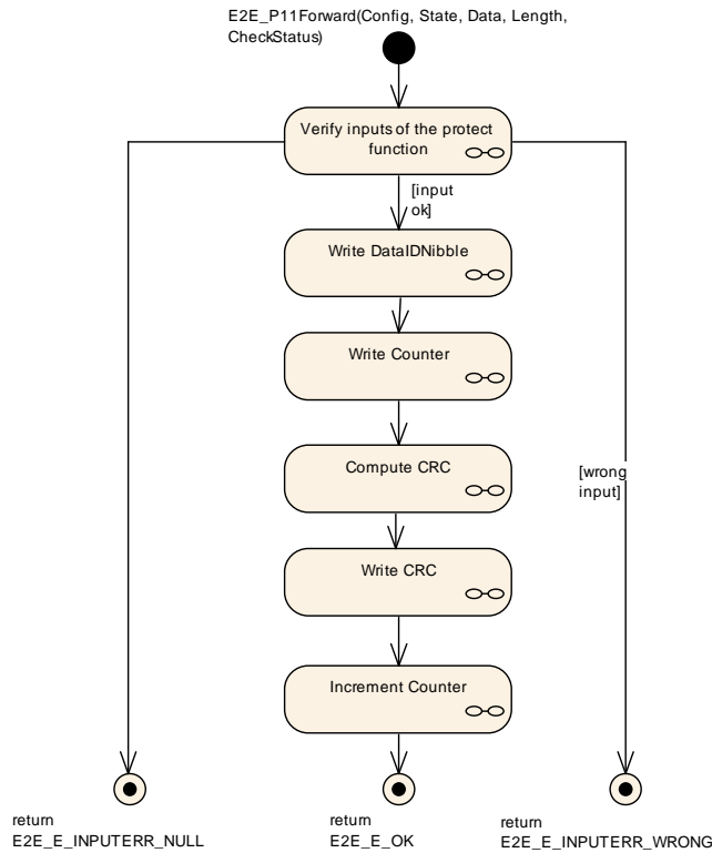
Figure 6.101: E2E Profile 11 Forward
