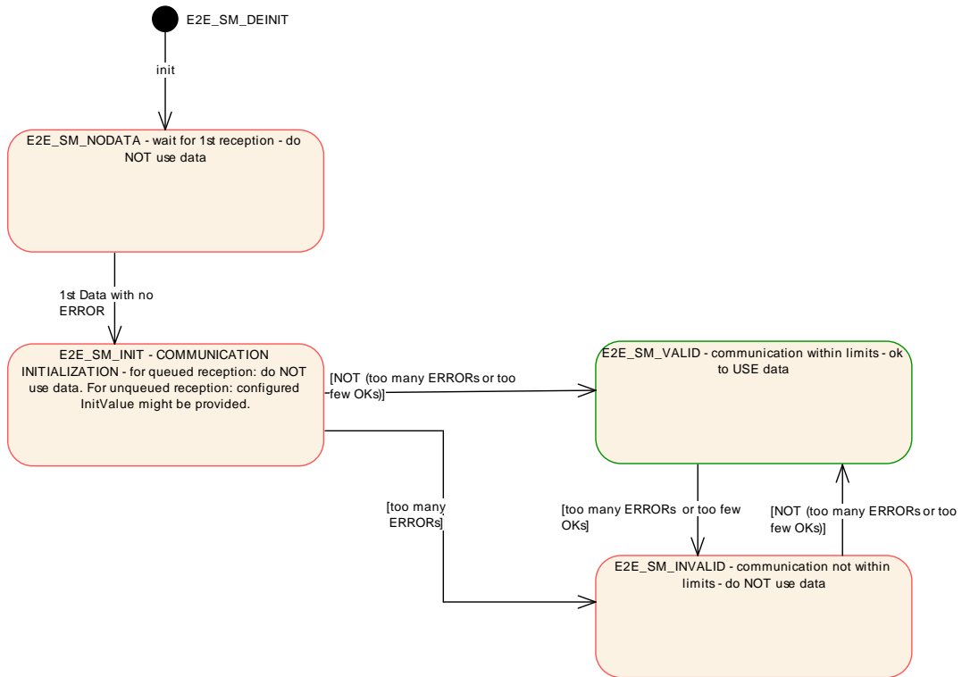
Figure 6.129: E2E state machine overview - [TransitToInvalid == 0]
