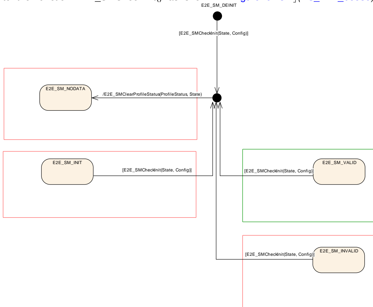
Figure 6.134: E2E state machine step E2E_SMCheckInit
