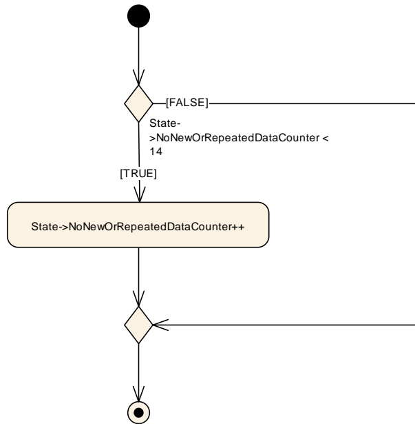
Figure 6.61: E2E Profile Check step "E2E_P01_process_NoNewOrRepeatedDataCounter"
