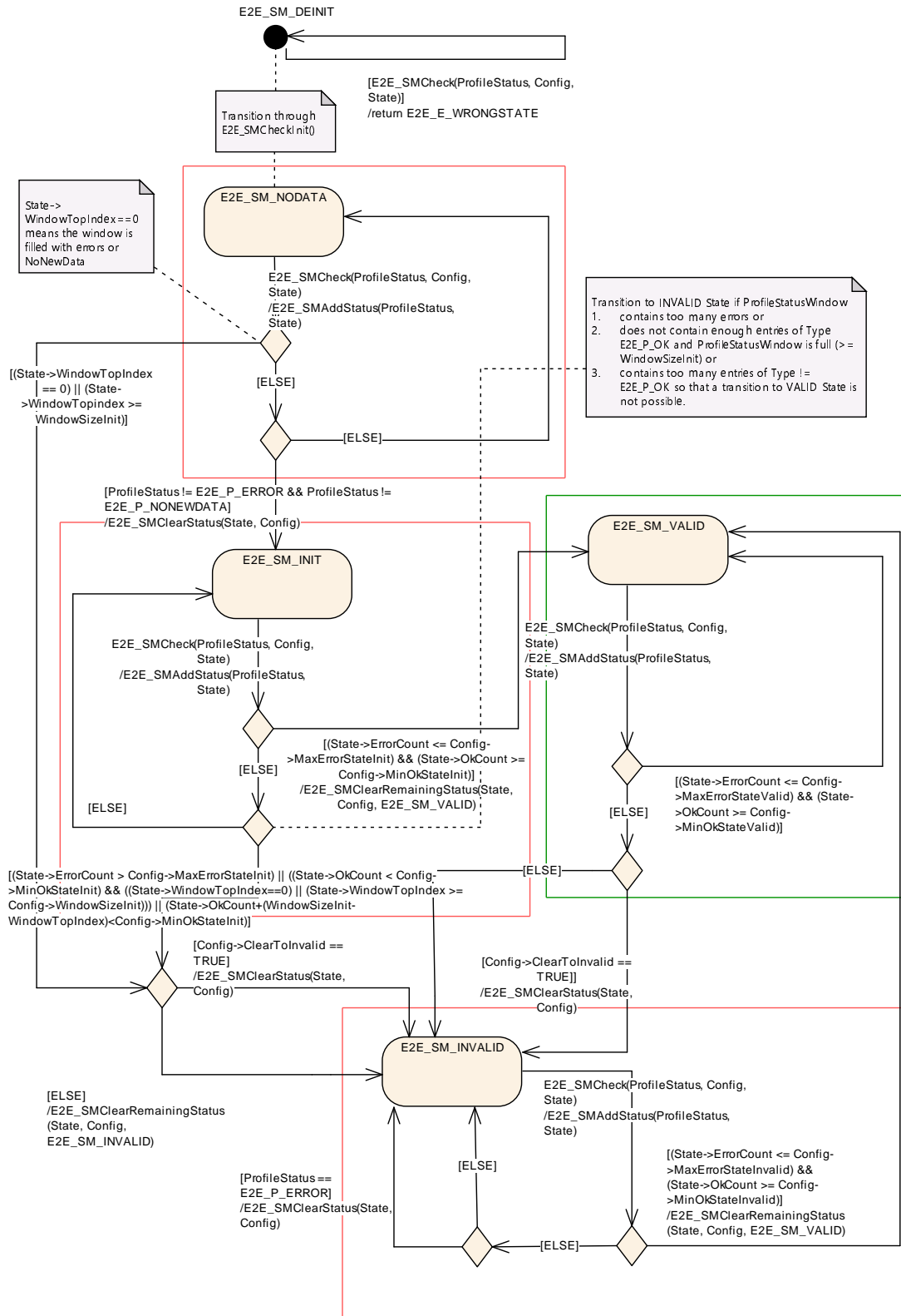
Figure 6.132: E2E state machine check - [TransitToInvalid == 1]
