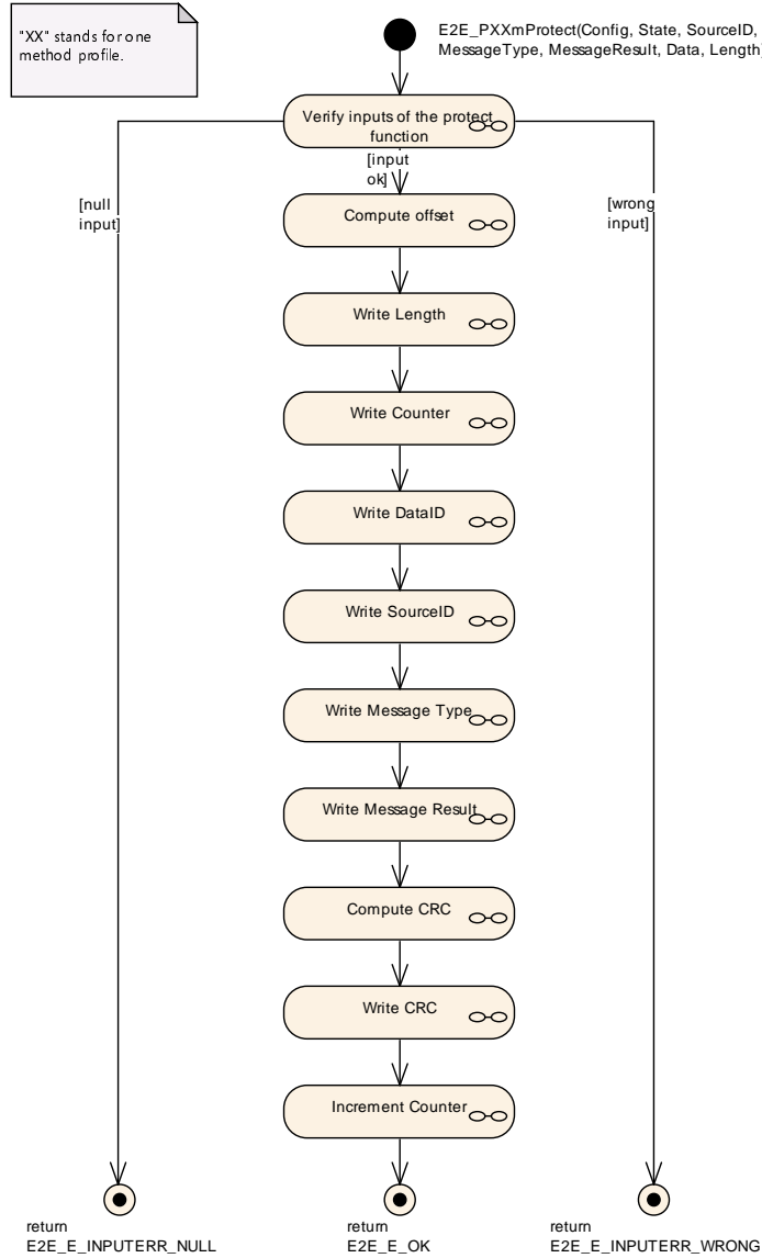
Figure 6.22: Behavior of E2E_PXXmProtect()
