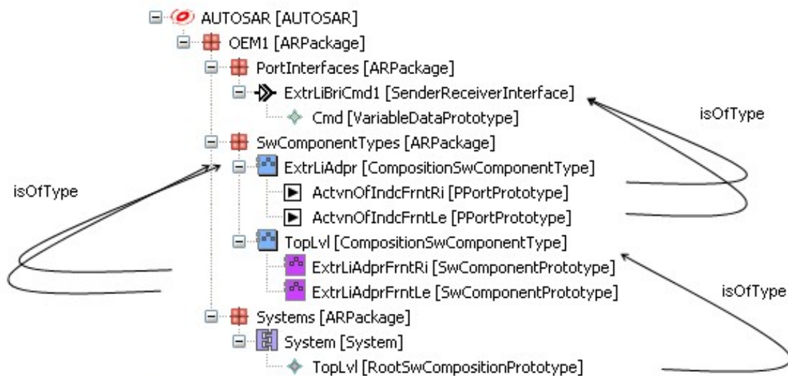
Figure 16.1: Example ExtrLi with Multiple Instantiation
