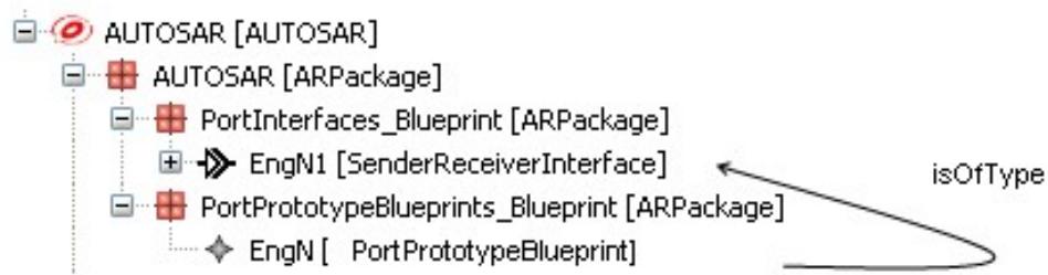
Figure 6.3: Example AUTOSAR Blueprints EngN
