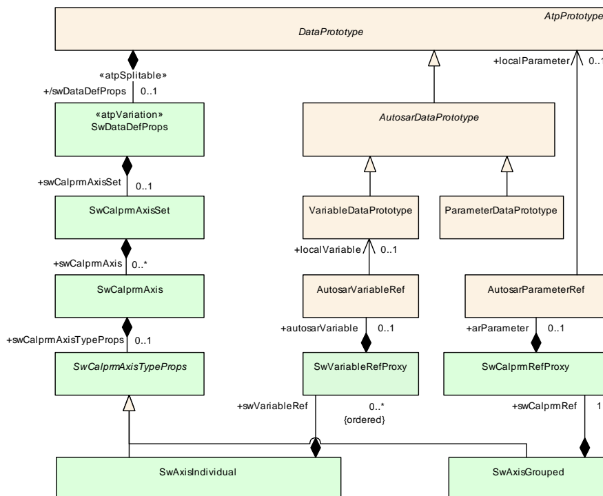
Figure 5.35: Extended Axis Elements and Input Variable Reference
