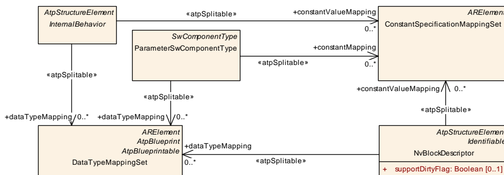
Figure 5.62: Relation between data type mapping and constant mapping
