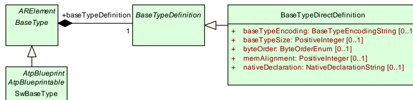
Figure 5.14: Base Type
