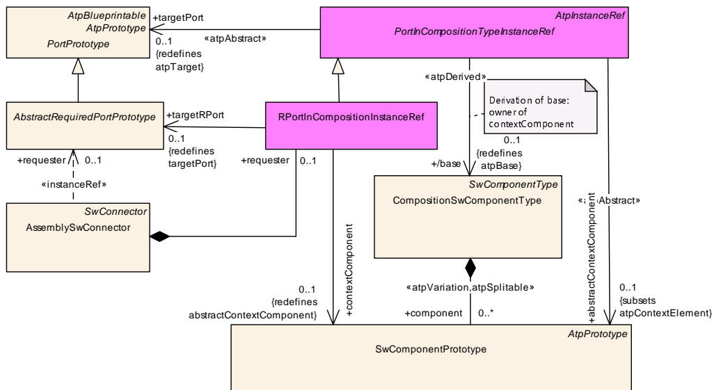
Figure D.16: Concrete modeling of references to RPortPrototype in the context of a CompositionSwComponentType
