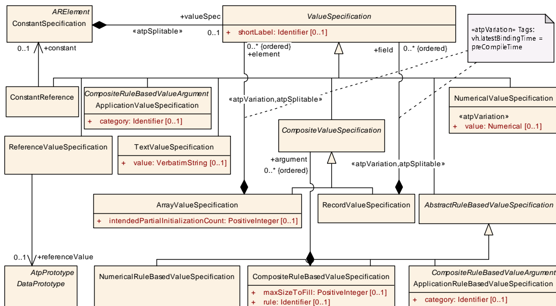
Figure 5.60: Summary of ValueSpecification
