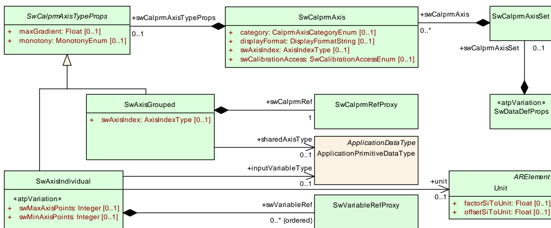
Figure 5.22: Modeling of SwAxisGrouped and SwAxisIndividual
