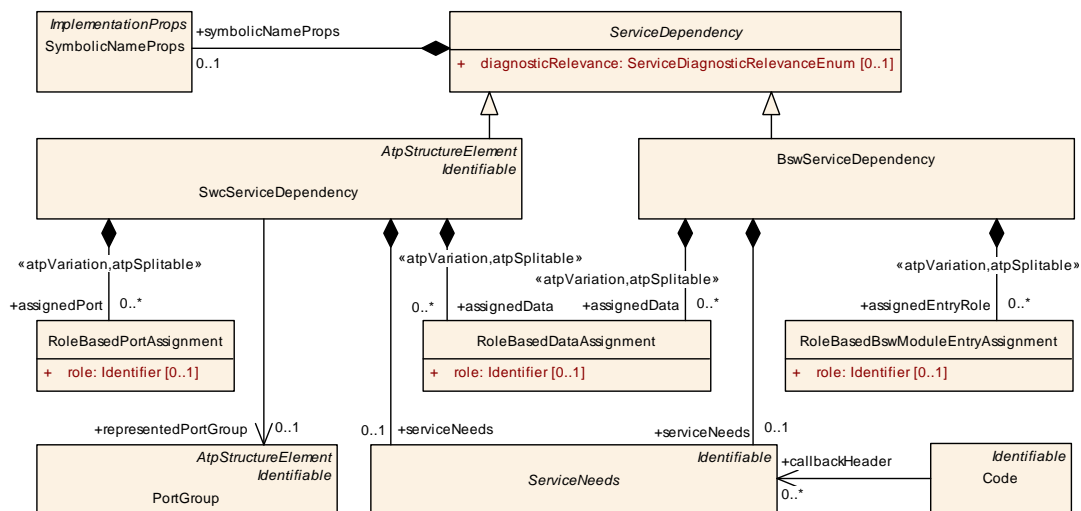
Figure 7.39: ServiceDependency is the abstract base class of SwcServiceDependency
