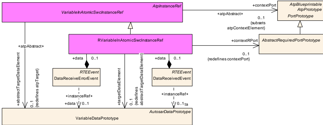
Figure D.2: Concrete modeling of references to VariableDataPrototype in the context of an RPortPrototype
