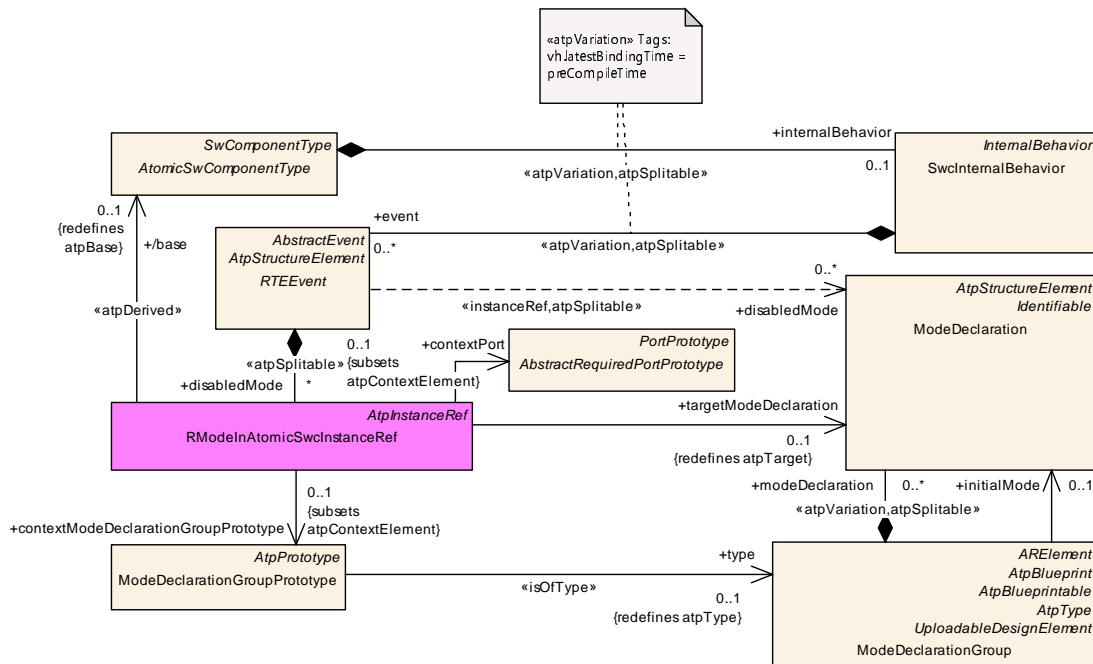
Figure D.32: Modeling of mode disabling
