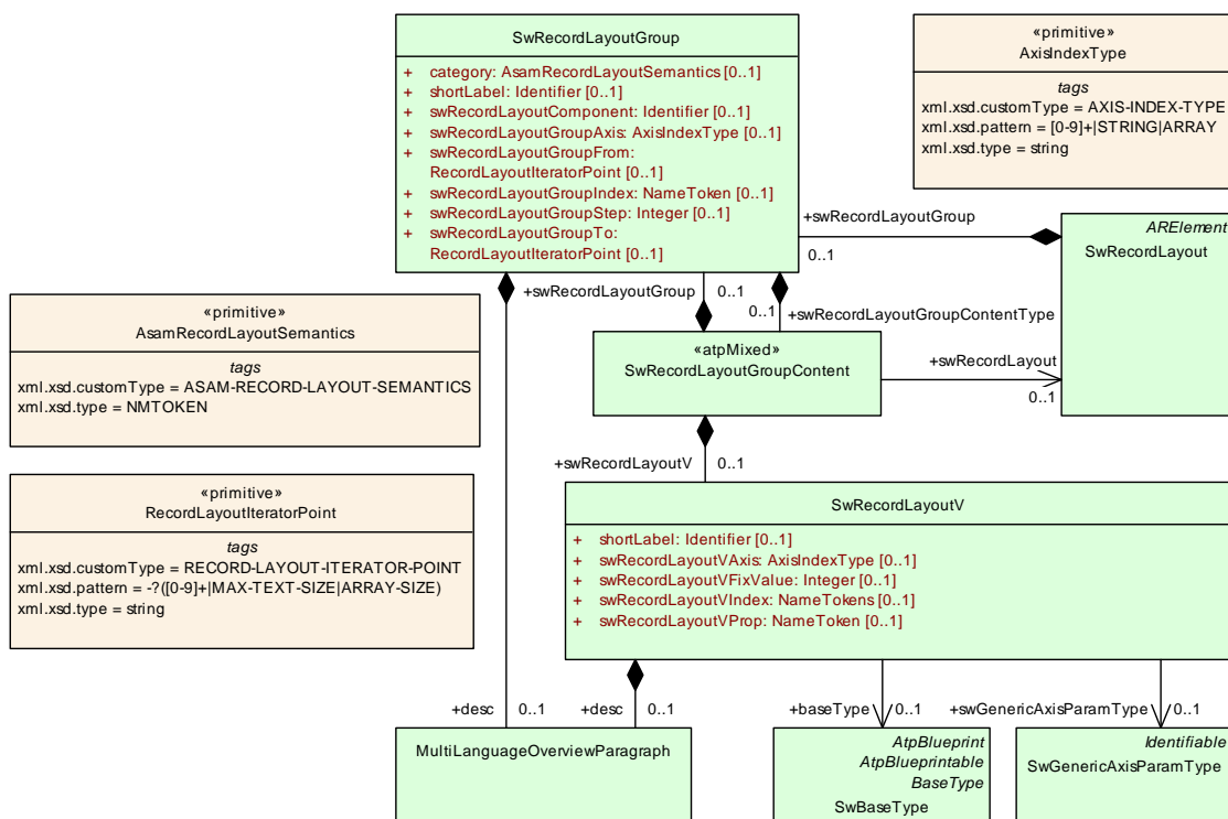
Figure 5.53: Specification of a record layout
