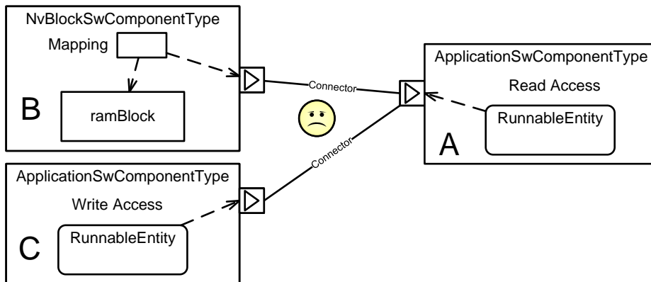
Figure B.45: Example invalid connection between software-components (a)
