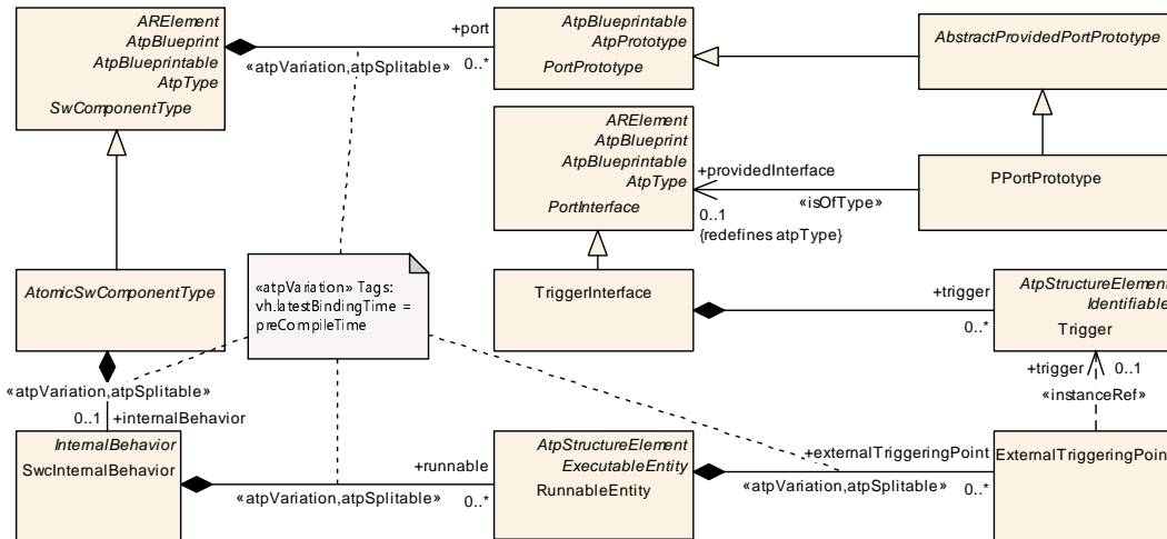
Figure 7.29: Model structure of a trigger source.
