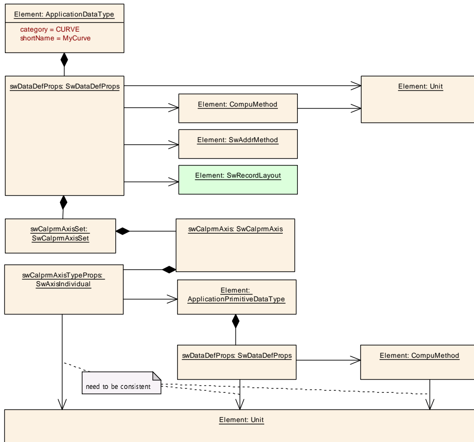
Figure 5.32: Illustration of a Curve in M1
