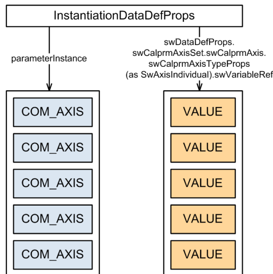
Figure 5.36: The n th COM_AXIS in the array of COM_AXIS s uses the n th VALUE in the array of VALUE s as working point.
