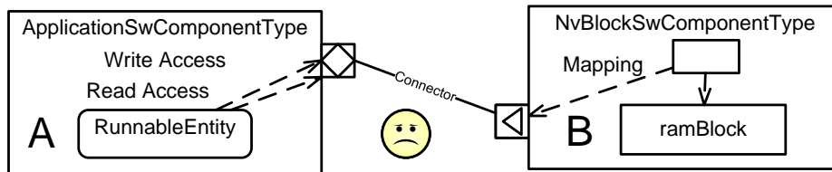
Figure B.47: Example invalid connection between software-components (c)
