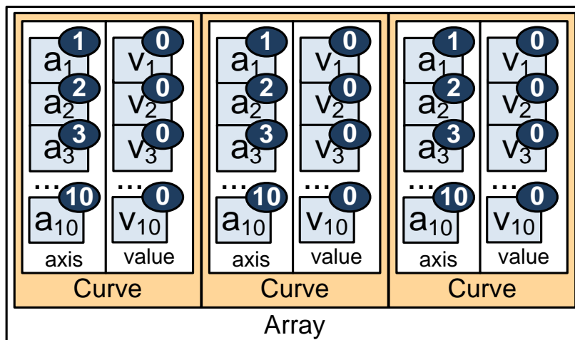
Figure B.30: Example of the initialization of an array of curve
