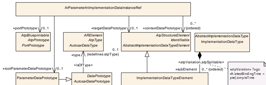
Figure 5.21: Implementation of ArParameterInImplementationDataInstanceRef
