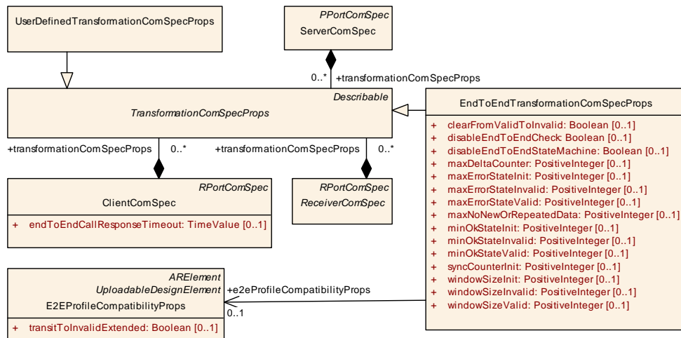
Figure 4.48: Specification of data transformation properties within ReceiverComSpec , ServerComSpec , and ClientComSpec
