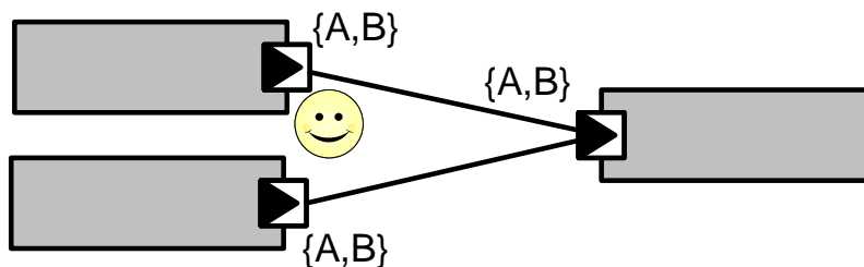
Figure B.32: legal n:1 communication
