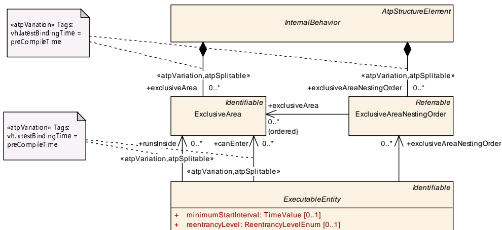
Figure 7.15: Description of nested usage of ExclusiveArea
