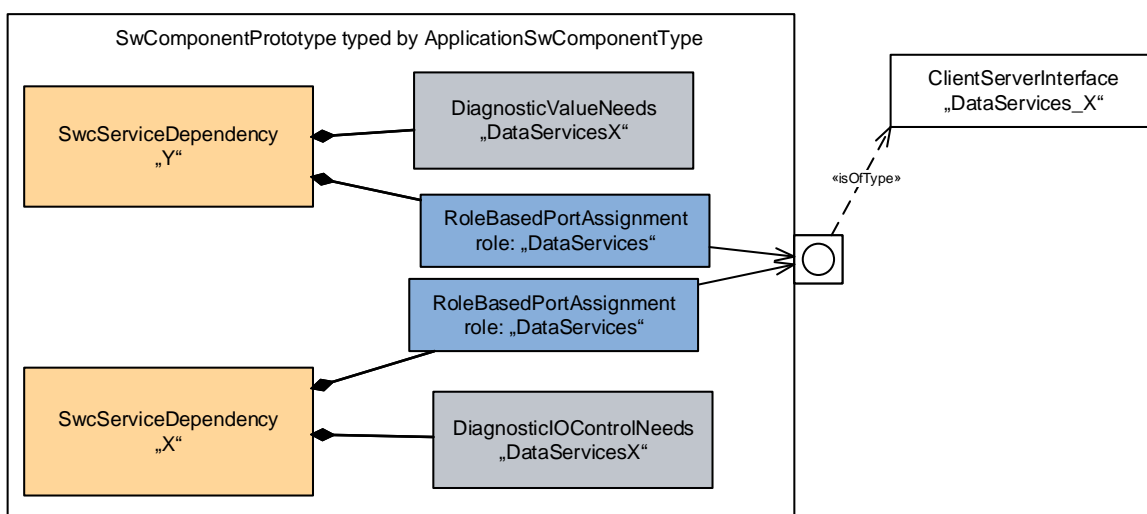
Figure 7.44: Two SwcServiceDependencies referencing one PortPrototype
