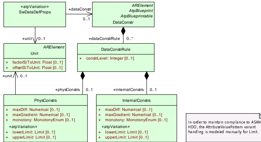
Figure 5.50: Meta-model for defining Data Constrains
