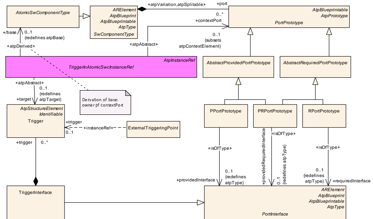
Figure D.5: Abstract modeling of references to Trigger in the context of a Atomic-SwComponentType
