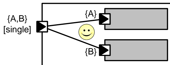
Figure B.36: Legal split of delegation connector
