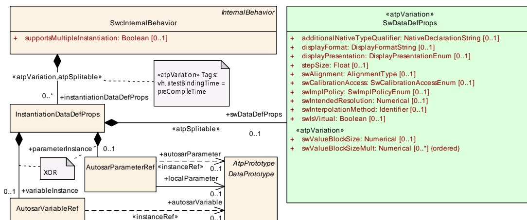
Figure 7.32: applying instantiation specific data definition properties
