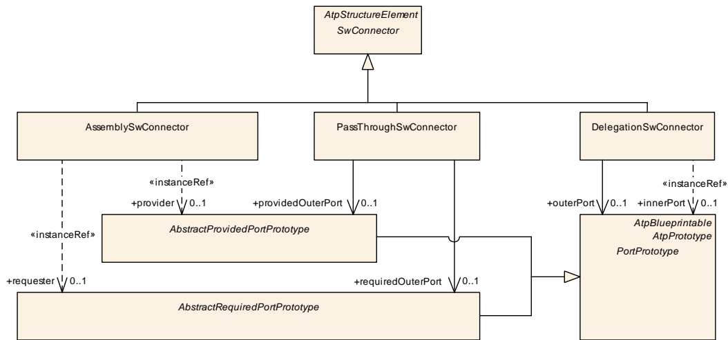
Figure 3.10: Connectors
