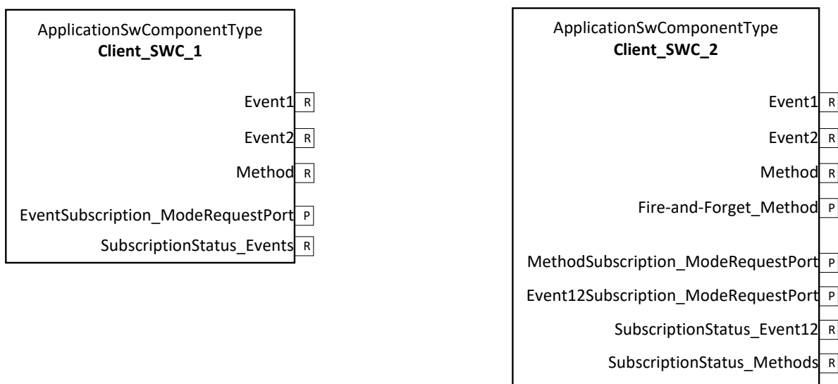
Figure 13.5: Client examples
