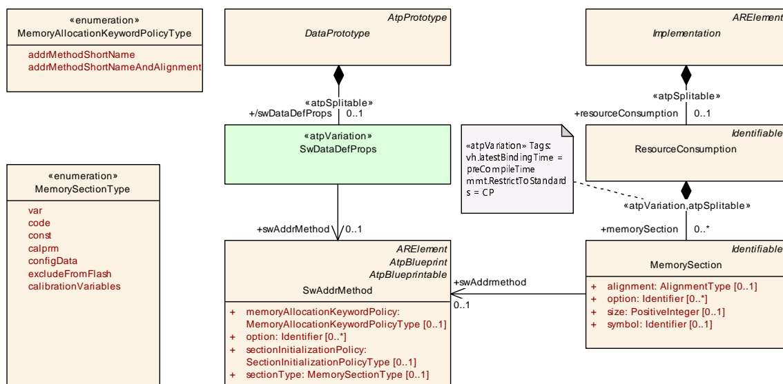
Figure 5.52: Assigning an address method to a memory section
