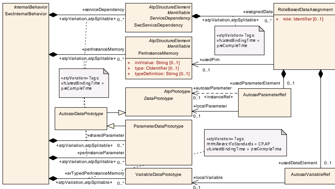
Figure 7.41: Details of RoleBasedDataAssignment for local data
