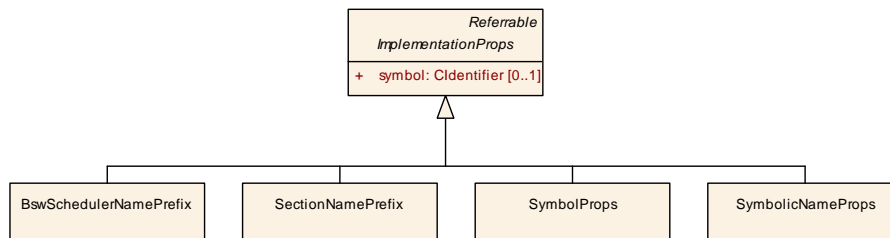
Figure 5.13: ImplementationProps and its subclasses
