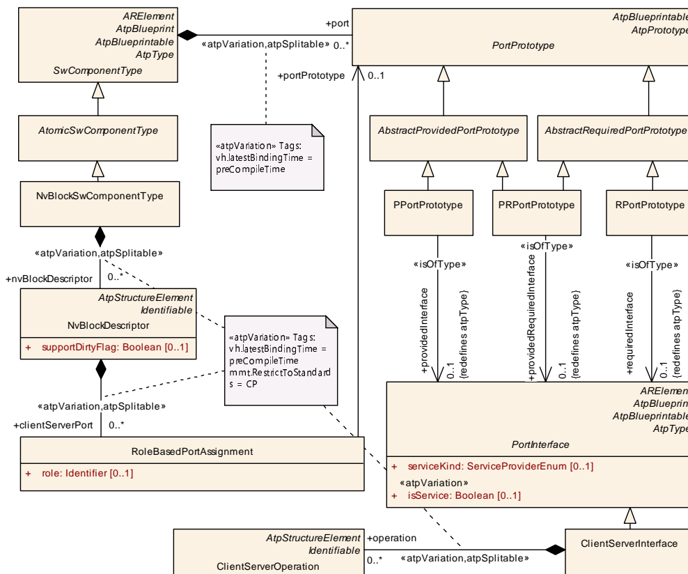
Figure 11.18: NvBlockNotification
