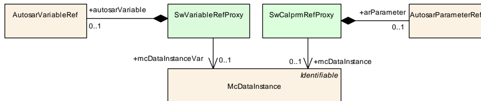
Figure 5.40: Proxy reference classes
