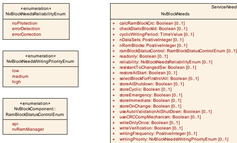
Figure 11.12: NvBlockNeeds
