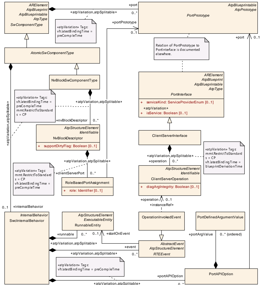
Figure 11.20: NvBlockSwComponentType and SwcInternalBehavior
