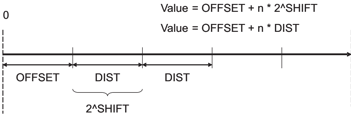
Figure 5.55: Values for swRecordLayoutVProp for fixed axis
