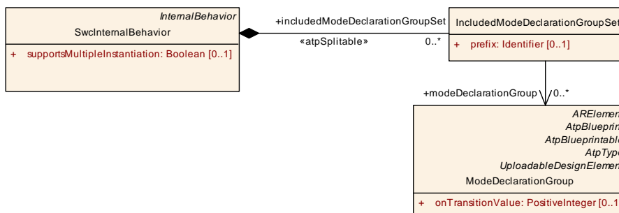
Figure 7.37: Included ModeDeclarationGroups
