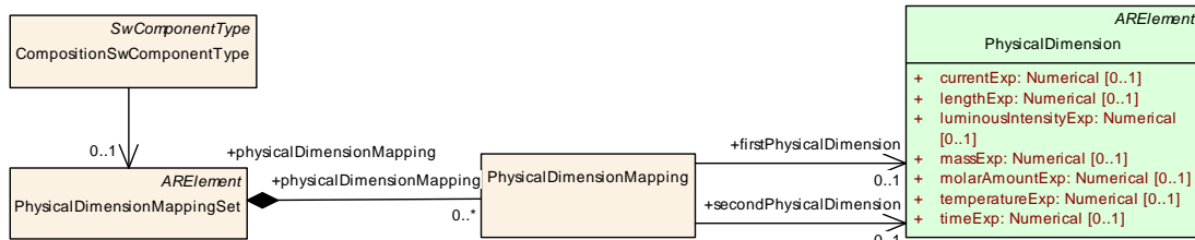
Figure 5.46: Modeling of PhysicalDimensionMapping
