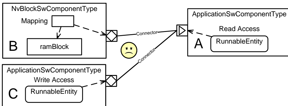
Figure B.46: Example invalid connection between software-components (b)
