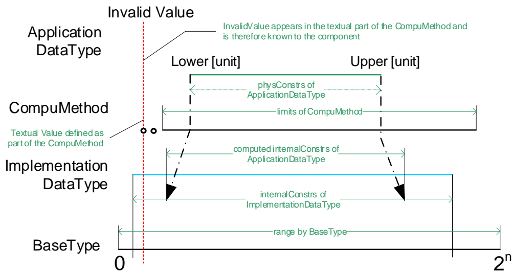
Figure 5.26: Value ranges and invalid values with discrete invalidValue defined inside the scope of the CompuMethod
