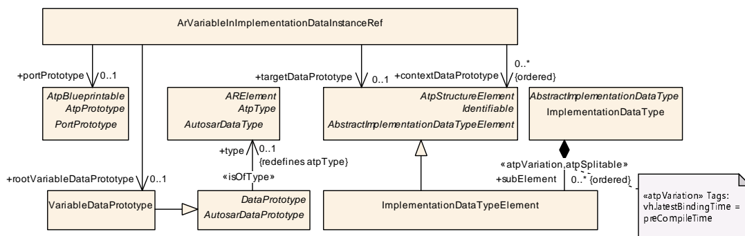
Figure 5.20: Implementation of ArVariableInImplementationDataInstanceRef
