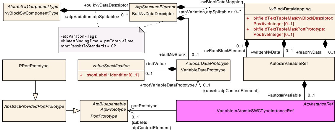
Figure 11.19: NvBlockSwComponentType and BulkNvDataDescriptor
