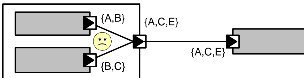
Figure B.43: Illegal merge of delegation connector
