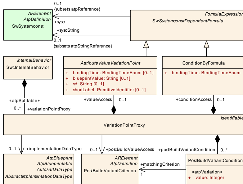
Figure 7.45: VariationPointProxy
