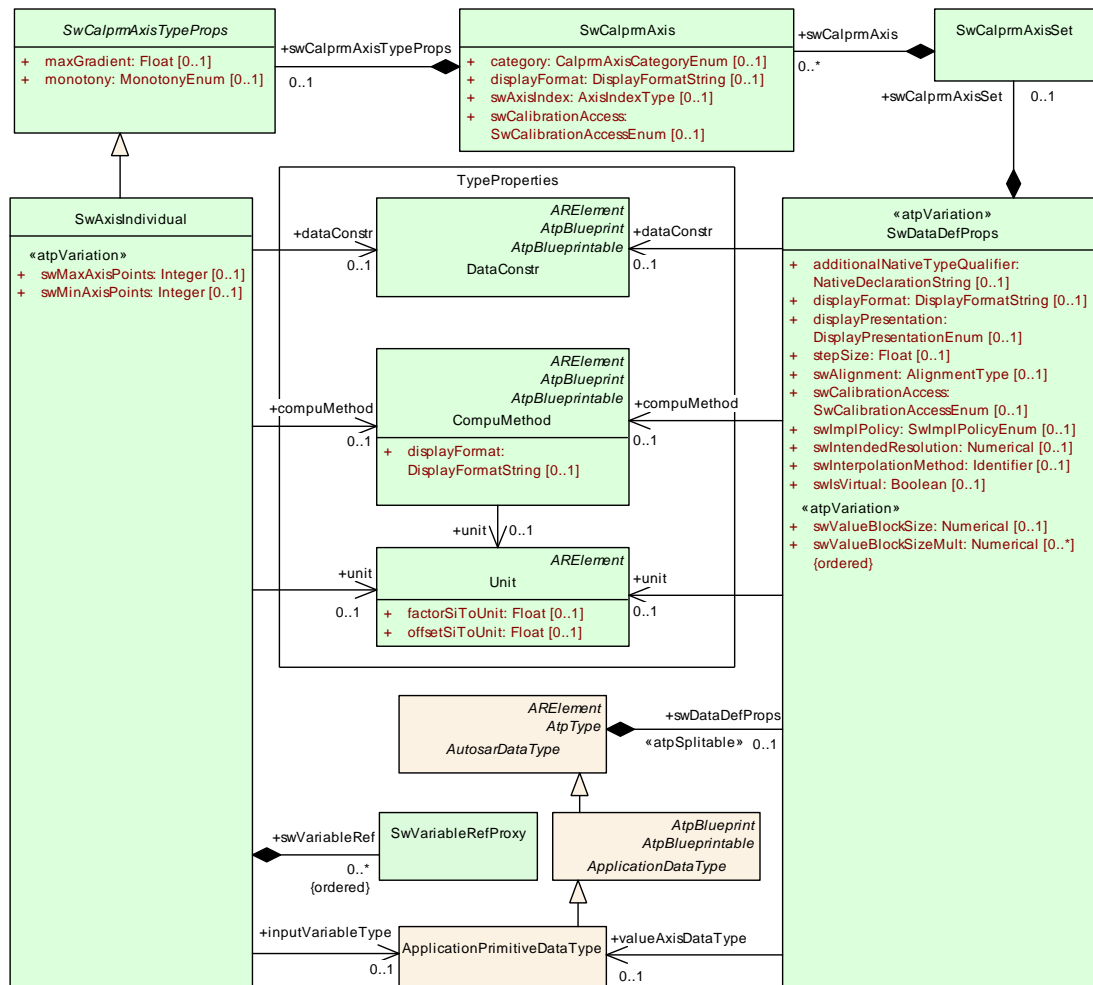
Figure 5.43: Various Attributes in the Context of SwDataDefProps
