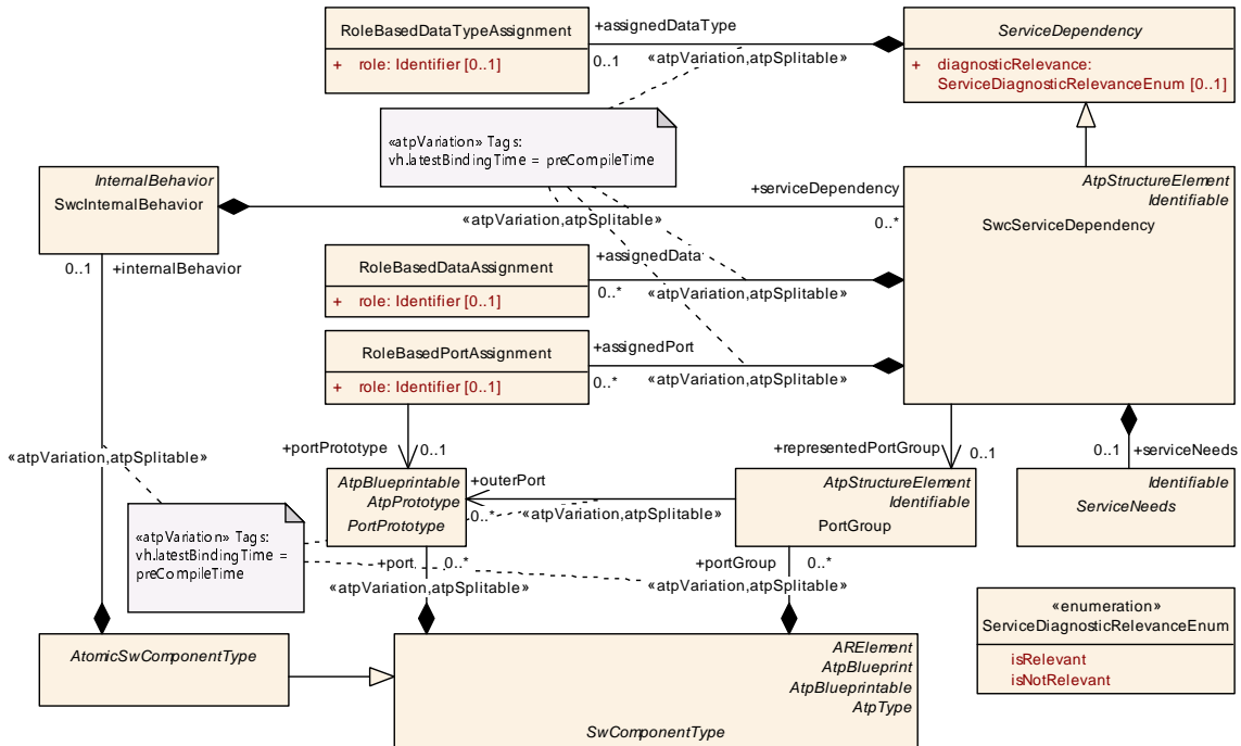
Figure 7.40: SwcServiceDependency in the SwcInternalBehavior
