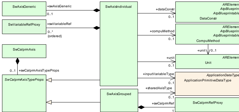
Figure 5.29: Overview on the Meta-Model for Axis Description
