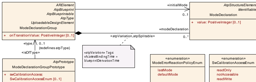
Figure 9.1: ModeDeclaration
