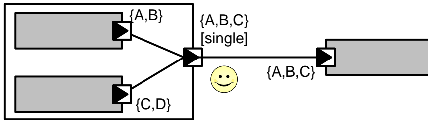
Figure B.39: Legal merge of delegation connector
