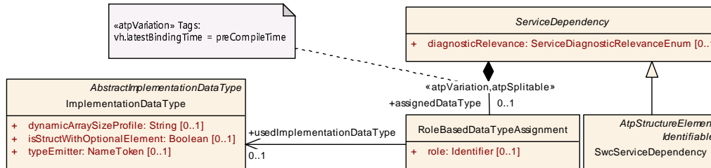
Figure 7.43: Details of RoleBasedDataTypeAssignment for local data
