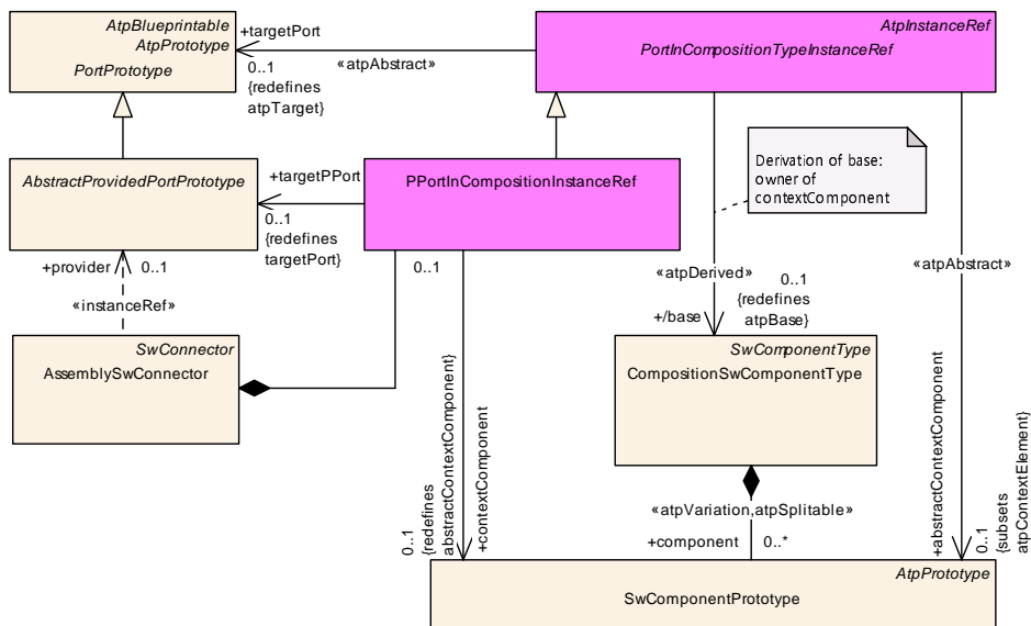
Figure D.15: Concrete modeling of references to PPortPrototype in the context of a CompositionSwComponentType
