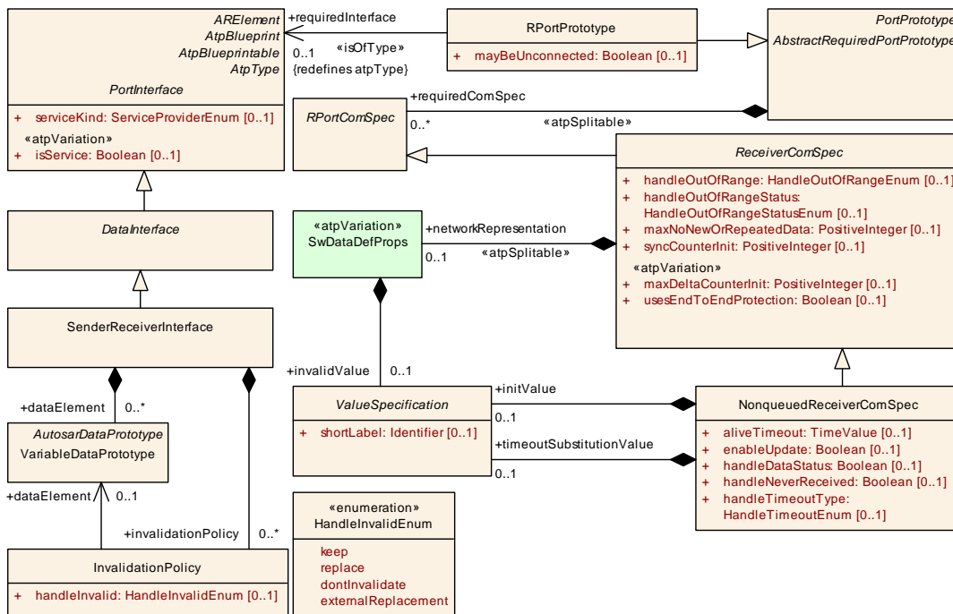
Figure 5.28: Relationships required to consider the invalidValue
