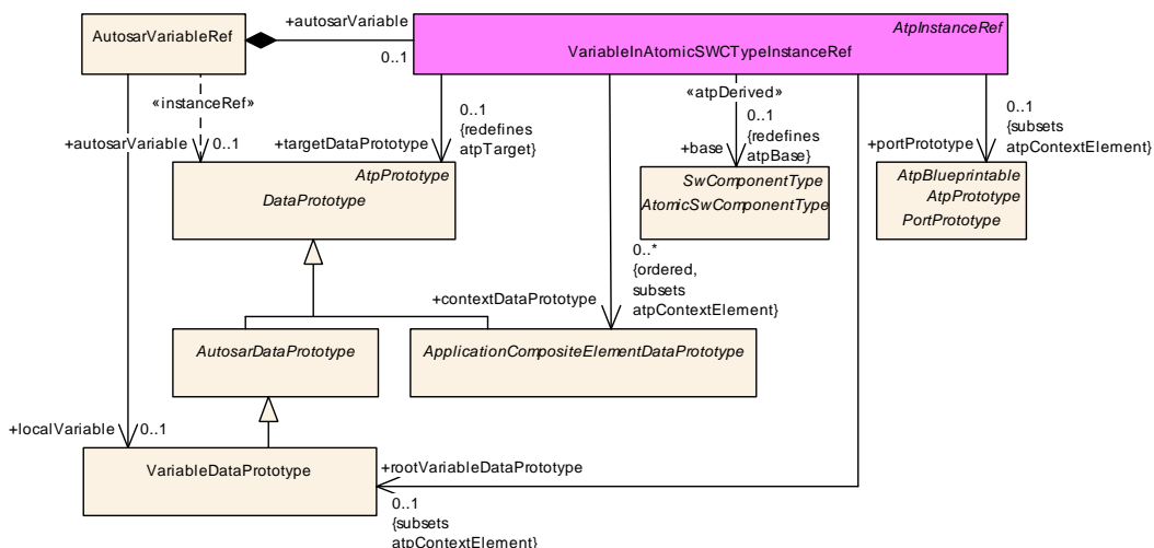
Figure 5.19: Implementation of the InstanceRef for AutosarVariableRef
