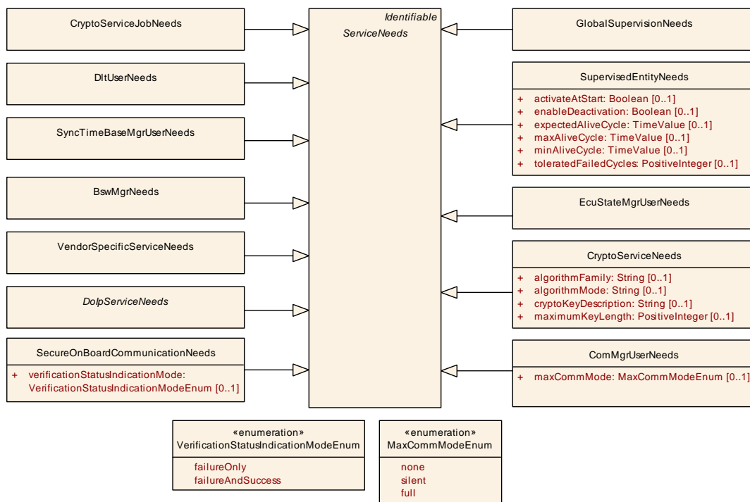
Figure 7.38: Meta-class ServiceNeeds and some of its specializations
