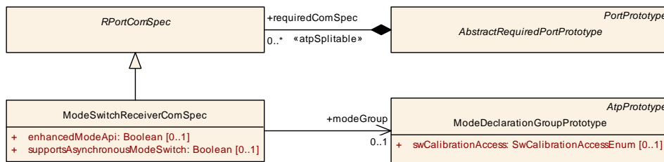
Figure 4.43: Communication attributes of PRPortPrototype with respect to mode switch communication.
