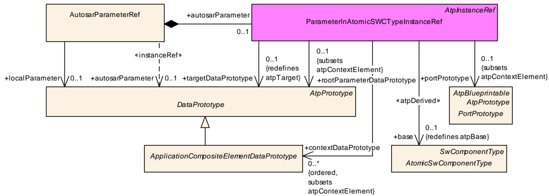
Figure 5.18: Implementation of the InstanceRef for AutosarParameterRef
