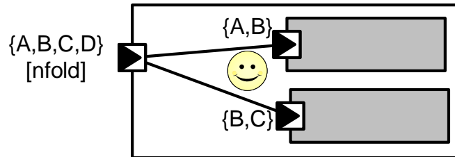
Figure B.35: Legal split of delegation connector
