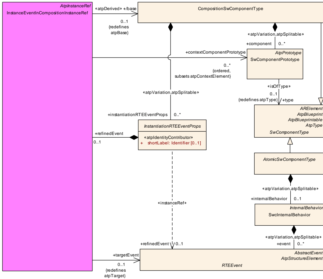
Figure D.23: Modeling of references to RTEEvent in the context of a InstantiationRTEEventProps from the point of view of a CompositionSwComponentType
