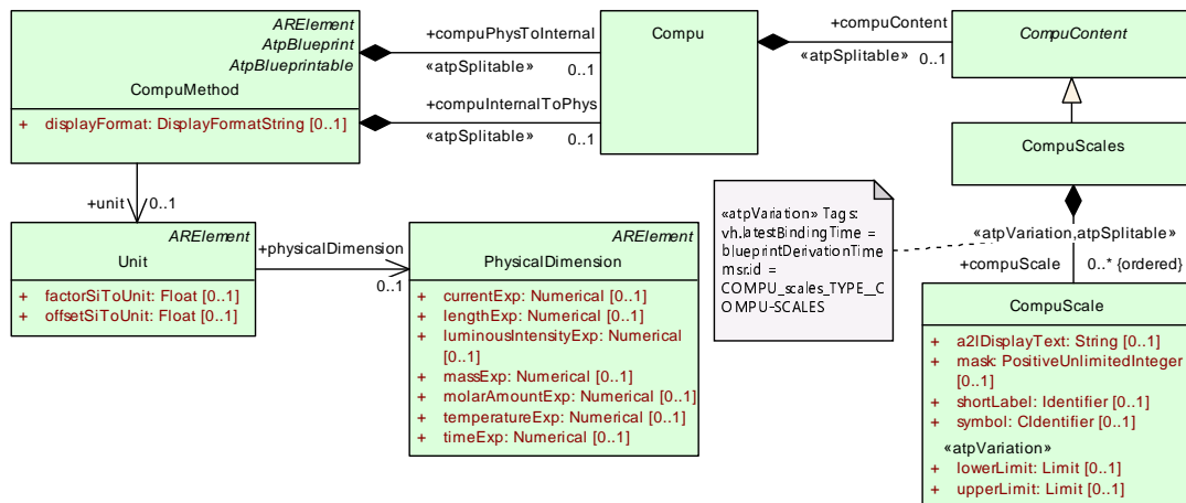
Figure 5.44: A CompuMethod and its attributes define data semantics
