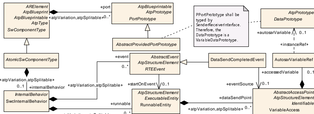
Figure 7.22: DataSendPoint
