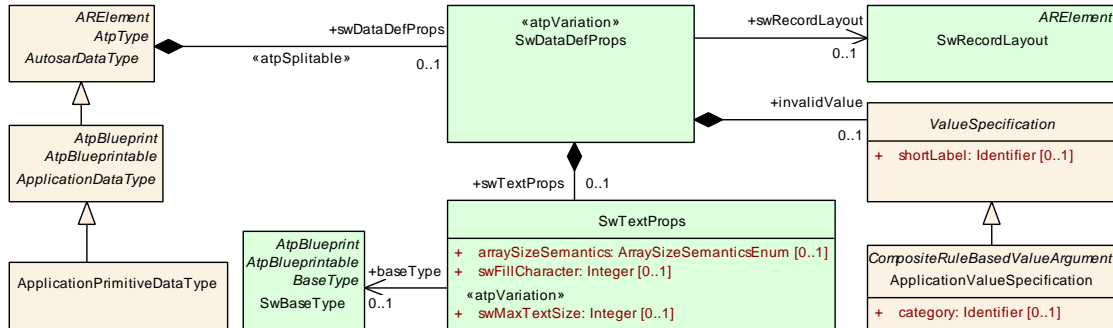
Figure 5.8: Specification of textual strings
