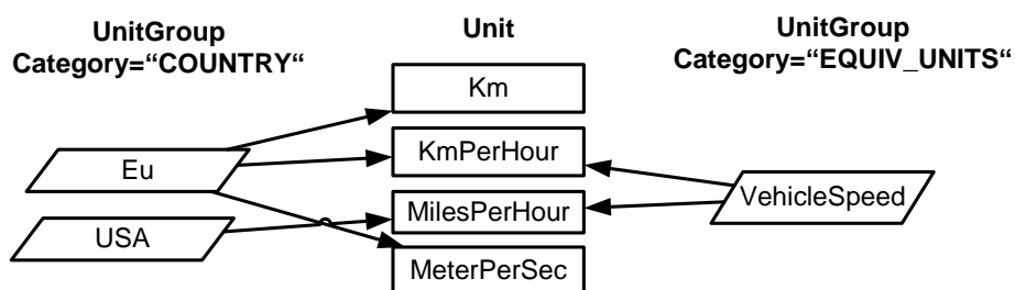
Figure 5.49: Example for units and unit groups
