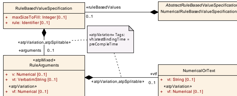
Figure 5.66: Definition of a NumericalRuleBasedValueSpecification
