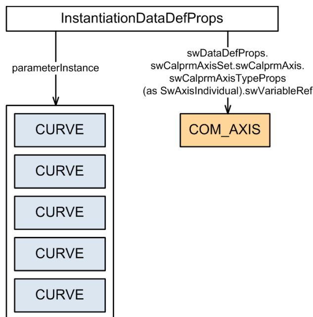
Figure 5.42: Each MAP in the array of CURVES uses the identical COM_AXIS
