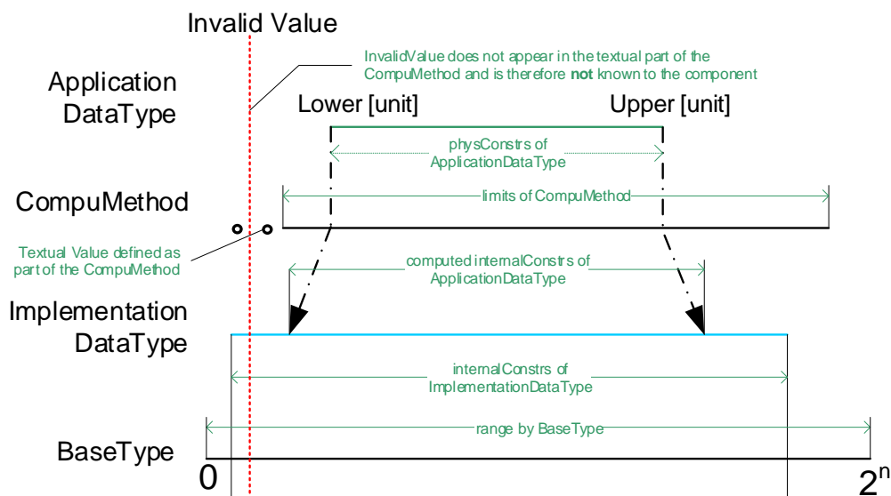
Figure 5.27: Value ranges and invalid values with discrete invalidValue defined outside the scope of the CompuMethod
