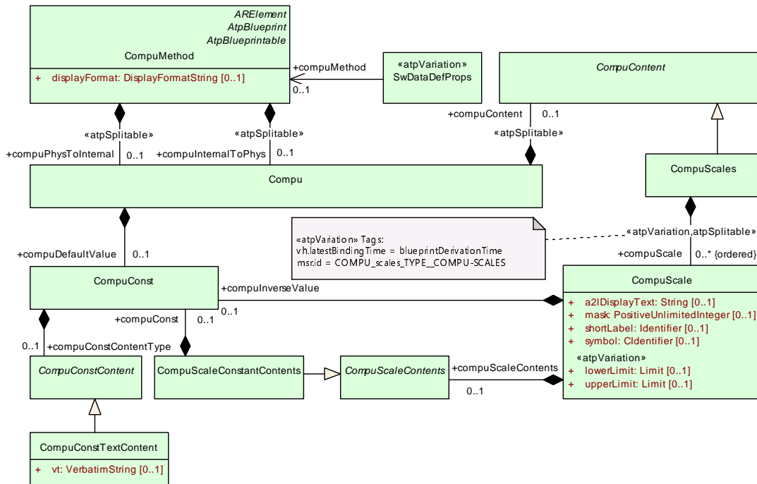
Figure 5.7: Relevant meta-classes for the specification of enumerations
