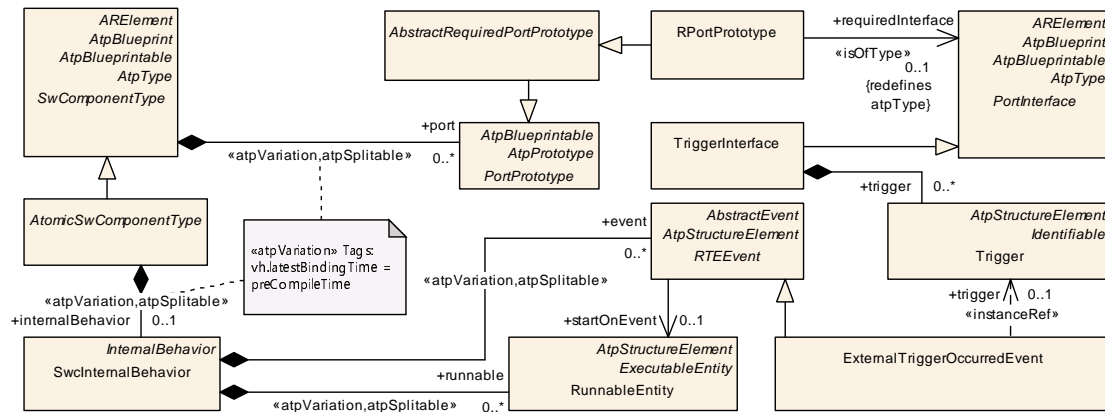
Figure 7.30: Model structure of a trigger sink
