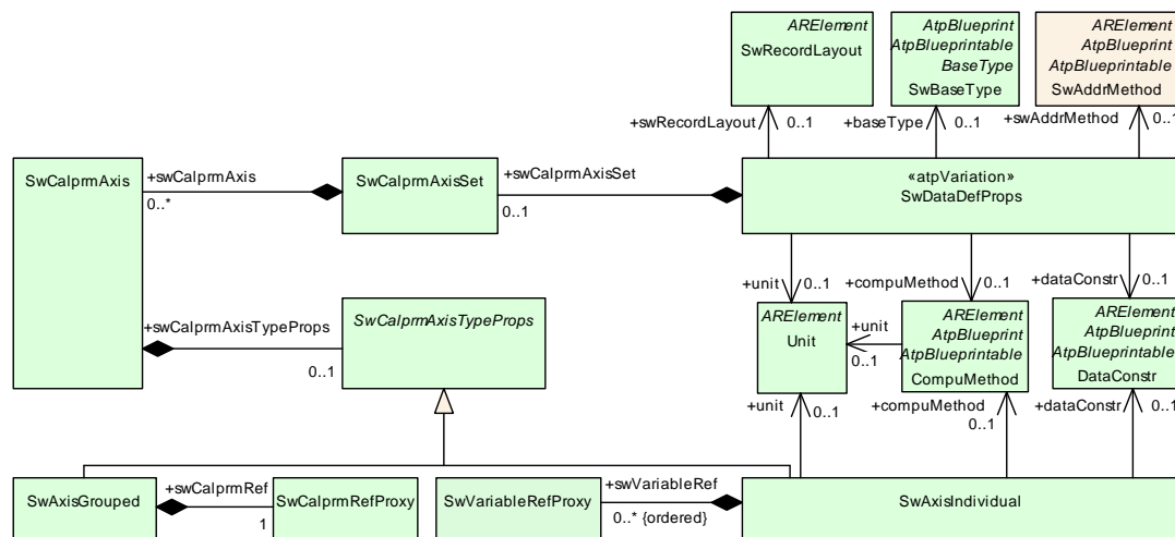
Figure 5.31: Meta-Model Elements used for a Curve
