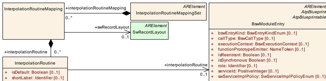
Figure 5.59: Mapping of Record Layouts and Interpolation Routines
