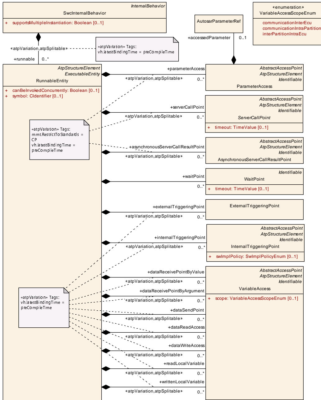
Figure 7.3: Details of RunnableEntity
