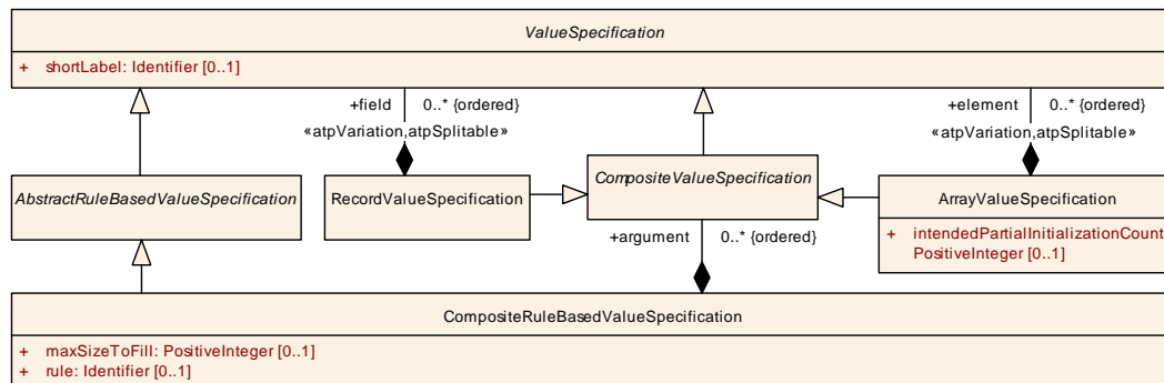
Figure 5.67: Rule-based value specification of arrays of a composite data type
