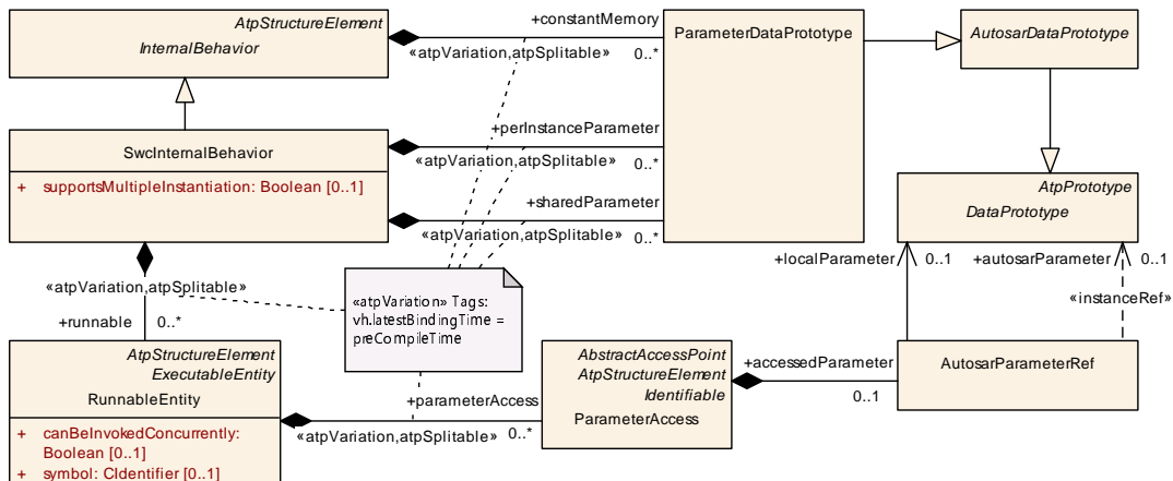
Figure 2.3: ParameterDataPrototypes in internal behavior
