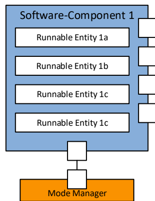
Figure 9.3: State Managers and software-components
