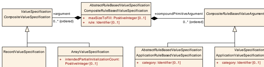
Figure 5.68: Rule-based value specification for compound primitive data objects
