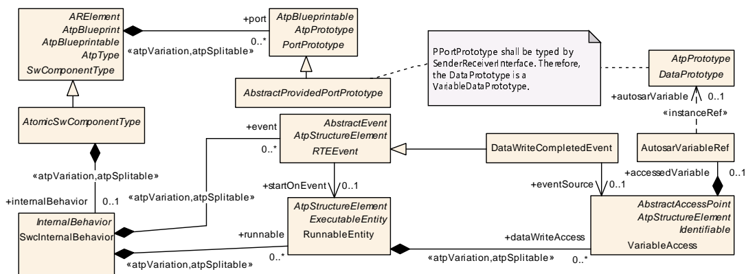
Figure 7.24: DataWriteAccess
