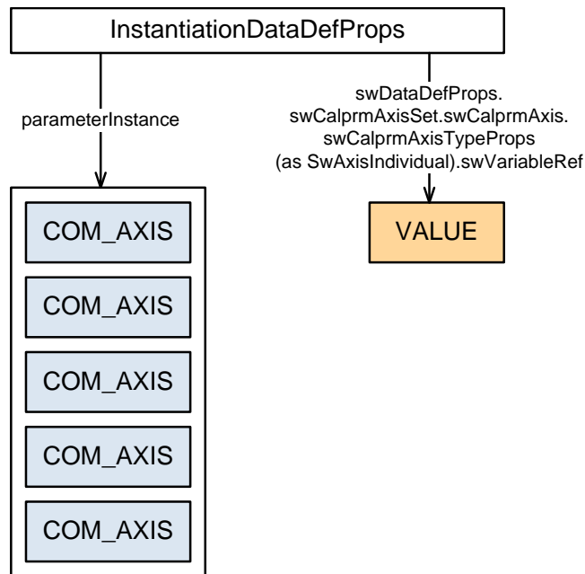
Figure 5.37: Each COM_AXIS in the array of COM_AXIS s uses the identical VALUE as working point.
