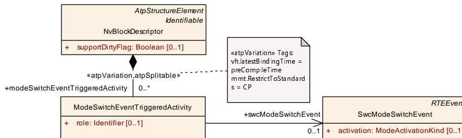
Figure 11.8: Usage of mode switch notification for the activation of a write-procedure of nv data
