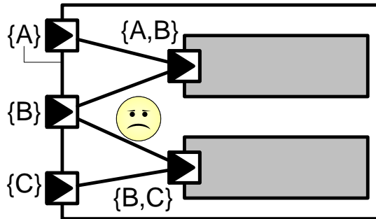
Figure B.41: Illegal split of delegation connector
