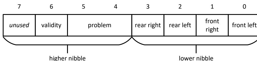
Figure B.31: Visualization of the layout of the example bitfield
