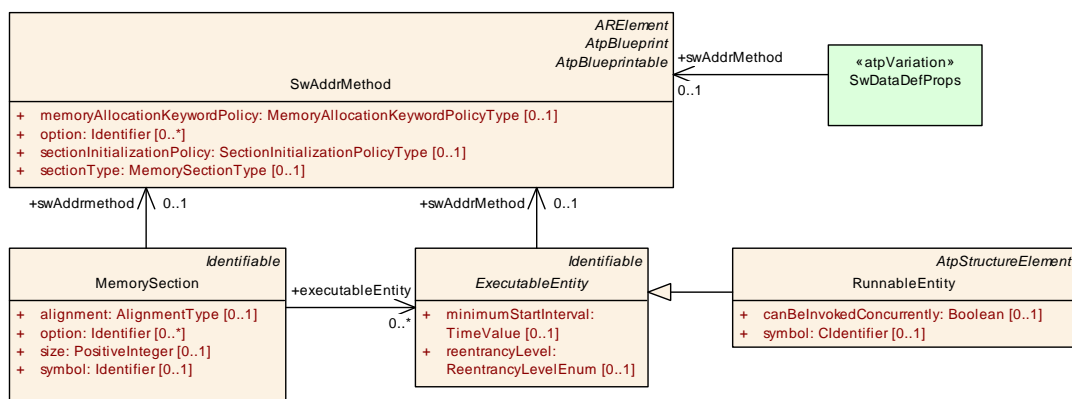
Figure 5.51: SwAddrMethod
