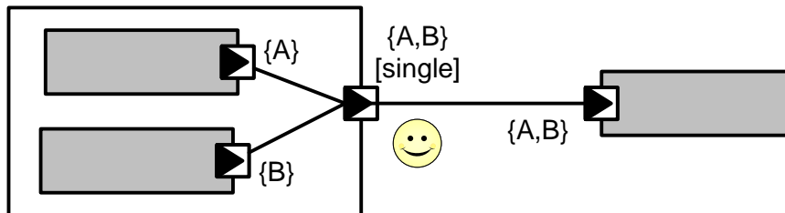
Figure B.37: Legal merge of delegation connector
