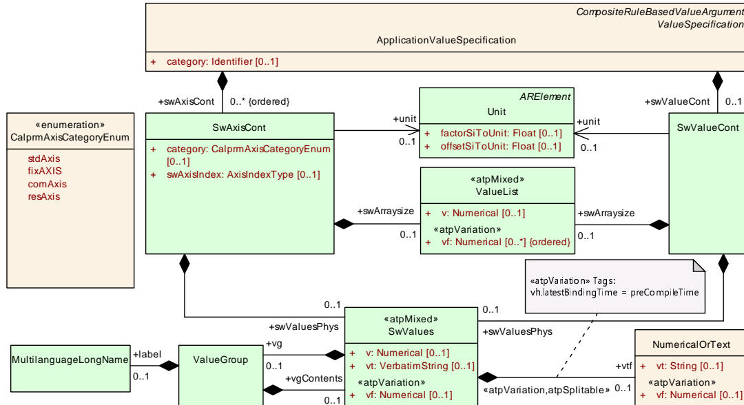
Figure 5.64: Definition of an ApplicationValueSpecification
