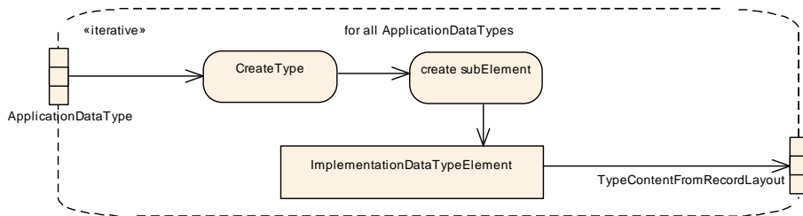
Figure 5.57: algorithm to map the details of an application data type to the corresponding implementation data type according to the record layout
