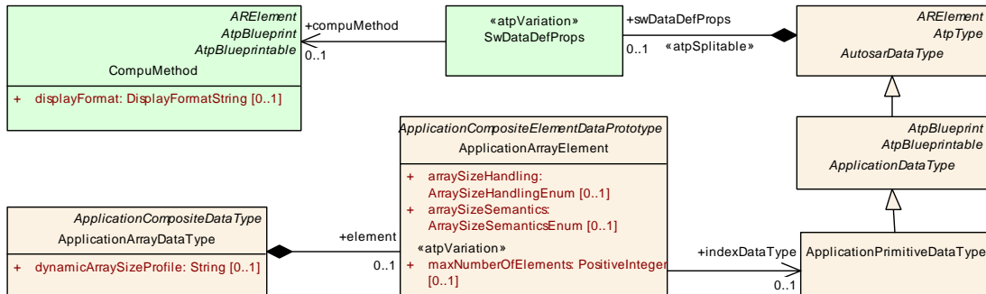
Figure 5.10: Modeling of the ApplicationArrayElement.indexDataType
