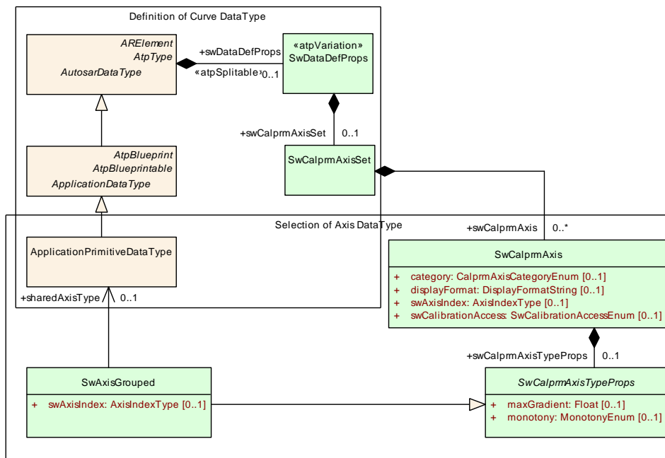
Figure 5.33: Definition of an ApplicationPrimitiveDataType that implements a curve
