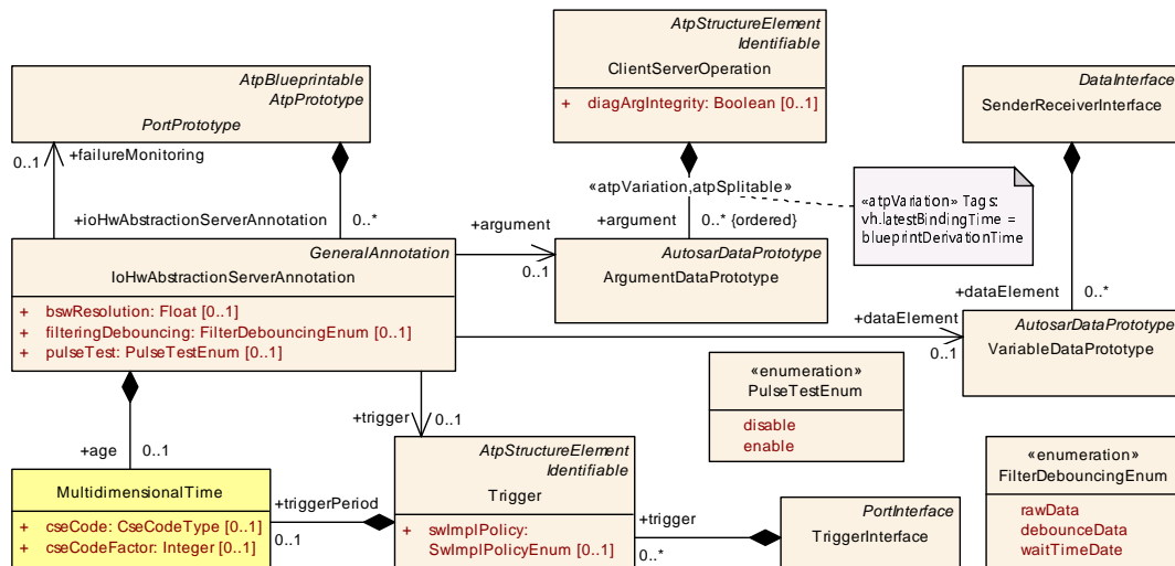
Figure 4.28: IoHwAbstractionServerAnnotation
