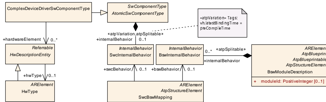
Figure 10.8: ComplexDeviceDriverSwComponentType
