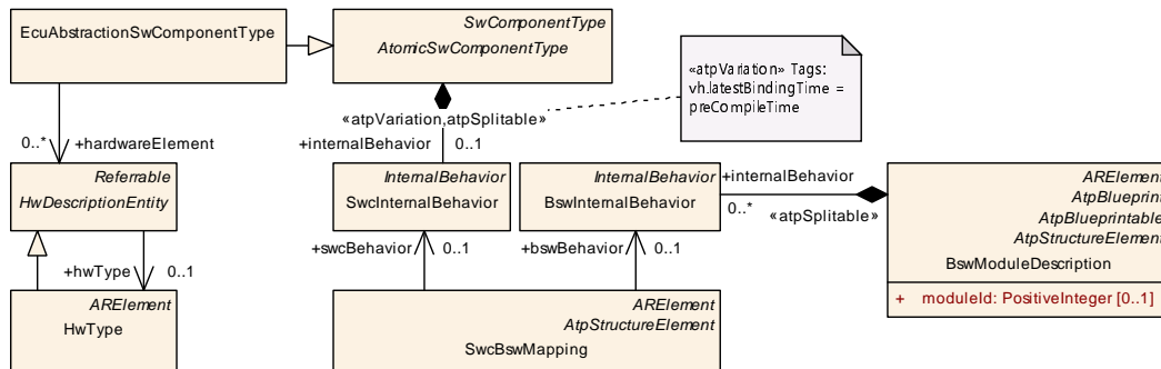
Figure 10.7: EcuAbstractionSwComponentType
