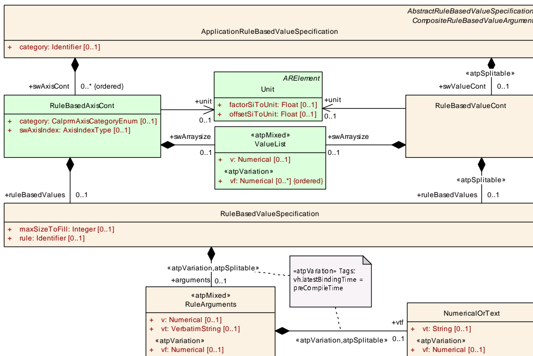
Figure 5.65: Definition of an ApplicationRuleBasedValueSpecification
