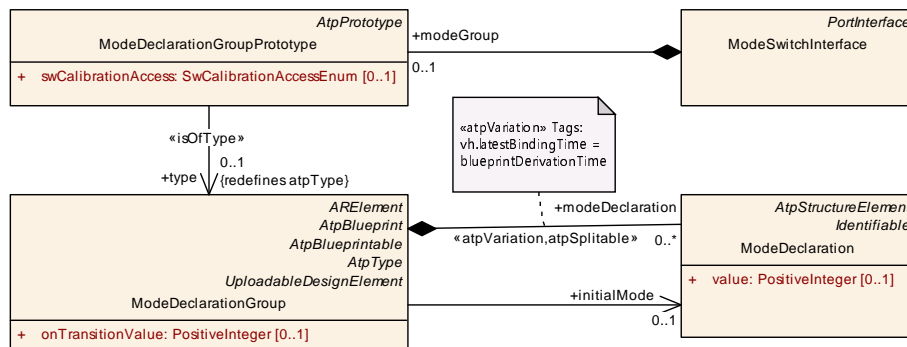
Figure 4.8: Mode Switch Interface
