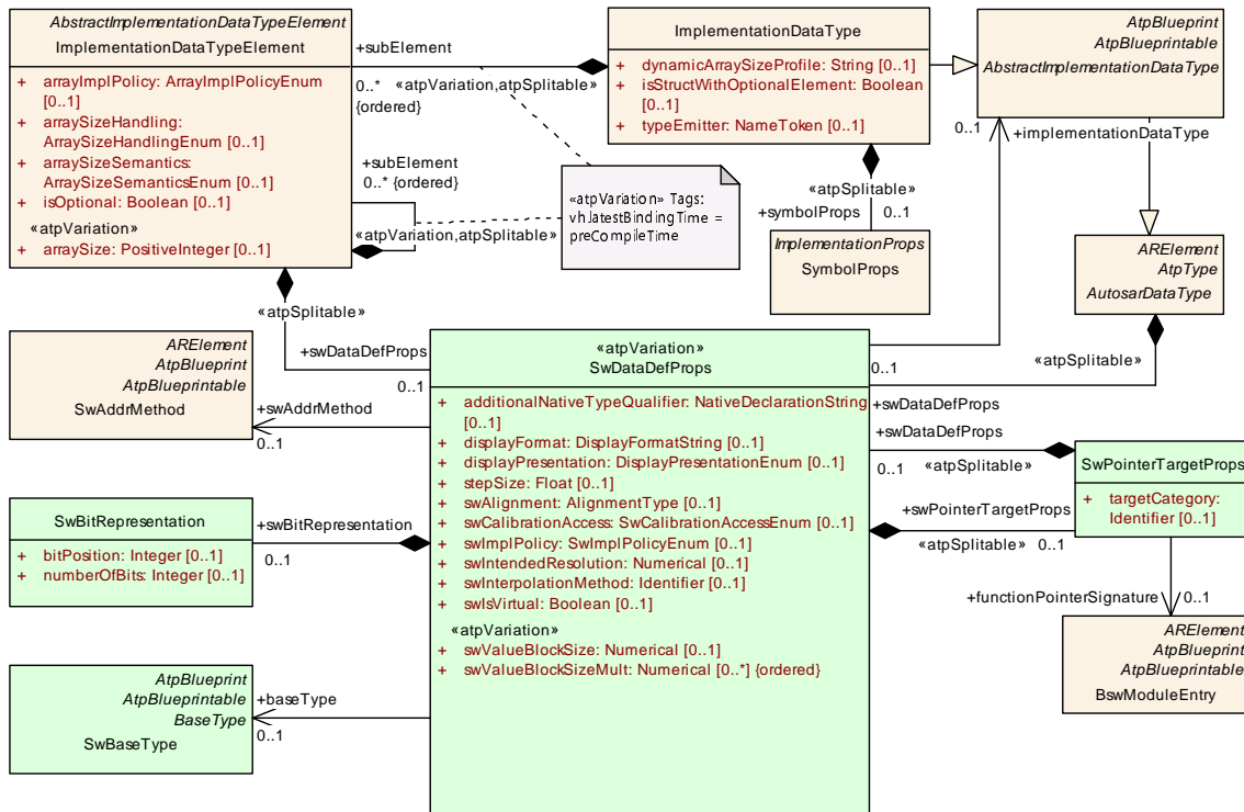
Figure 5.11: SwDataDefProps used in the context of ImplementationDataType
