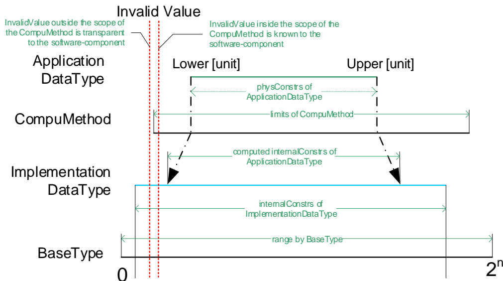
Figure 5.25: Value ranges and invalid values for linear and rational CompuMethod
