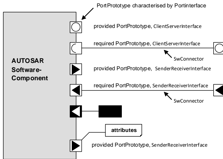
Figure 3.1: Graphical representation of software-components in AUTOSAR
