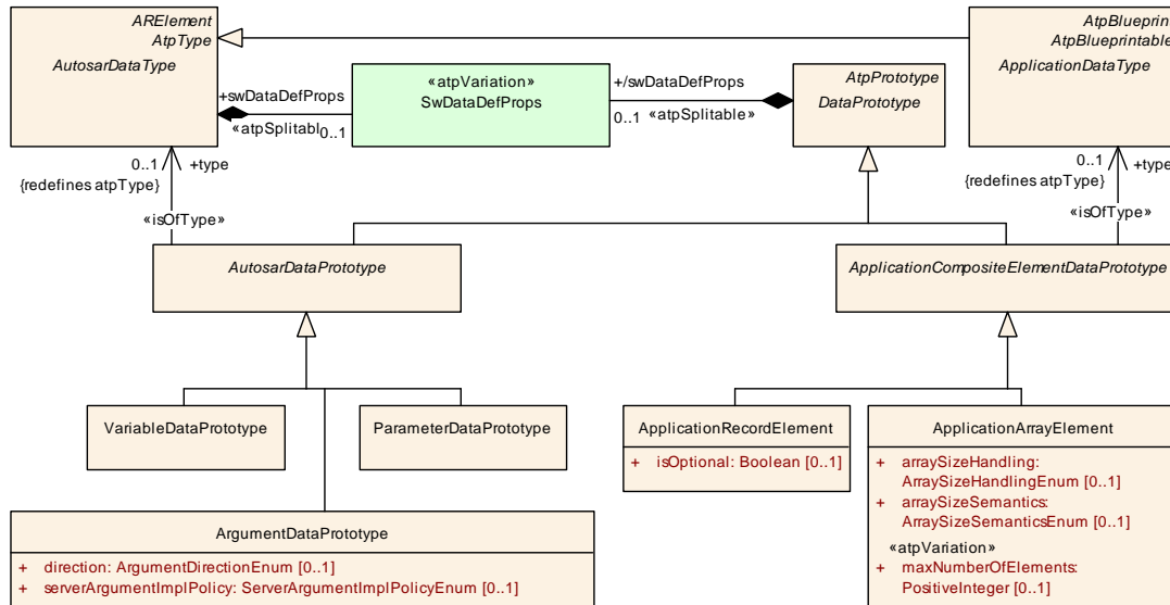
Figure 5.15: Data Prototypes Overview
