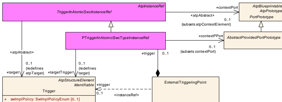
Figure D.7: Concrete modeling of references to Trigger in the context of a PPortPrototype
