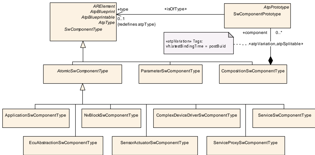
Figure 3.4: Overview of Component Types
