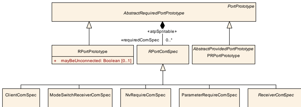
Figure 4.34: Overview of communication attributes of RPortPrototype
