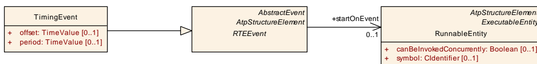
Figure 7.5: Periodic activation of RunnableEntities
