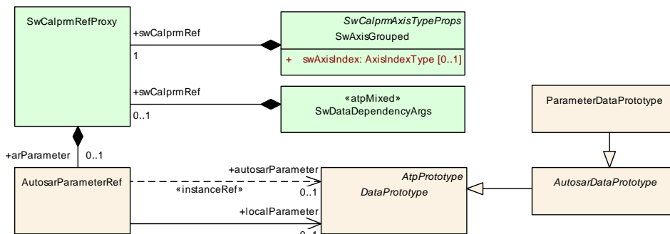
Figure 5.39: Applying Proxy Parameter Reference Mechanism
