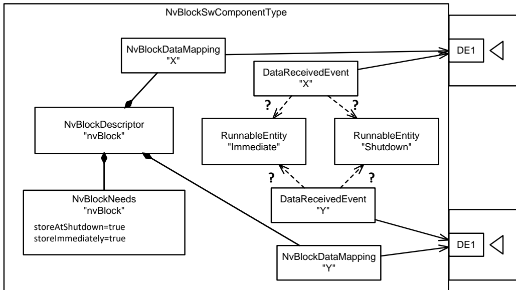
Figure 11.9: Existence of several event-based writing strategies for the same NvBlockDescriptor
