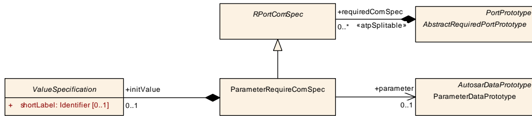
Figure 4.45: Communication attributes of ParameterDataPrototypes with respect to RPortPrototype
