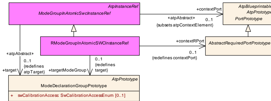
Figure D.11: Concrete modeling of references to ModeDeclarationGroupPrototype in the context of an RPortPrototype
