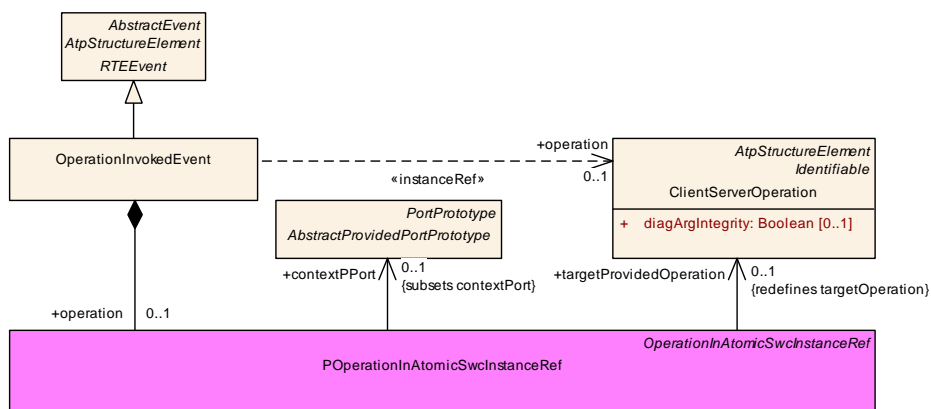
Figure D.30: Modeling of references to a ClientServerOperation used in the context of an RTEEvent
