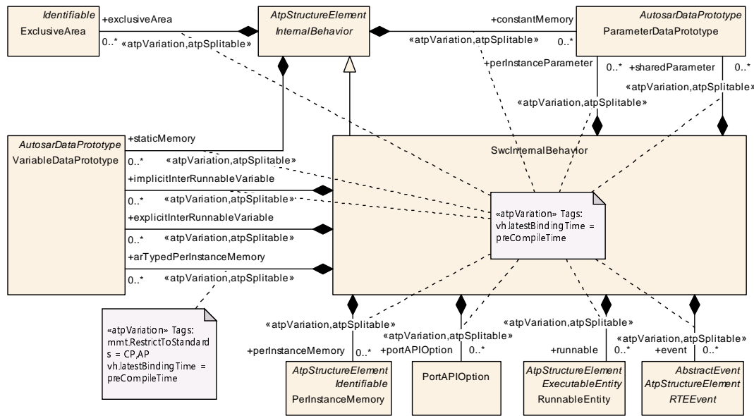
Figure 7.2: SwcInternalBehavior
