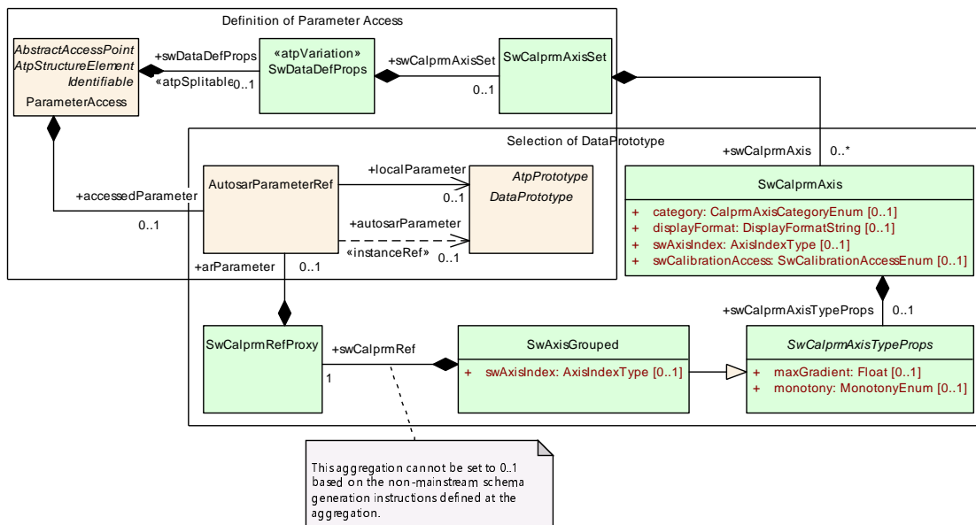
Figure 5.34: Usage of SwAxisGrouped in the context of a ParameterAccess
