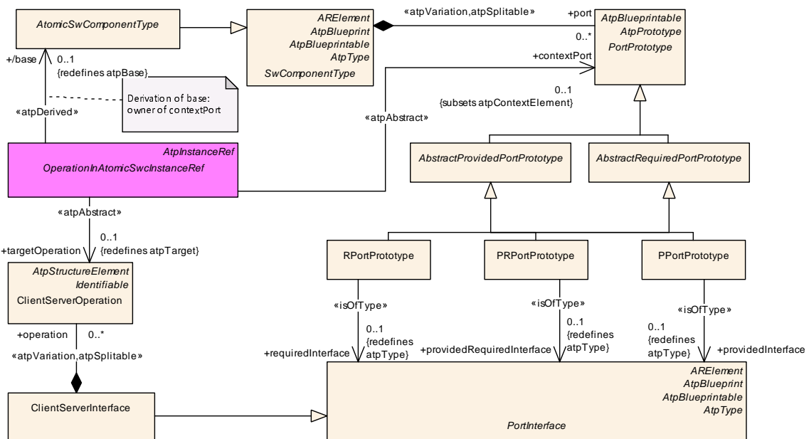
Figure D.8: Abstract modeling of references to ClientServerOperation in the context of a AtomicSwComponentType
