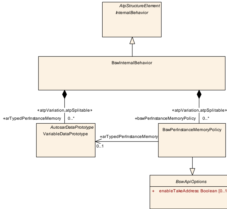
Figure 5.16: BSW Measurement Data
