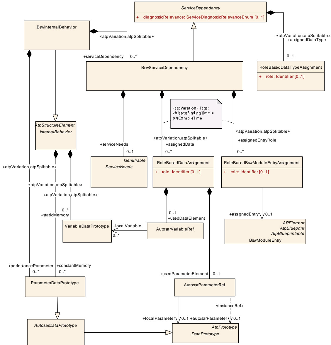
Figure 12.2: BswServiceDependency attached to a BswInternalBehavior
