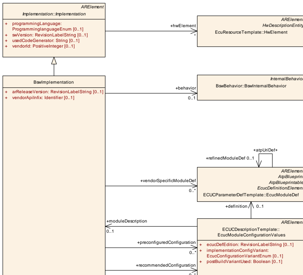
Figure 6.1: Overview of class BswImplementation
