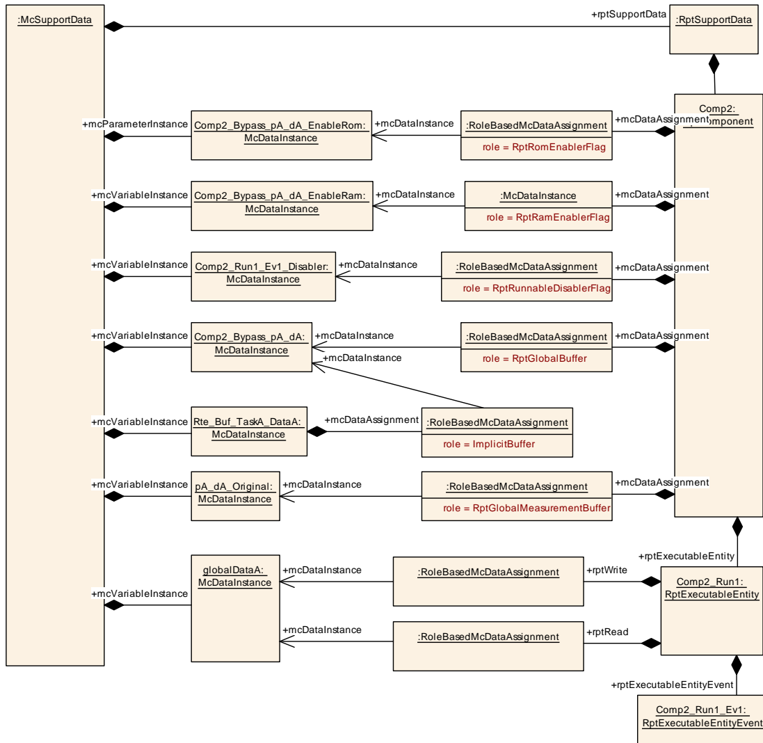
Figure 9.13: Example about RptComponent usage
