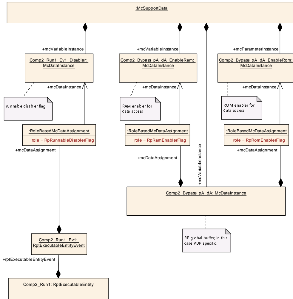
Figure 9.11: Example about Level3 enabler
