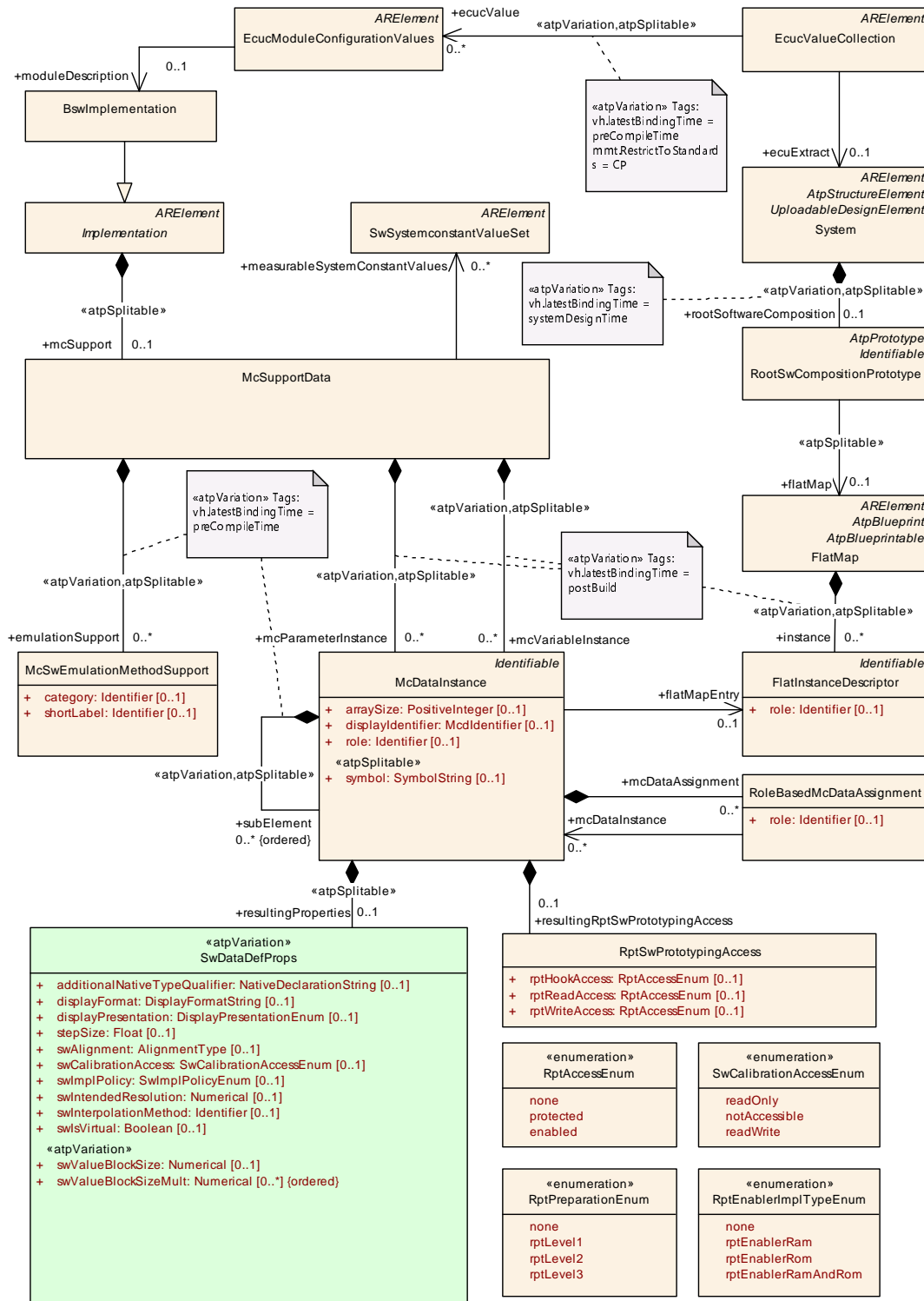
Figure 9.1: Calibration Support Data attached to Implementation
