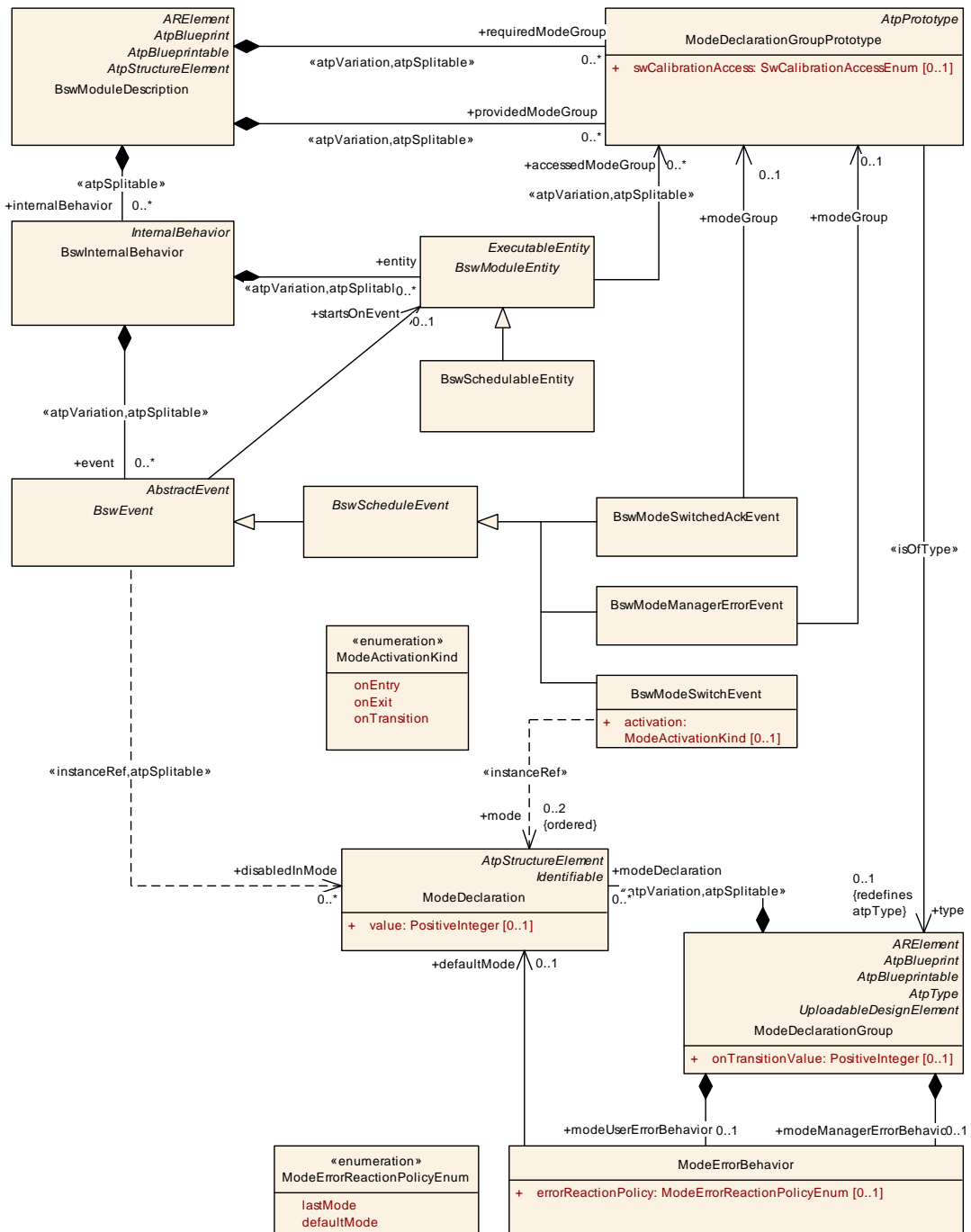
Figure 5.9: Details on BSW Events related to Mode Switches
