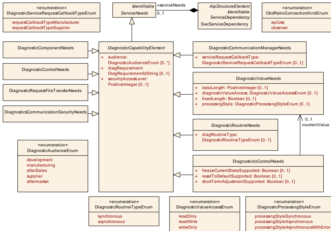
Figure 12.4: Class ServiceNeeds from CommonStructure and derived classes for diagnosis use cases
