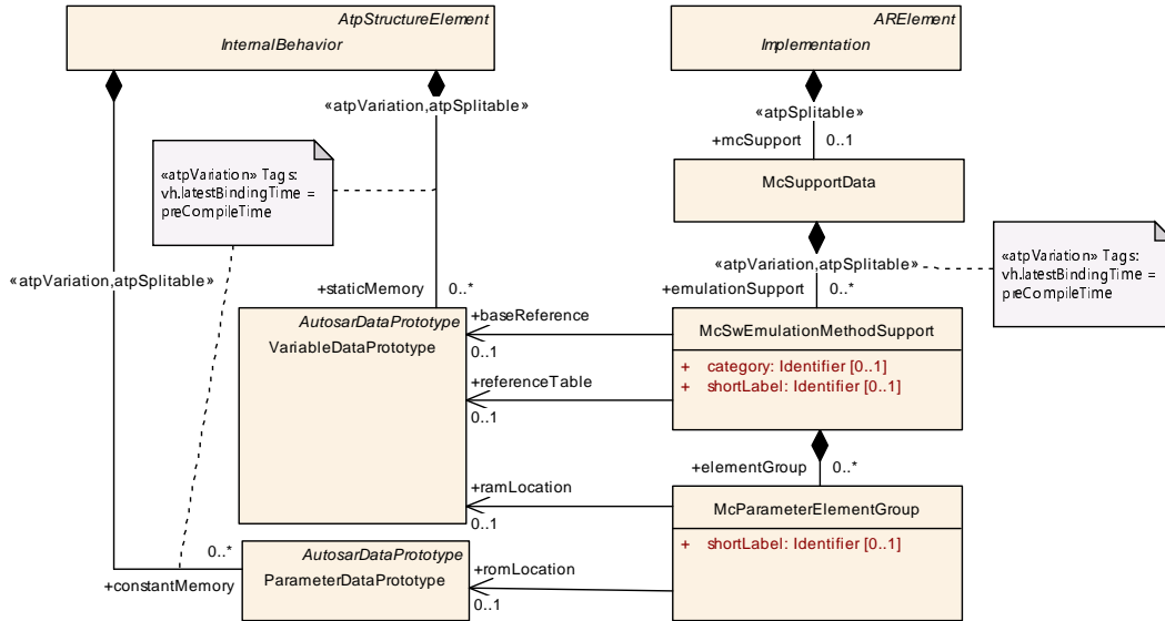
Figure 9.3: Describing the Software Emulation Method for Calibration Data
