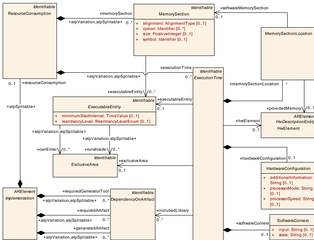
Figure 8.5: Detailed relations of an ExecutionTime description
