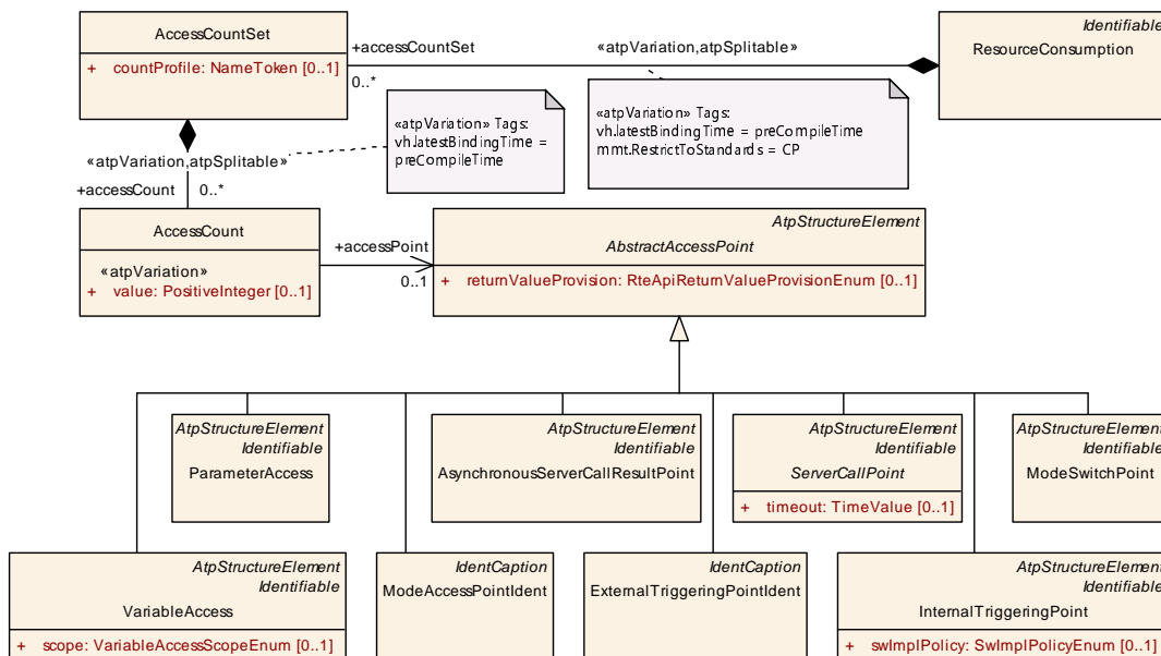
Figure 4.7: Overview AccessCountSet
