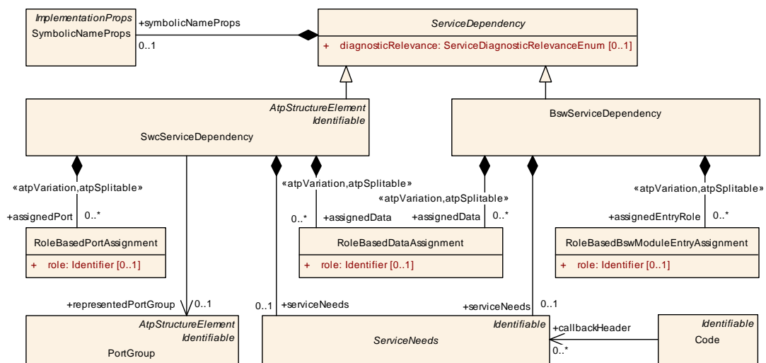
Figure 12.1: Concept of ServiceDependency for BSW and SWC
