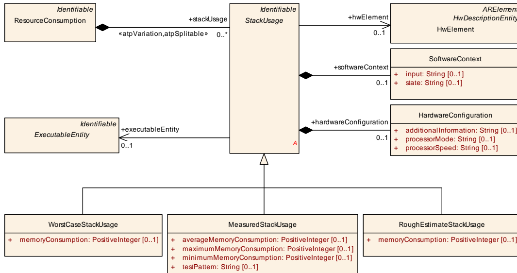
Figure 8.3: Stack Memory Consumption
