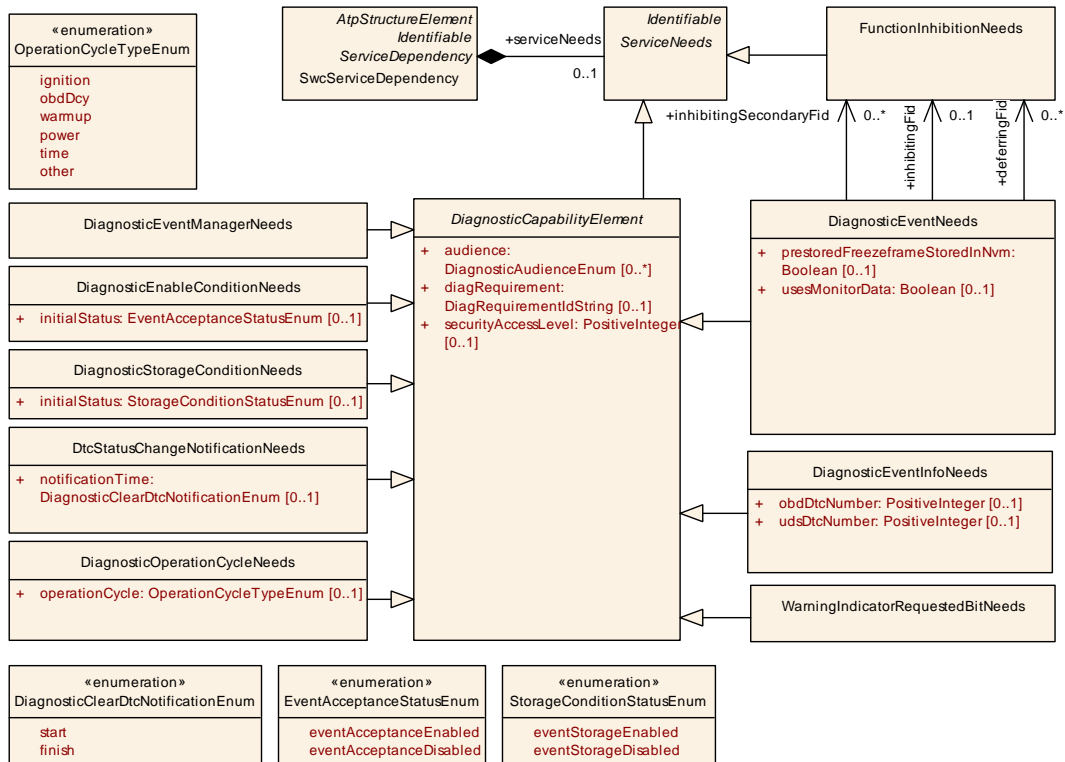
Figure 12.5: Class ServiceNeeds from CommonStructure and derived classes for diagnosis use cases
