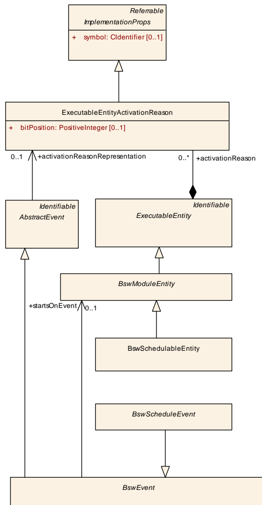
Figure 5.12: BswModuleEntity and activation reason
