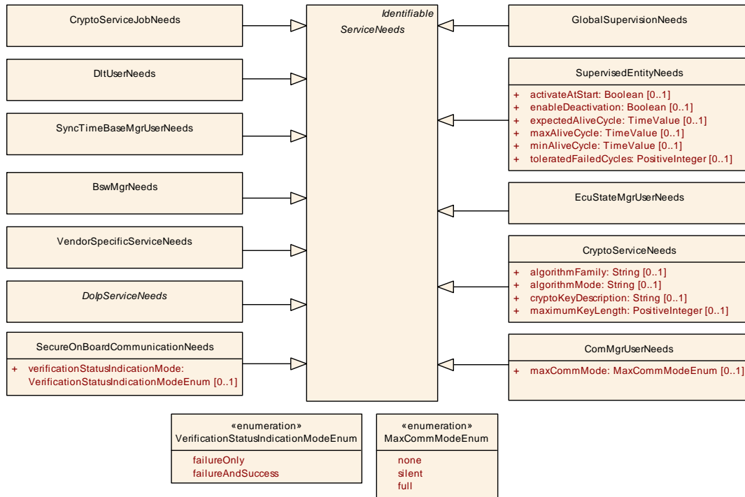
Figure 12.3: Class ServiceNeeds from CommonStructure and some derived classes
