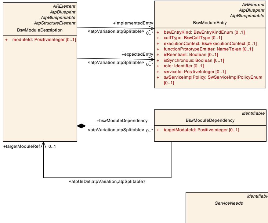
Figure 4.3: Details of class BswModuleDependency
