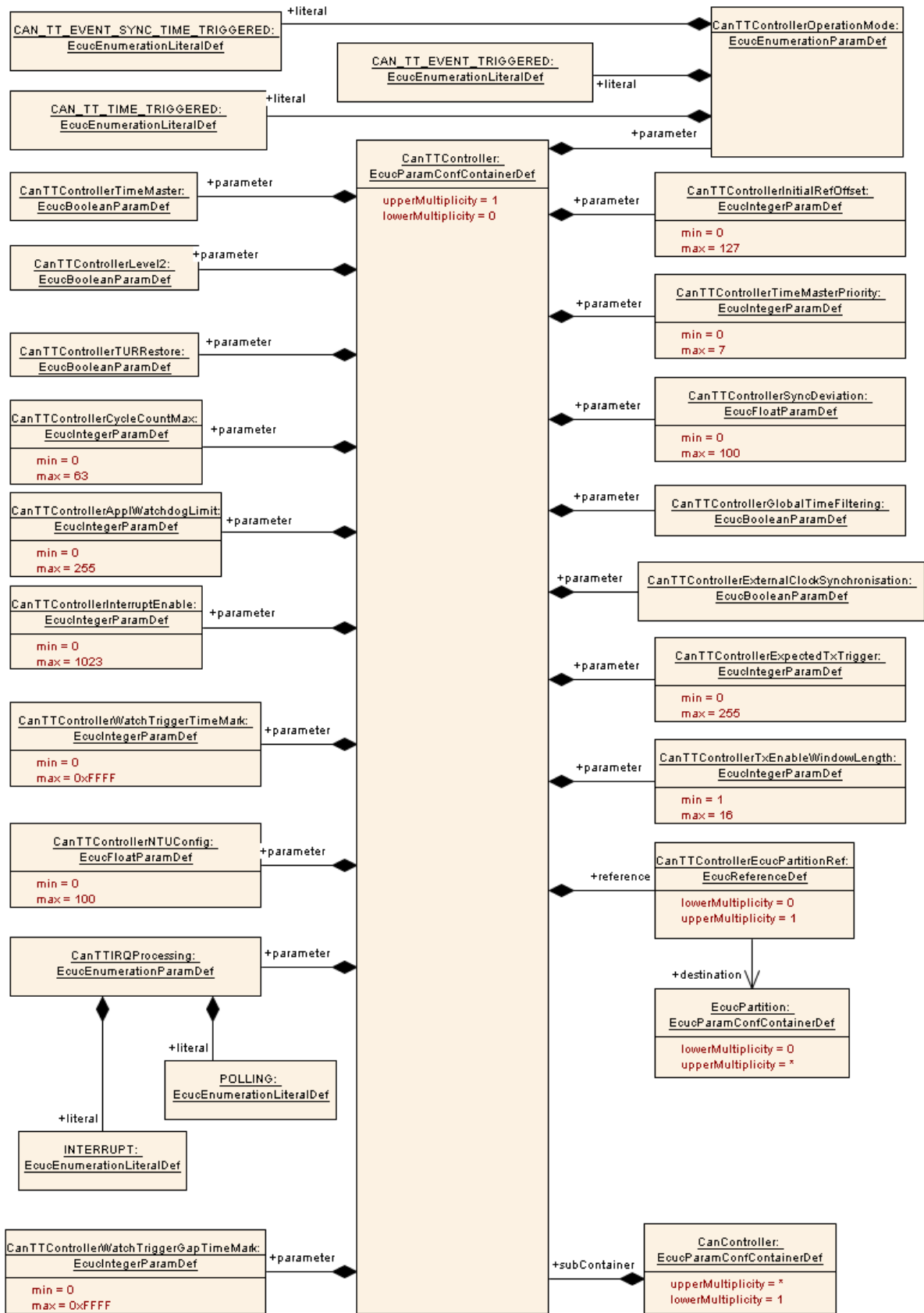
Figure 10.2: CAN Driver Time Triggered Controller Configuration
