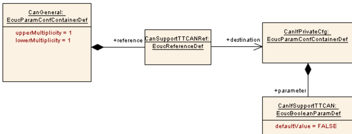
Figure 10.1: CAN Driver Time Triggered General Configuration
