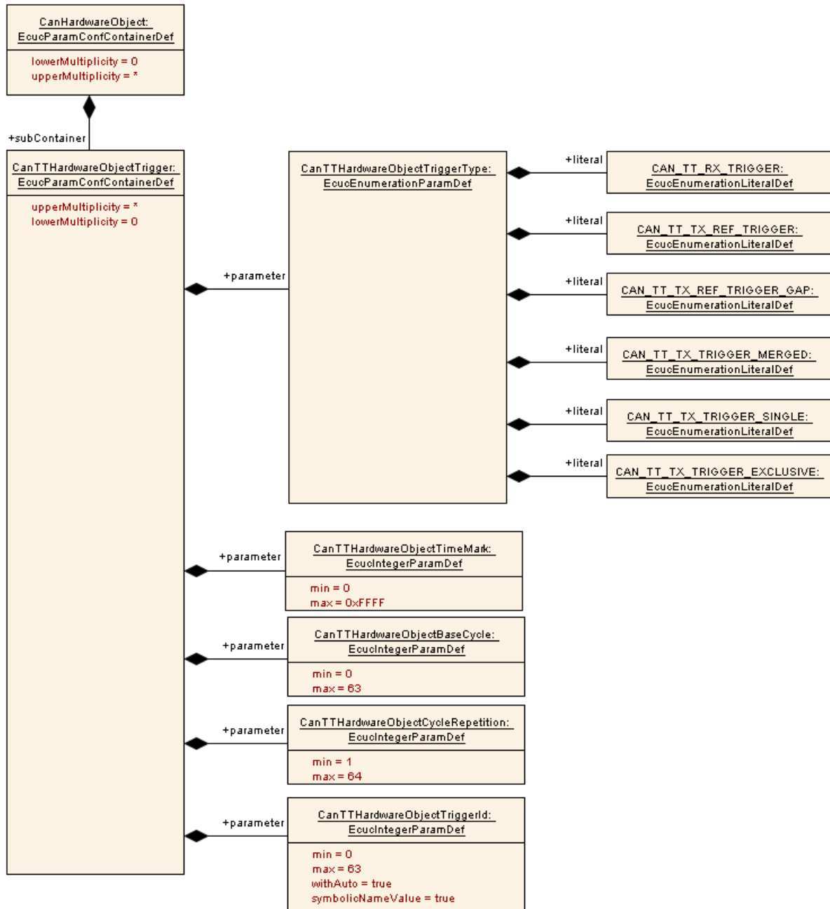
Figure 10.3: CAN Driver Time Triggered Hardware Object Configuration
