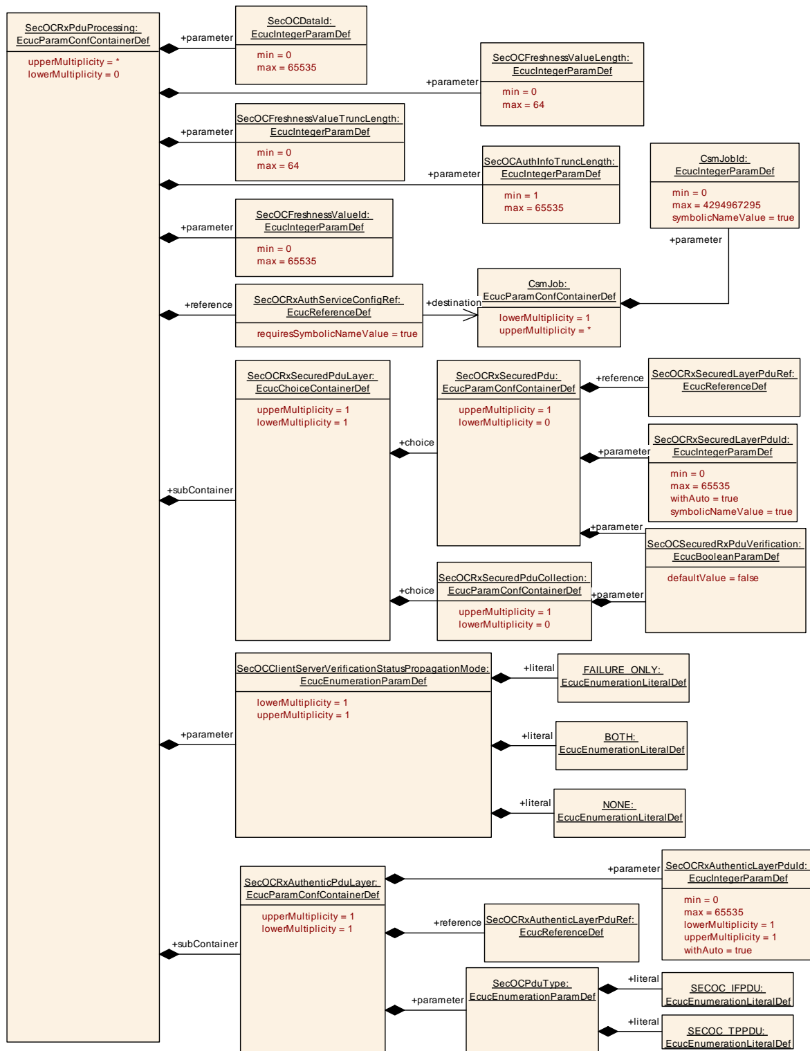
Figure 18: The AUTOSAR SecOC Rx Pdu Configuration Part 1
