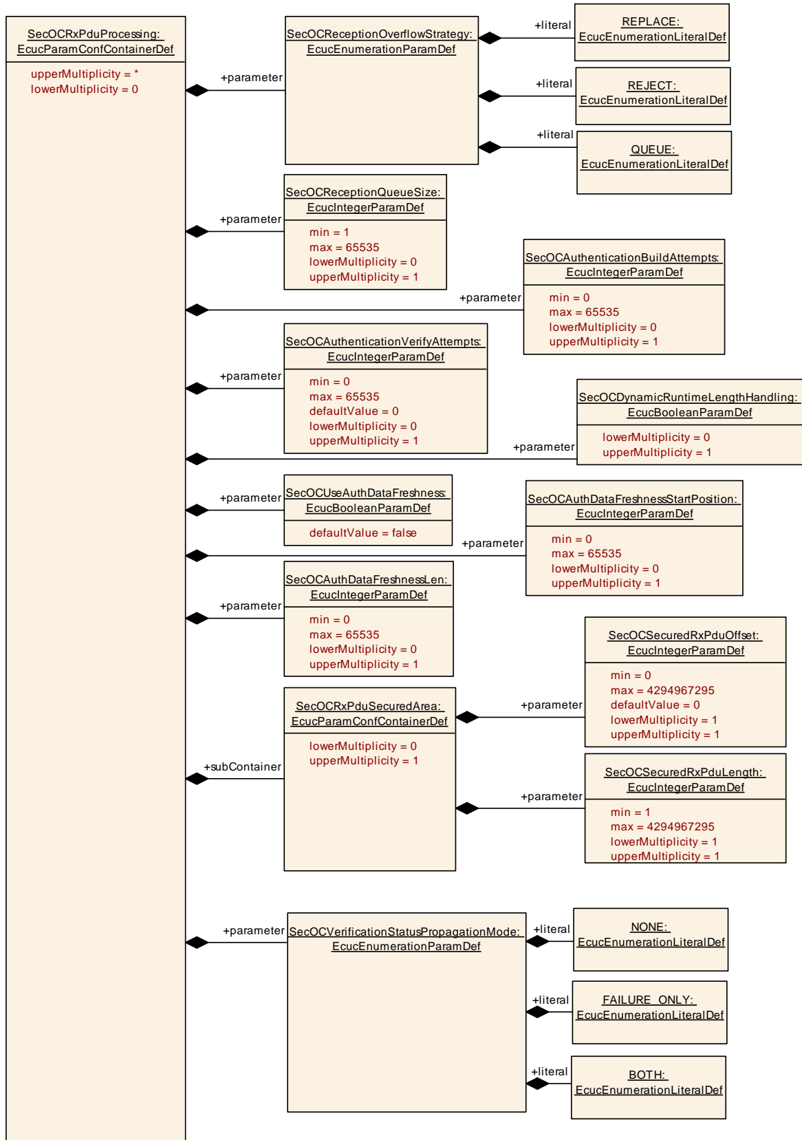
Figure 19: The AUTOSAR SecOC Rx Pdu Configuration Part 2
