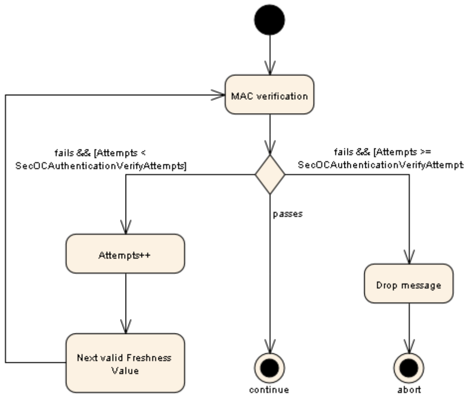
Figure 6: Verification of MAC
