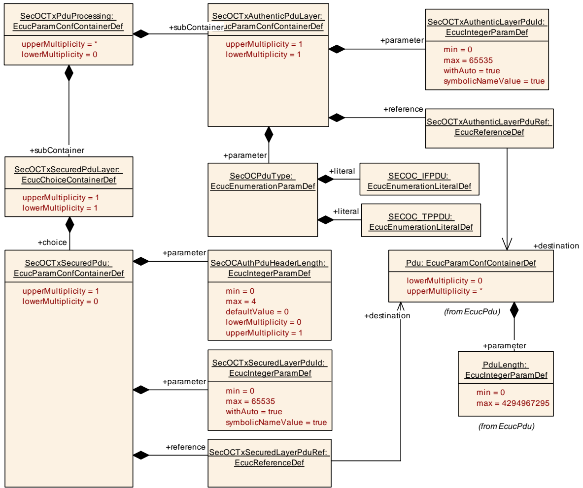
Figure 20: The AUTOSAR SecOC Tx Pdu Configuration Part 1
