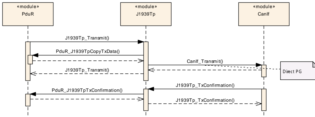
Figure 9.4: Transmission of Direct PG
