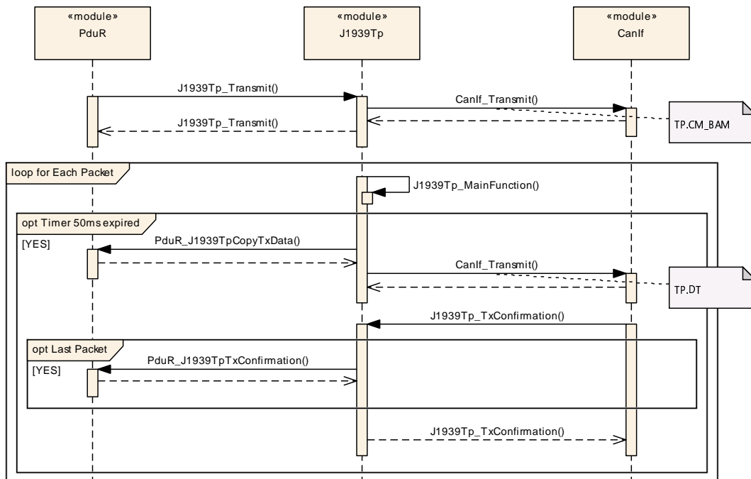
Figure 9.5: Transmission via BAM
