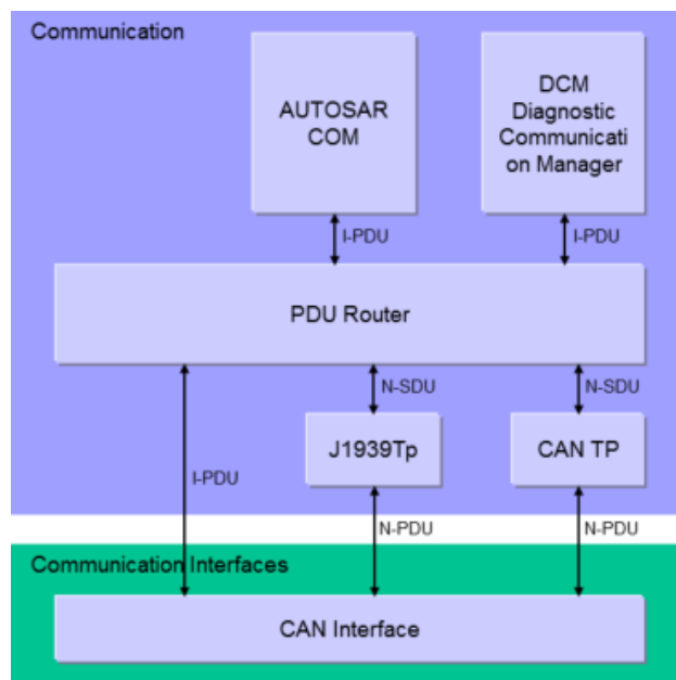
Figure 1.1: AUTOSAR Communication Stack
