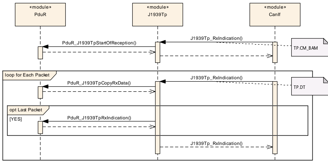
Figure 9.2: Reception via BAM
