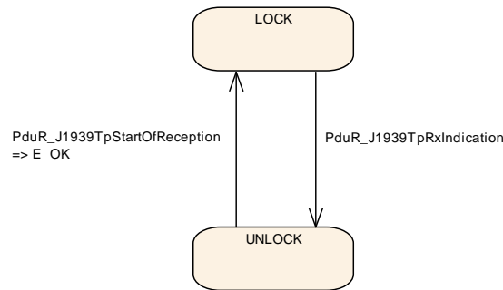
Figure 7.6: Rx Buffer locking
