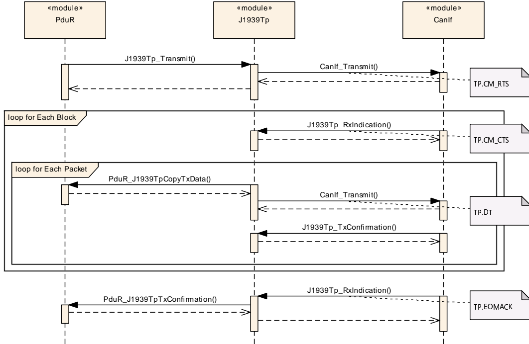
Figure 9.6: Transmission via CMTD
