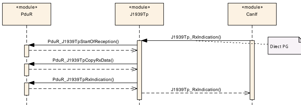
Figure 9.1: Reception of Direct PG
