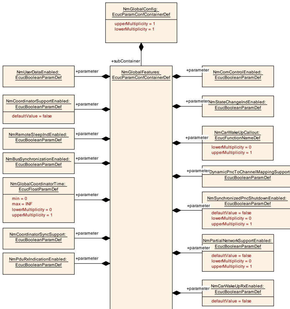
Figure 10.4: NmGlobalFeatures overview
