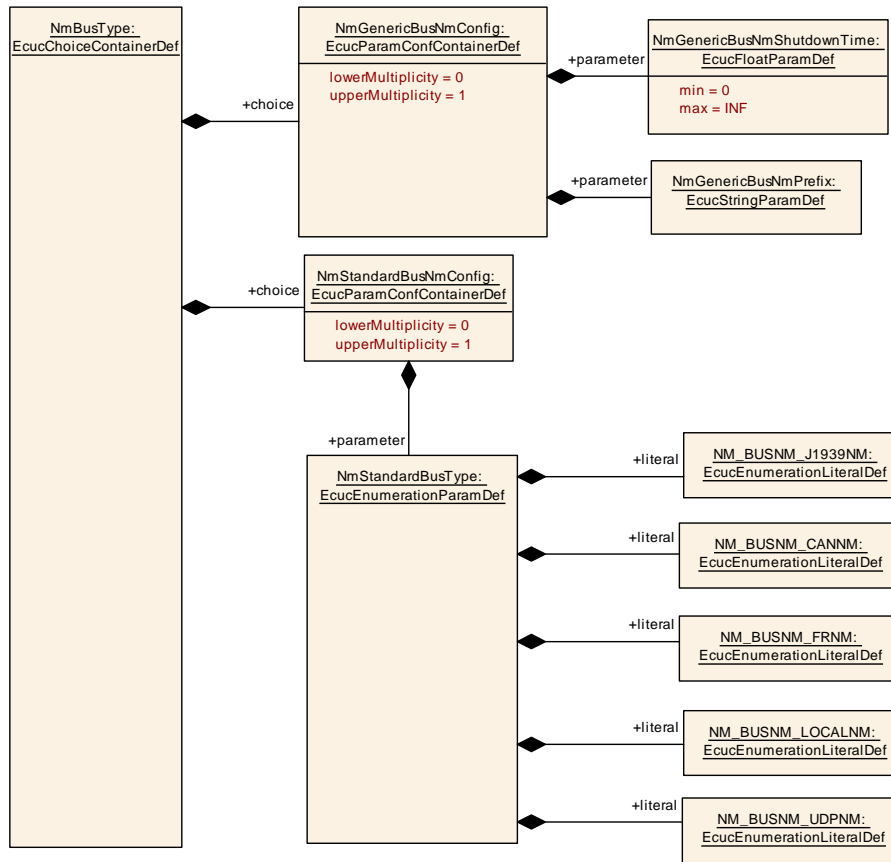
Figure 10.6: NmBusType overview
