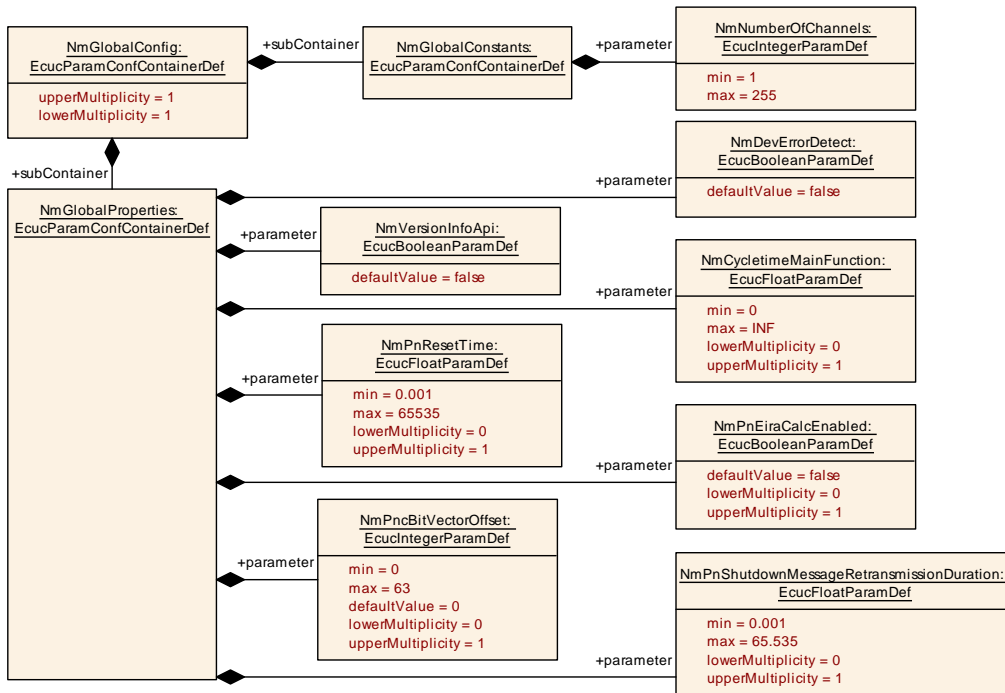
Figure 10.3: NmGlobalConfig overview
