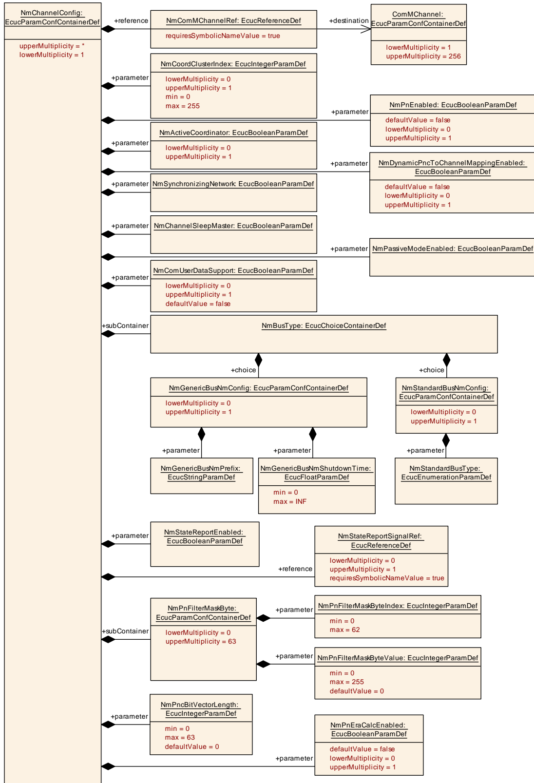
Figure 10.5: NmChannelConfig overview
