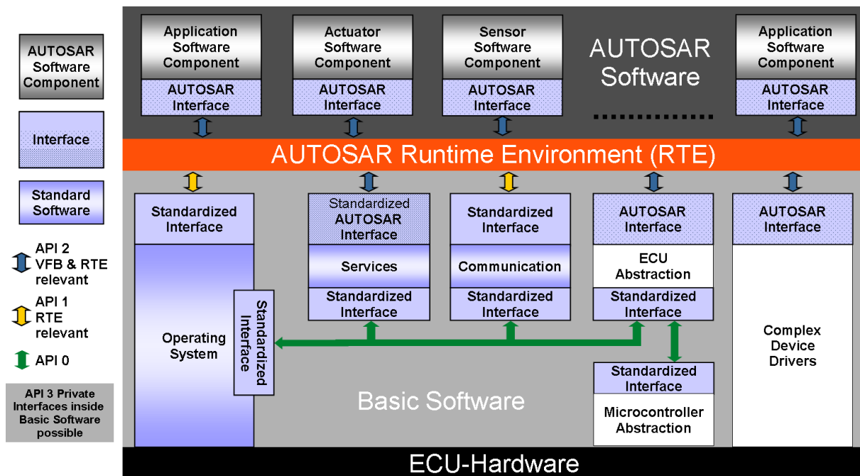
Figure 7-1: AUTOSAR architecture
