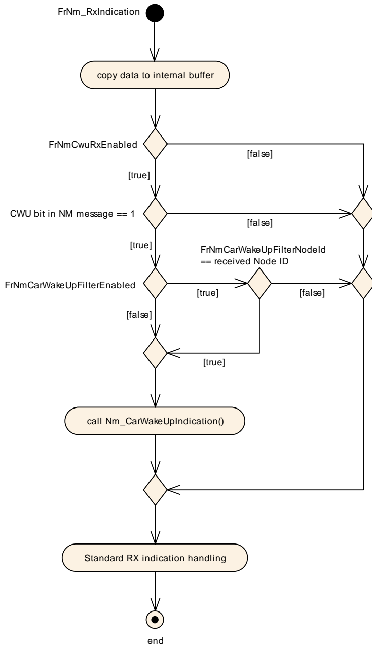
Figure 7.5: CarWakeUp indication handling
