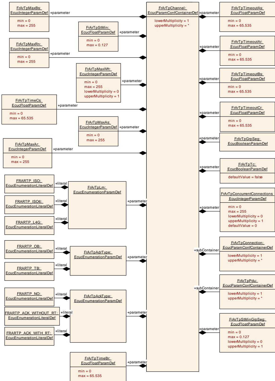
Figure 23: FrArTpChannel configuration
