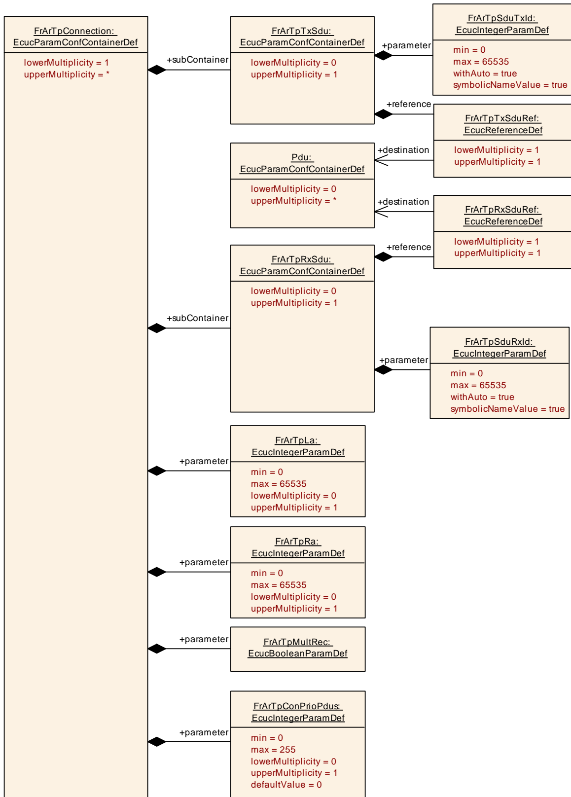
Figure 24: FrArTpConnection configuration
