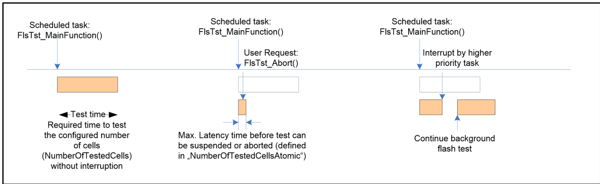
Figure 7.2: Background Test: Test Process
