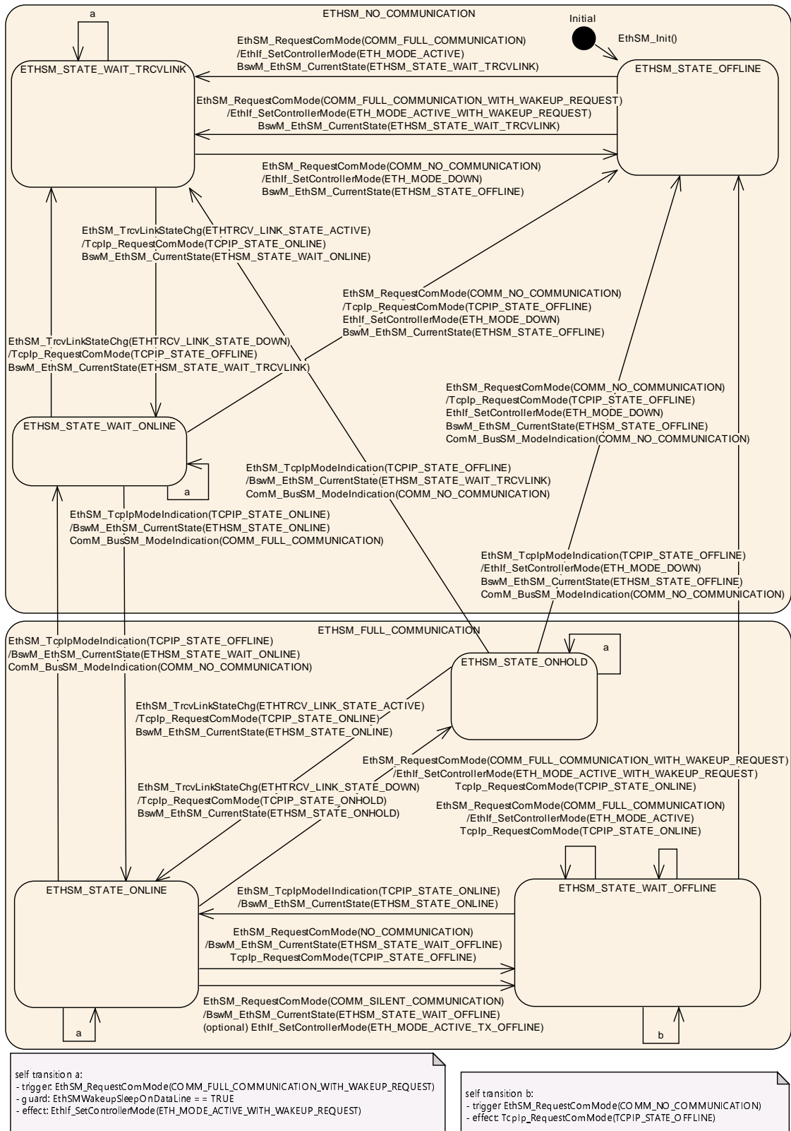
Figure 7.1: Network mode state machine of the EthSM
