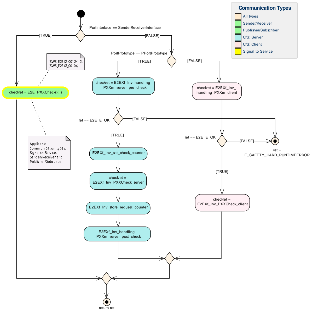
Figure 7.18: E2EXf_Inv_handling_main_check
