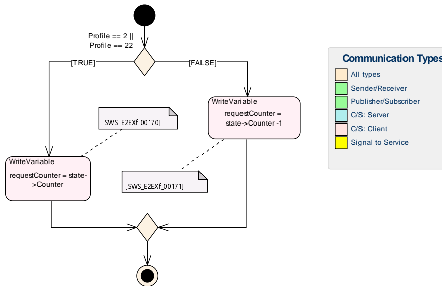
Figure 7.9: E2EXf_store_request_counter
