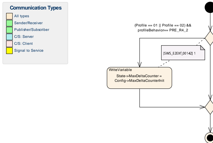
Figure 7.17: E2EXf_Inv_handling_P01_P02_forceConstantMxDeltaCounter
