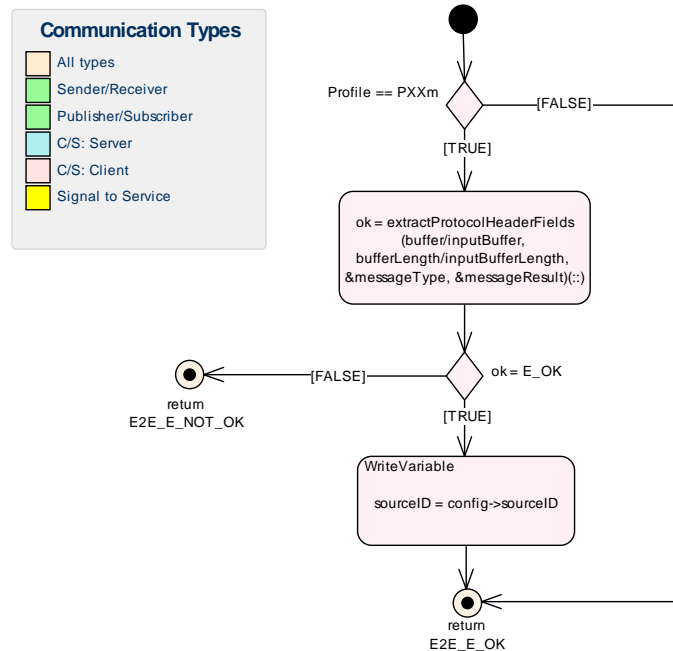
Figure 7.10: E2EXf_handling_PXXm - client
