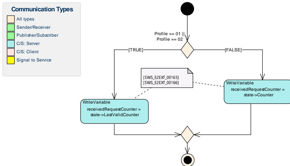
Figure 7.25: E2EXf_Inv_store_request_counter
