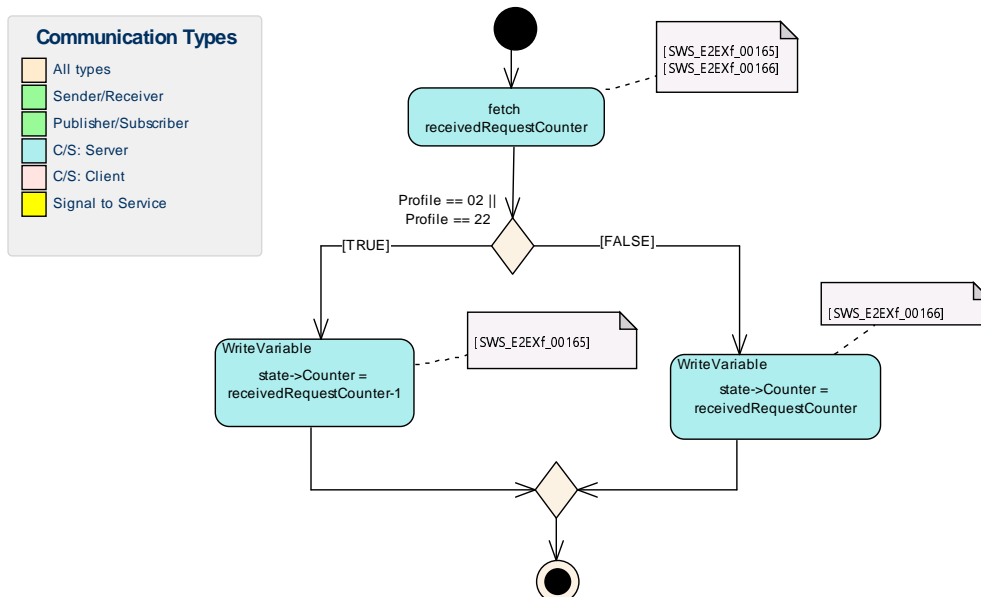
Figure 7.12: E2EXf_set_response_counter
