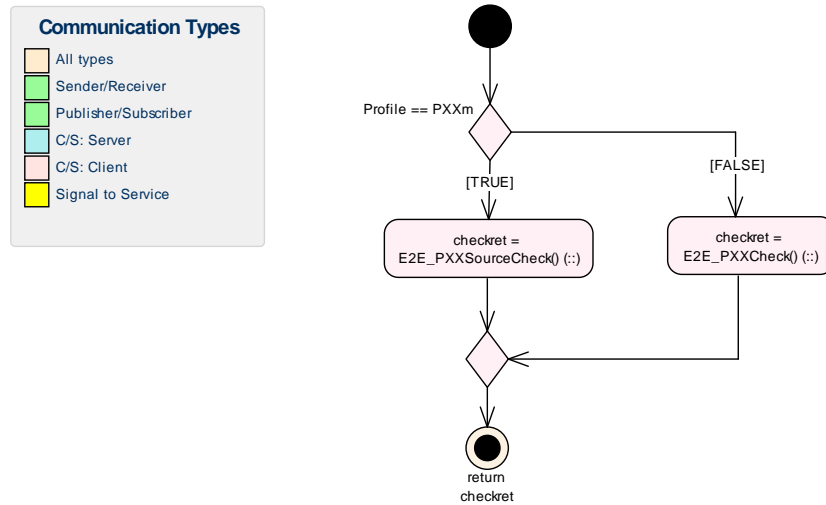
Figure 7.21: E2EXf_Inv_handling_PXXCheck - client(check)
