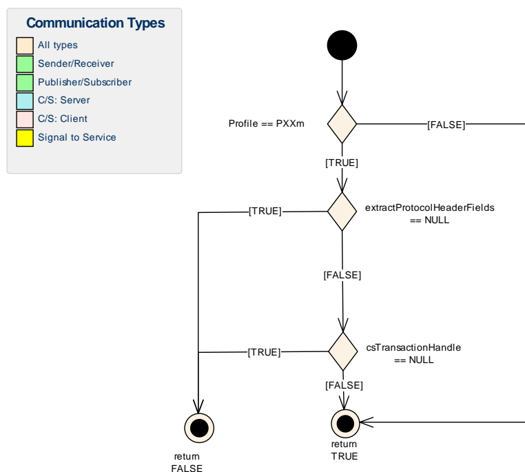
Figure 7.15: E2EXf_Inv_input_checks_PXXm
