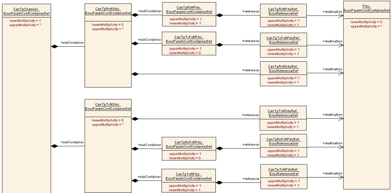
Figure 10.4: CanTpChannel configuration overview
