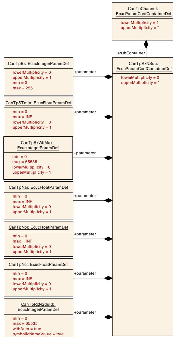
Figure 10.6: CanTpRxNSdu configuration overview (part 2)
