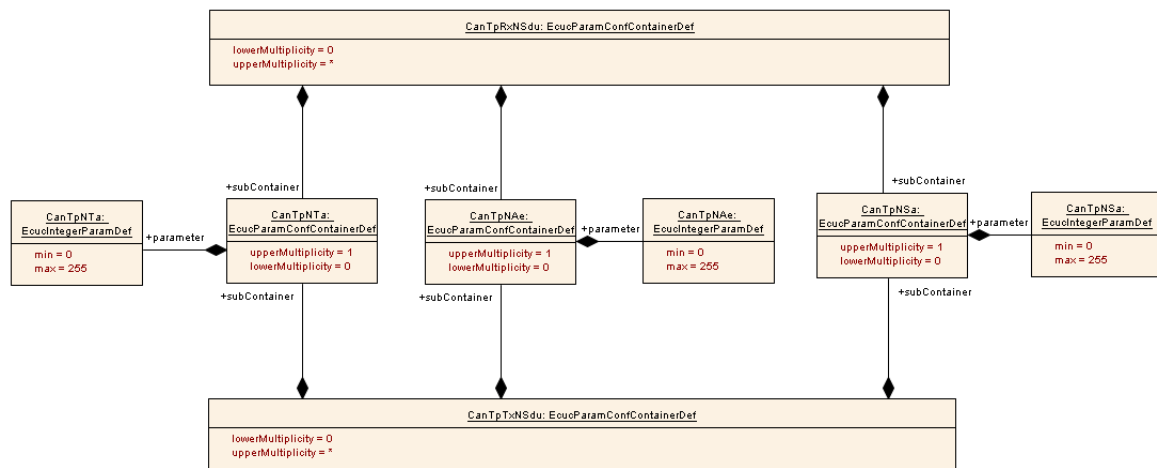
Figure 10.8: CanTpNTa, CanTpNSa and CanTpNAe configuration overview
