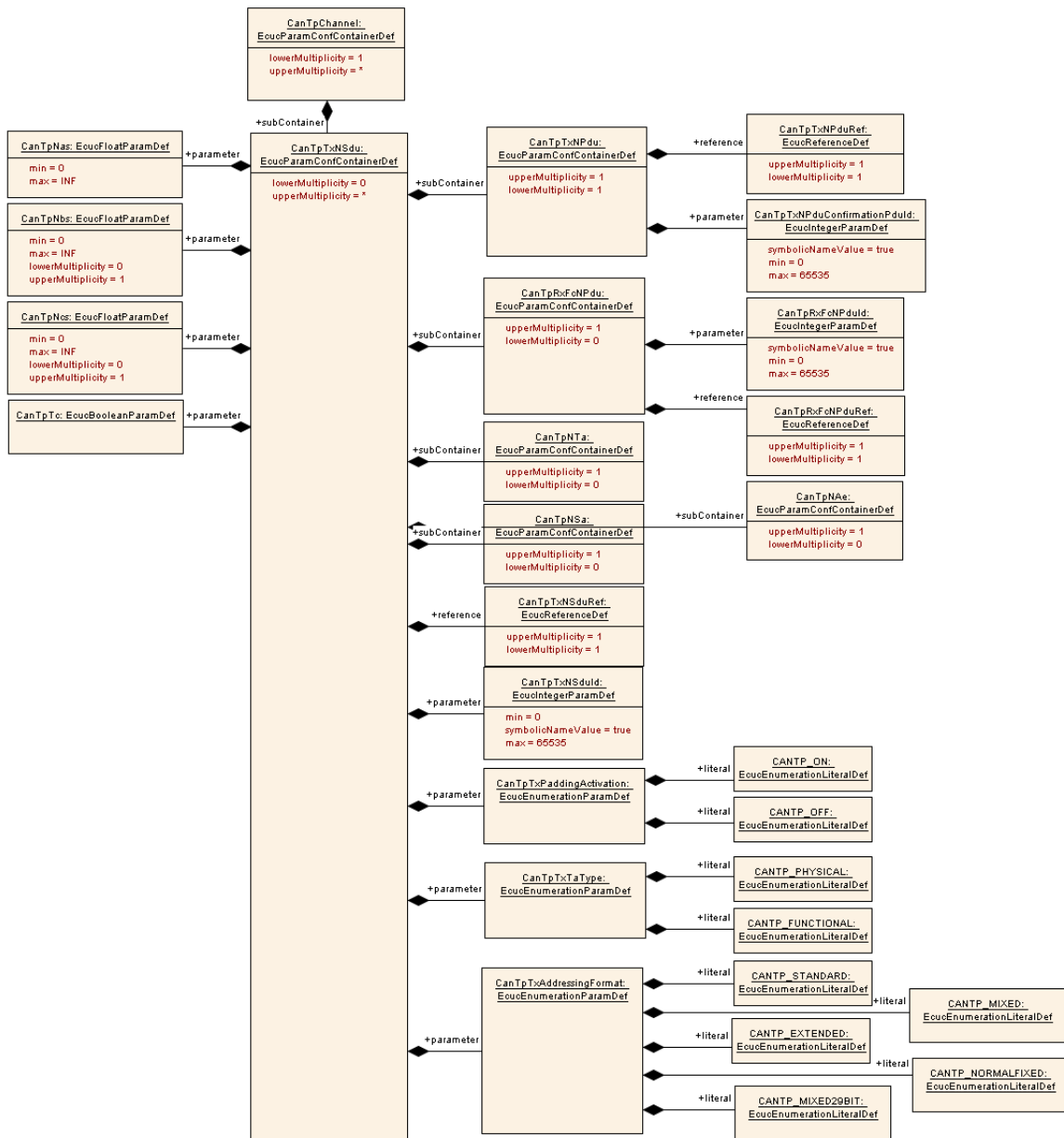
Figure 10.7: CanTpTxNSdu configuration overview
