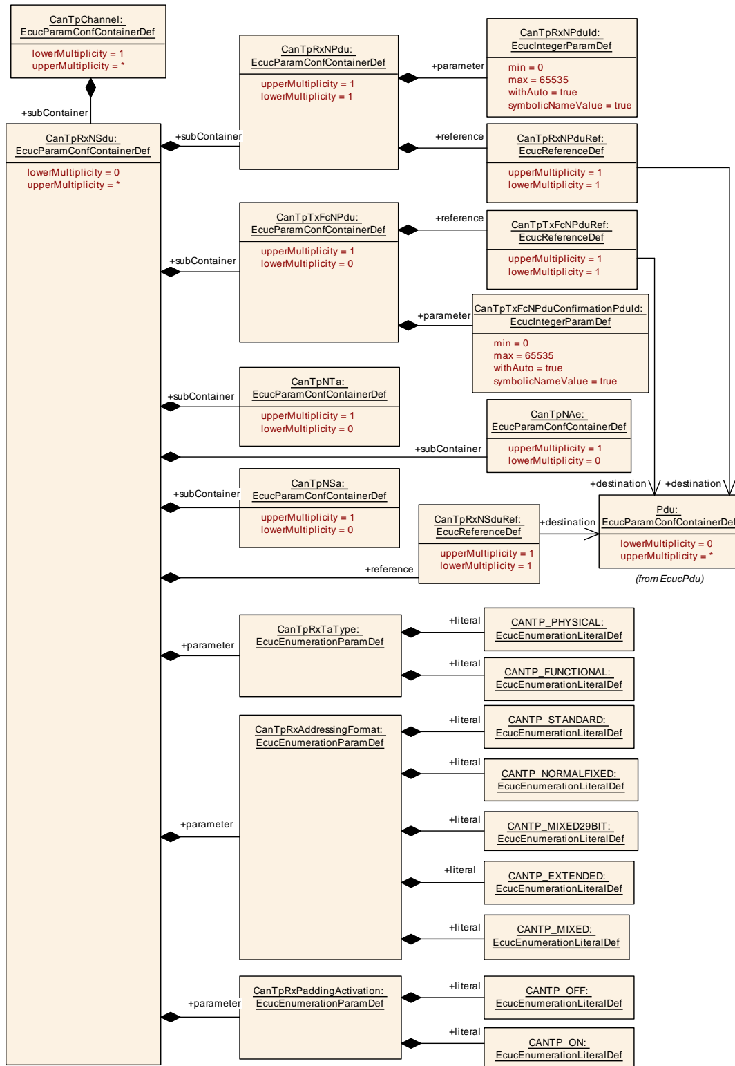
Figure 10.5: CanTpRxNSdu configuration overview (part 1)
