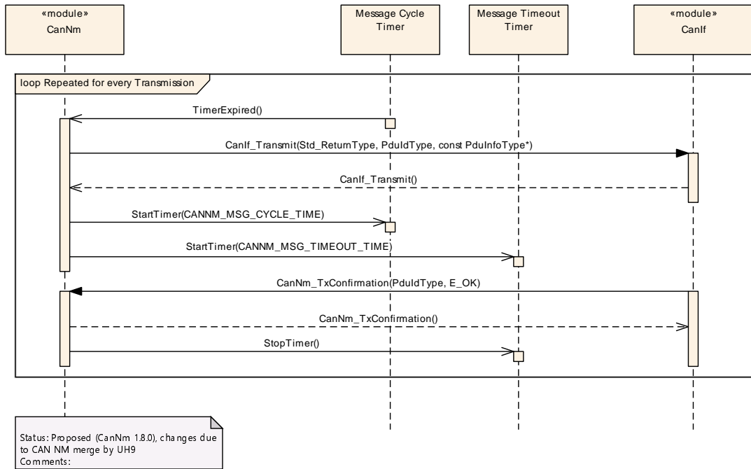
Figure 9.1: CanNm Transmission
