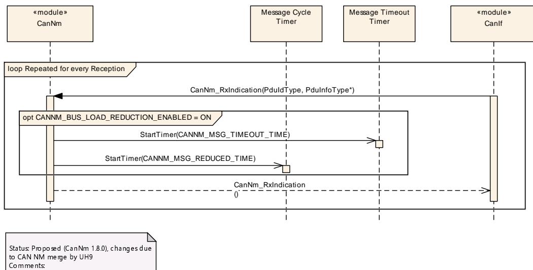
Figure 9.2: CanNm Reception
