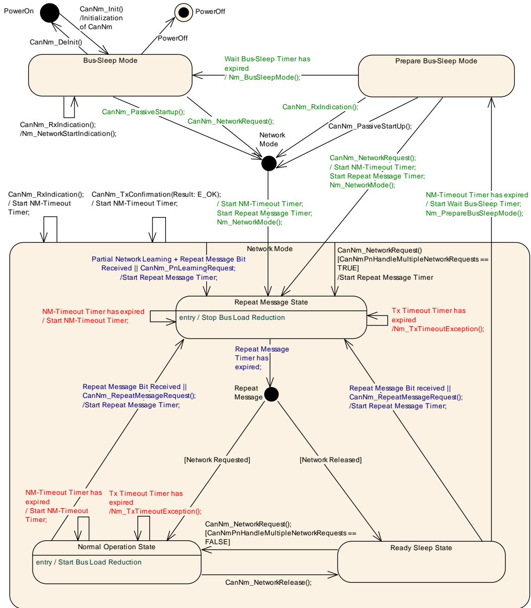
Figure 7.1: CanNm Algorithm
