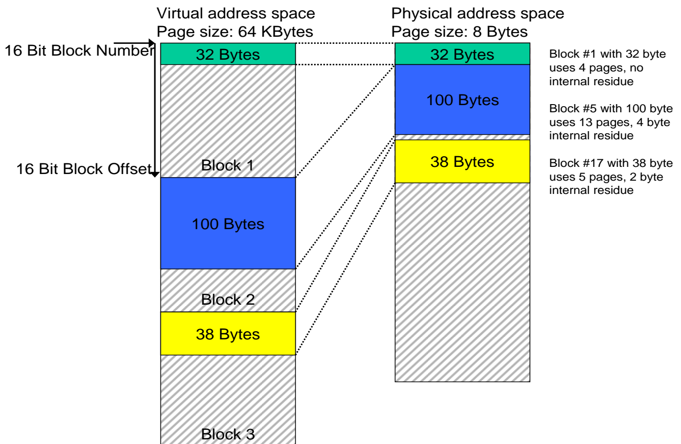
Note: Sizes not shown to scale Figure 6.2: Virtual vs. physical address space
