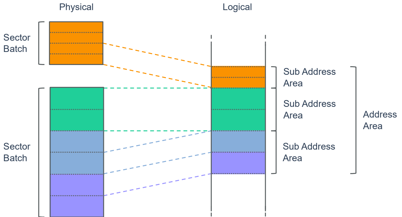
Figure 6.1: Overview of Address Translation/Mapping
