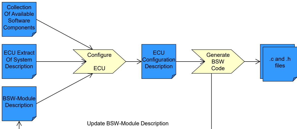
Figure 1.1: Overview AUTOSAR Methodology [1]
