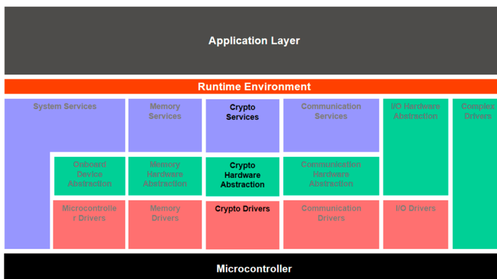
Figure 4.1: AUTOSAR layered view of the crypto stack [1]
