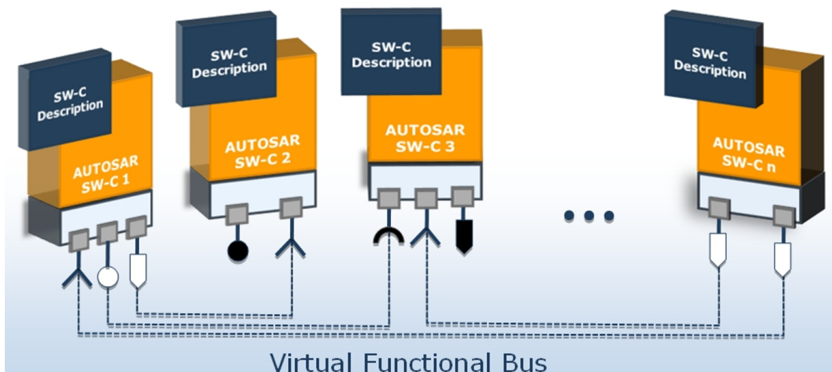
Figure 2.2: Software Components
