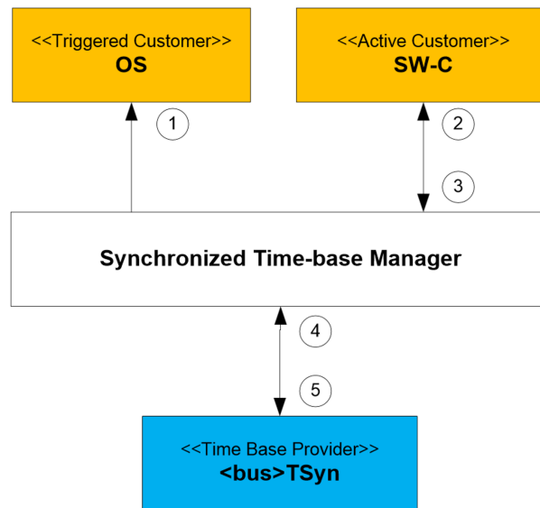
Figure 3.2: Synchronized Time-base Manager as broker
