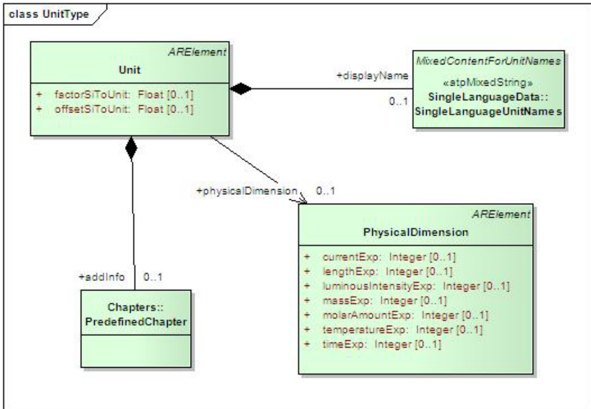
Figure 4.26: Units
