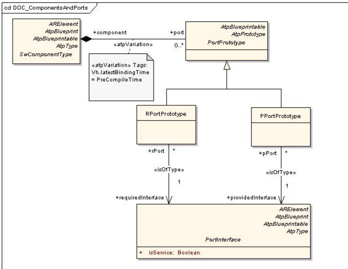
Figure 4.10: PortPrototypes
