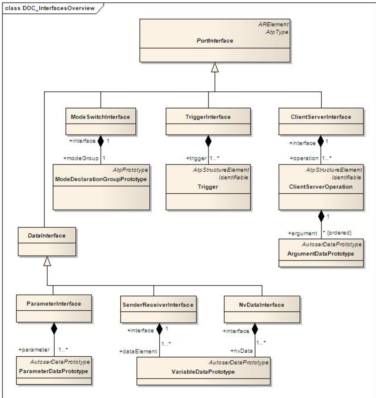
Figure 4.12: Interfaces Overview
