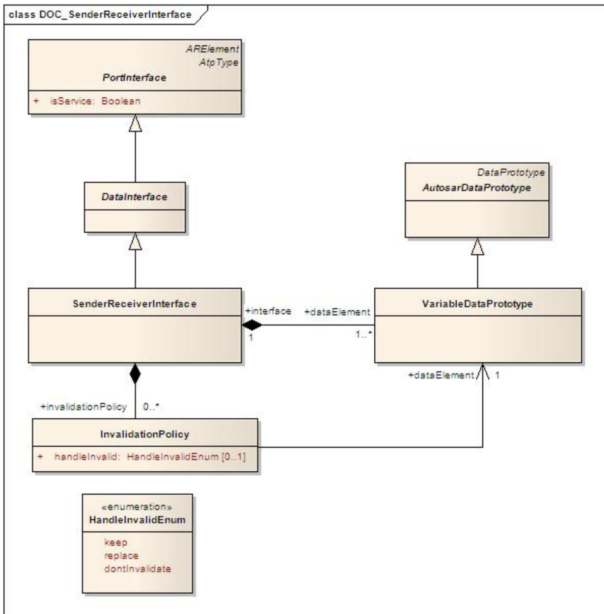
Figure 4.13: SenderReceiverInterface
