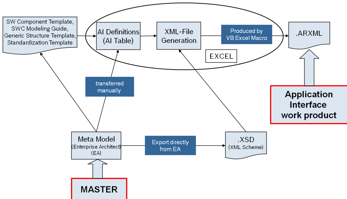
Figure 2.1: The AI Table Process
