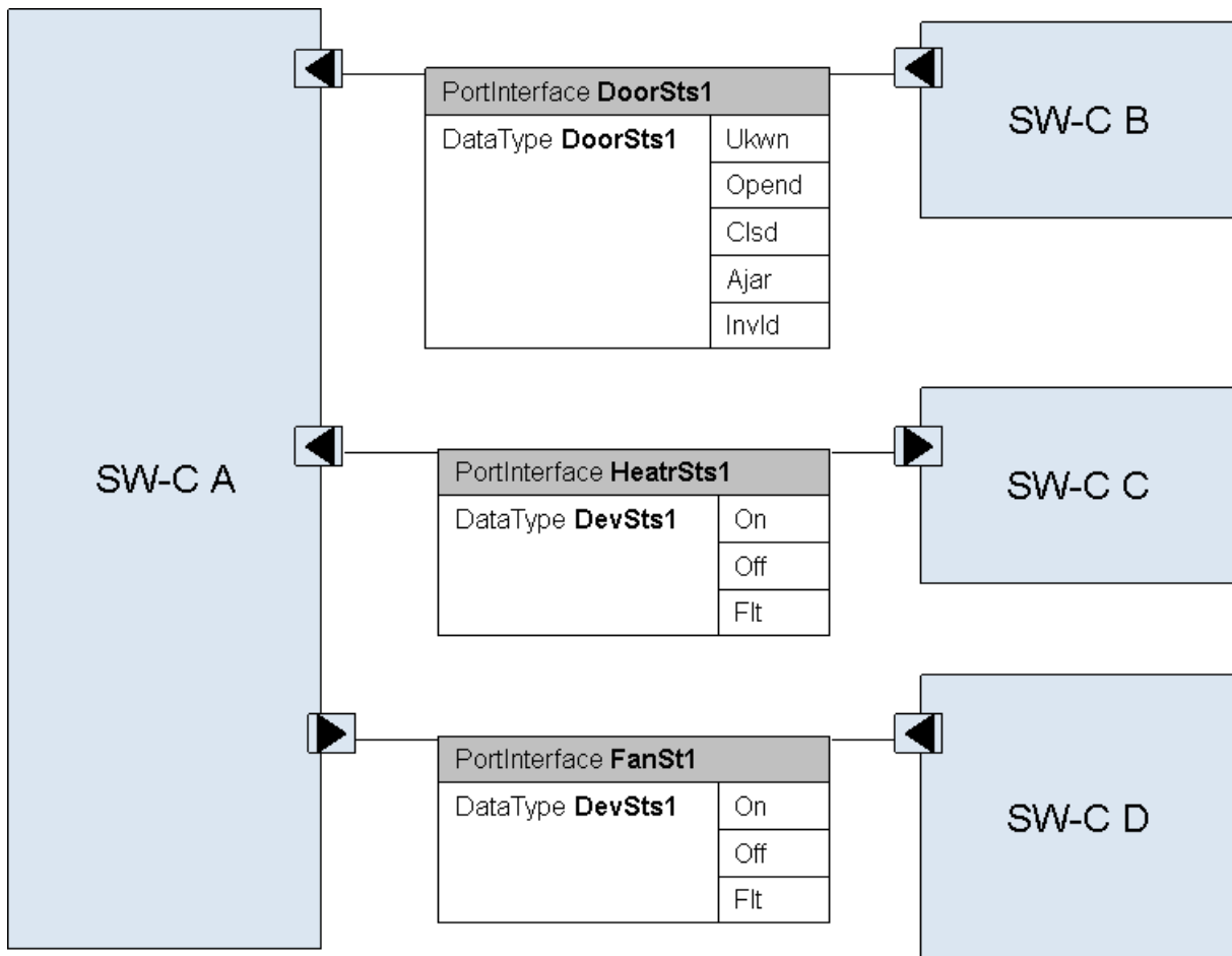
Figure 8.12: Reusability of DataTypes
