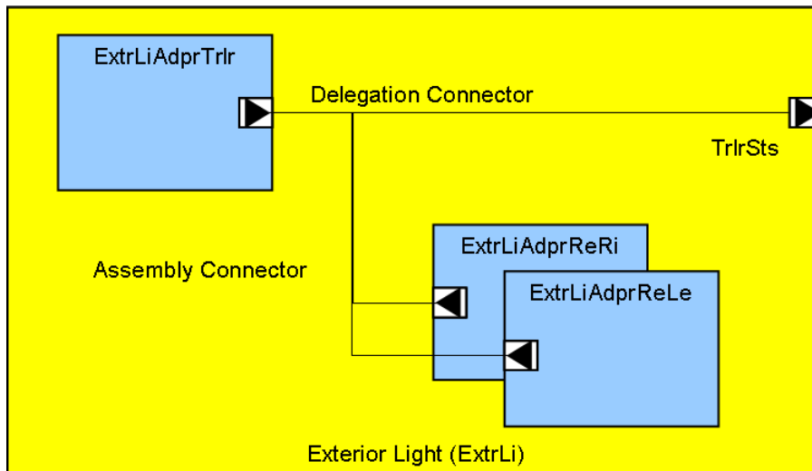
Figure 4.8: : Exterior Light Decomposition example
