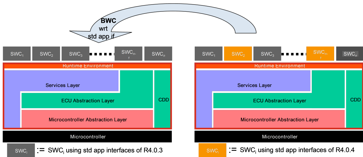
Figure 5.2: Example representation of BWC w.r.t. Application Interfaces
