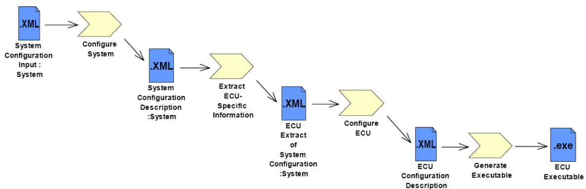
Figure 3.1: Overview AUTOSAR Methodology
