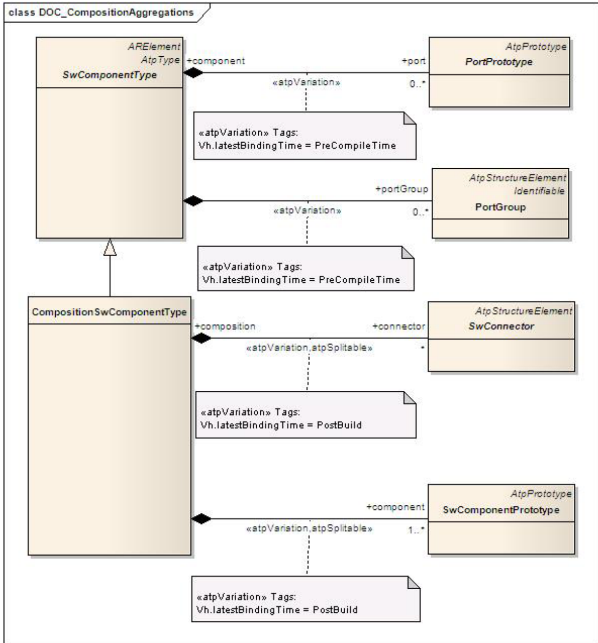
Figure 4.6: Composition - Aggregations
