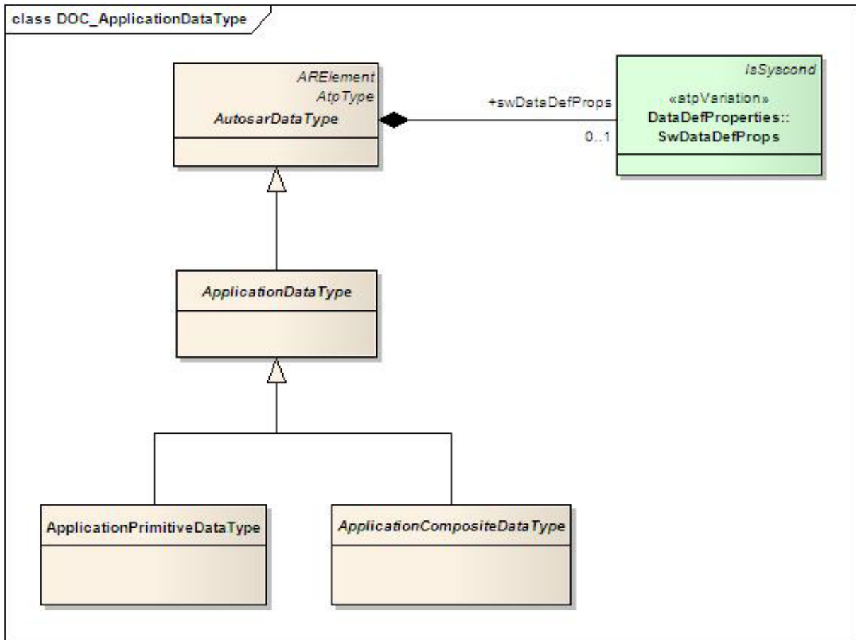
Figure 4.19: Application Data Type
