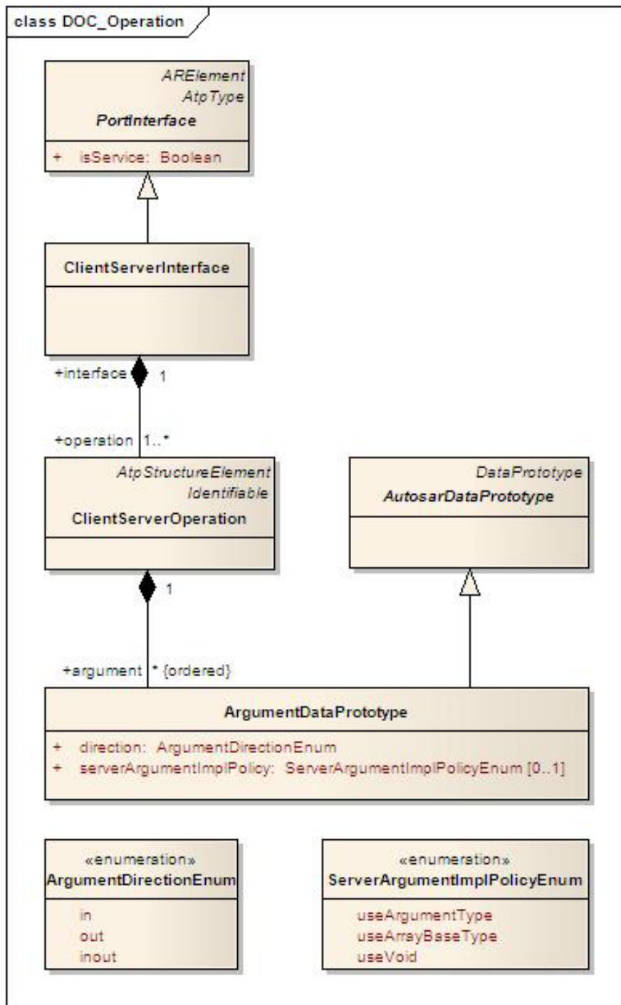
Figure 4.15: ClientServerInterface
