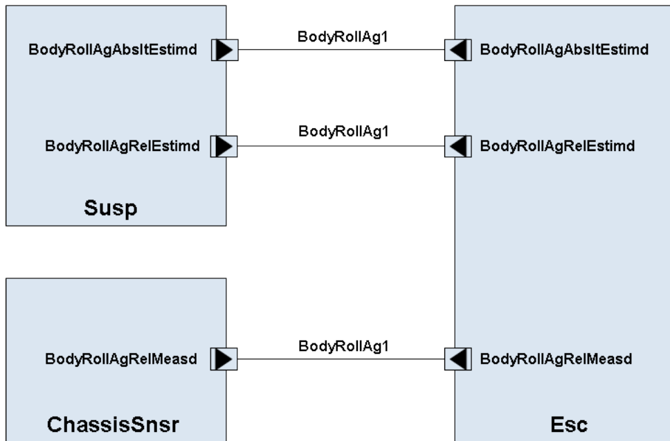
Figure 8.11: PortInterface reusability example
