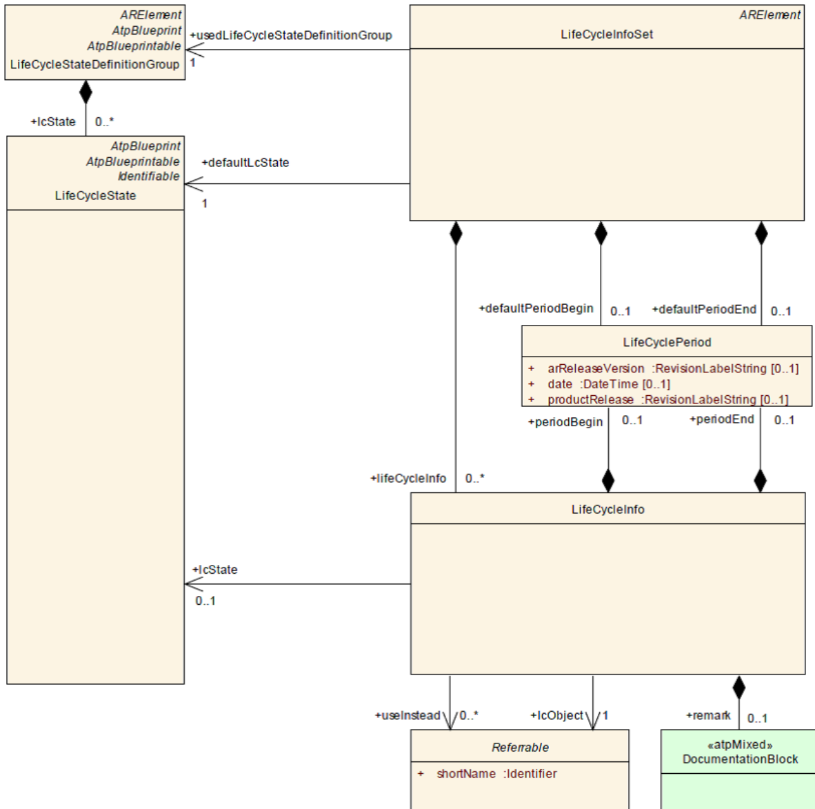
Figure 6.2: Definition of Life Cycle - meta model representation
