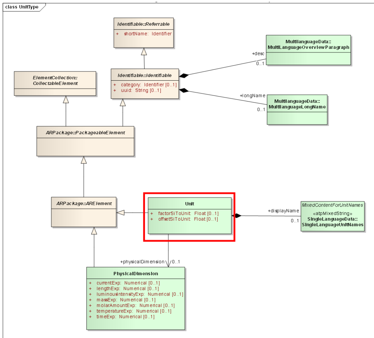
Figure 9.2: Cut-out from the meta-model defining the structure of the element Unit
