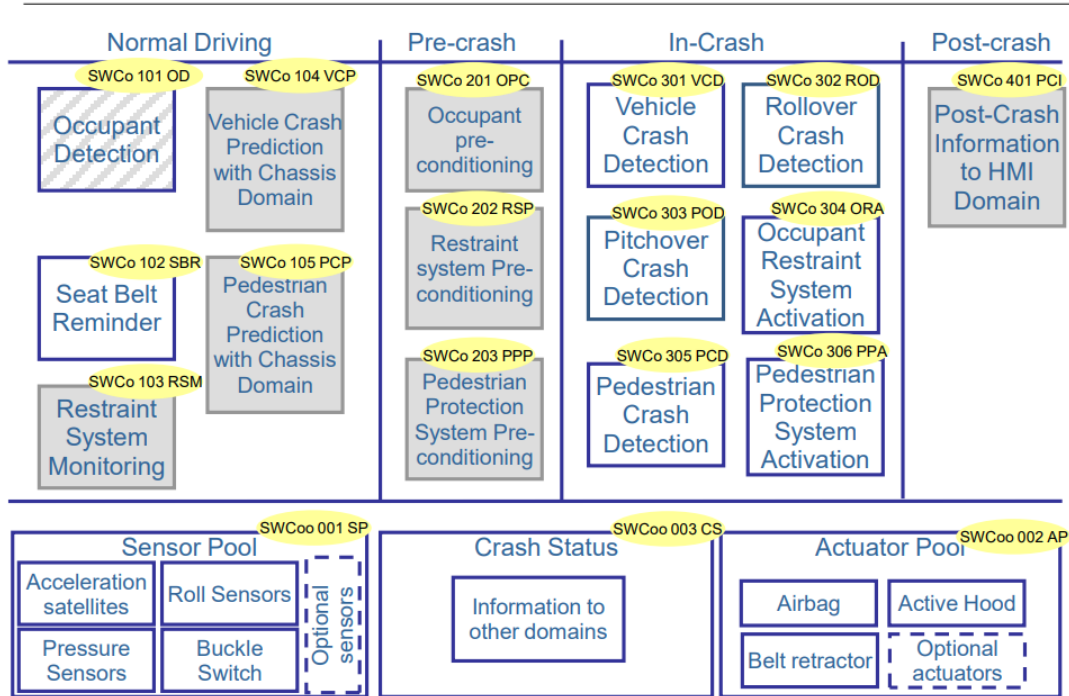
Figure 3.1: OPSS SWCo Decomposition (Exemplary)
