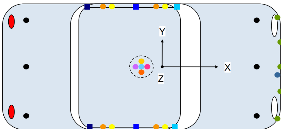
Figure 4.1: Sensor Location in the vehicle for In-Crash functions.
