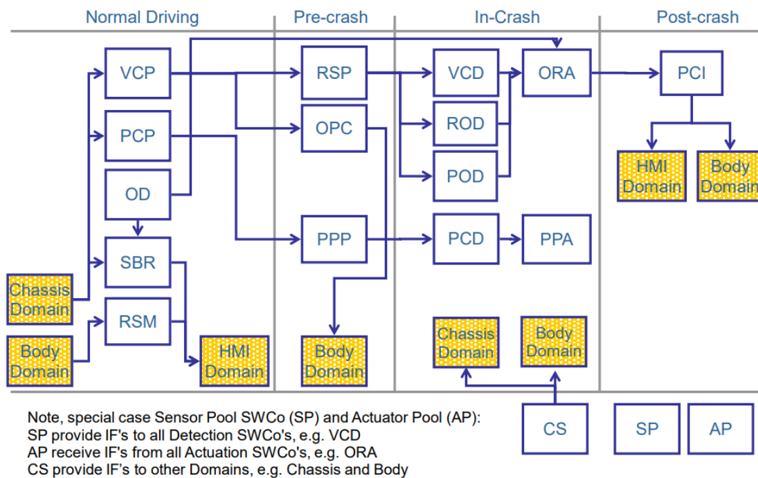
Figure 3.2: Overall SW Composition and Interaction with other Domains
