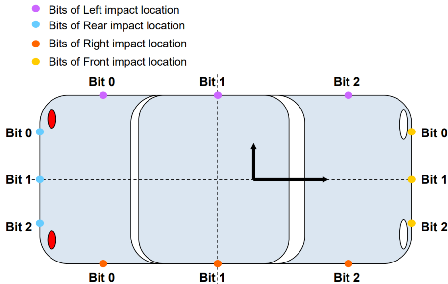
Figure 4.4: Definition of Crash Impact Location around the vehicle perimeter
