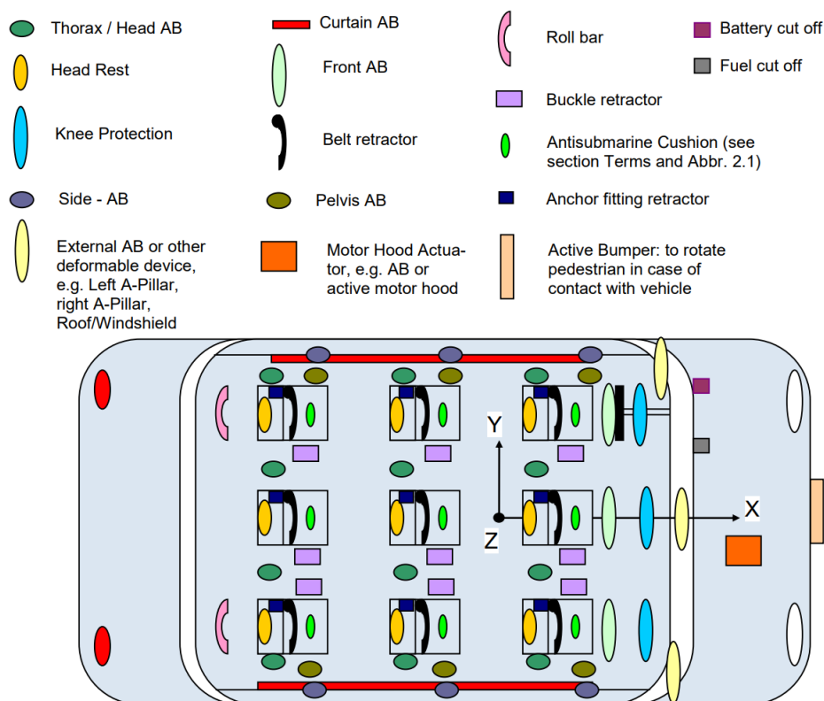
Figure 4.2: Actuator Location in the vehicle for Occupant Protection In-Crash functions
