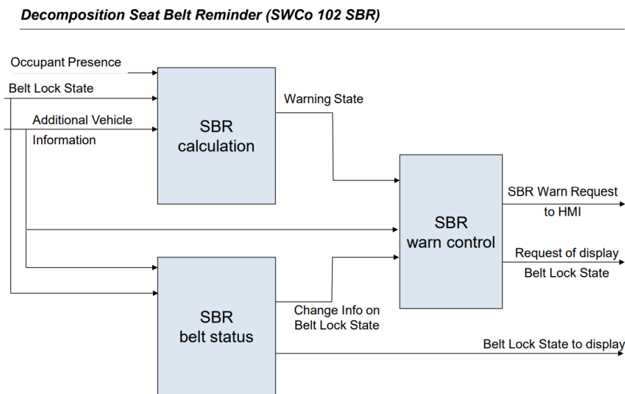
Figure 4.3: Seat Belt Reminder Model
