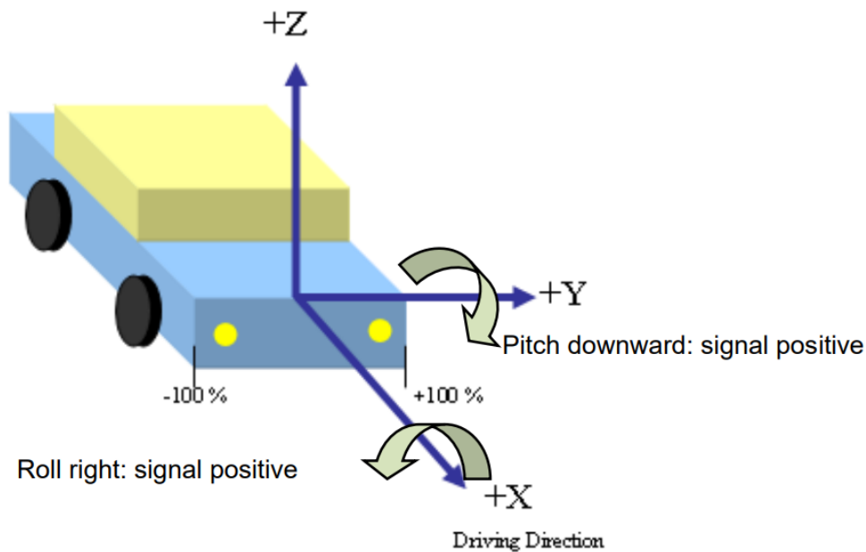
Figure 2.3: Coordinate Reference System for OPSS
