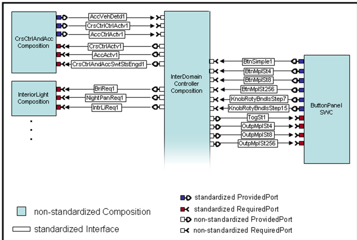
Figure 5.3: Architecture with the InterDomainController and ButtonPanel
