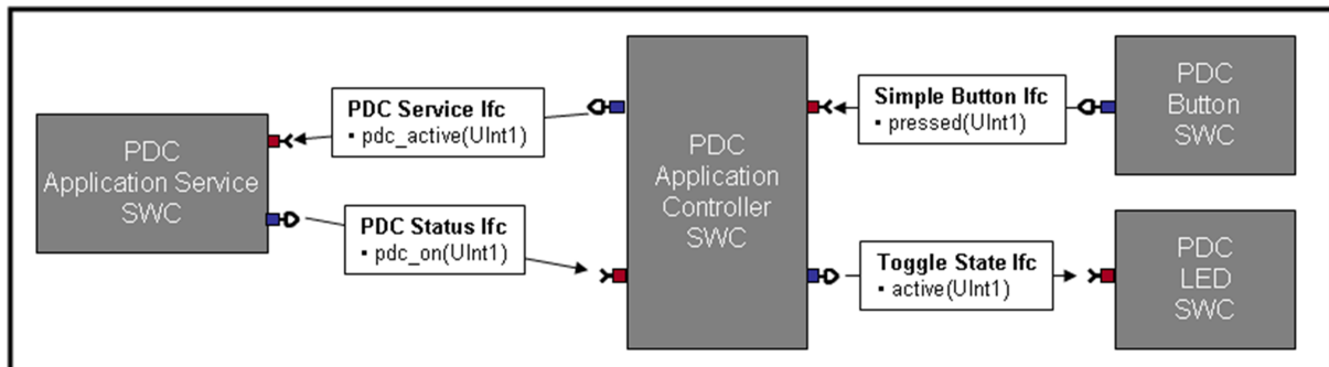
Figure 4.3: Example PDC application using UI device interfaces
