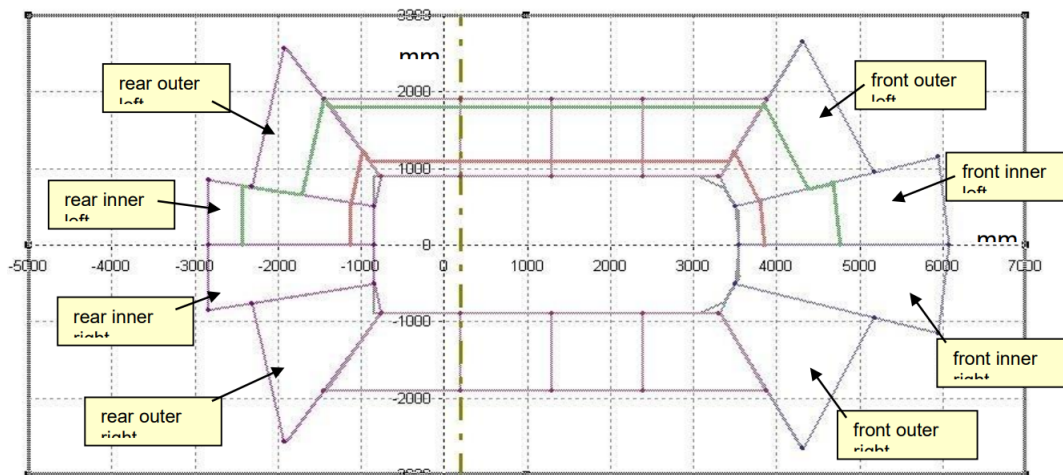
Figure 4.13: Relevant park segments for 8 ultrasonic sensor detection in front and rear
