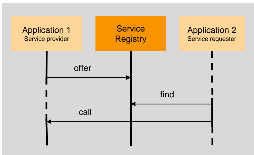
Figure 6.5: Service Discovery
