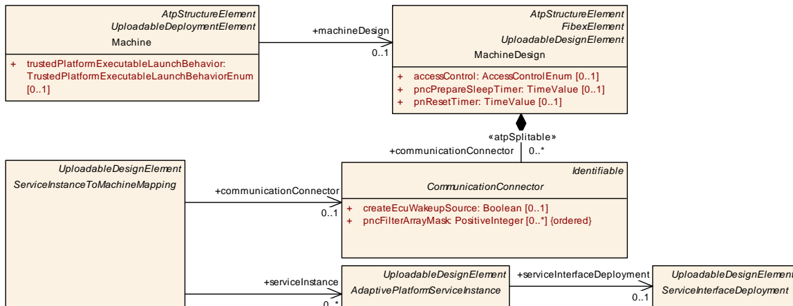
Figure 6.3: Service InstanceToMachineMapping
