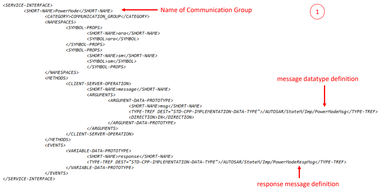
Figure 6.10: CG Template Service Interface Description, example PowerMode
