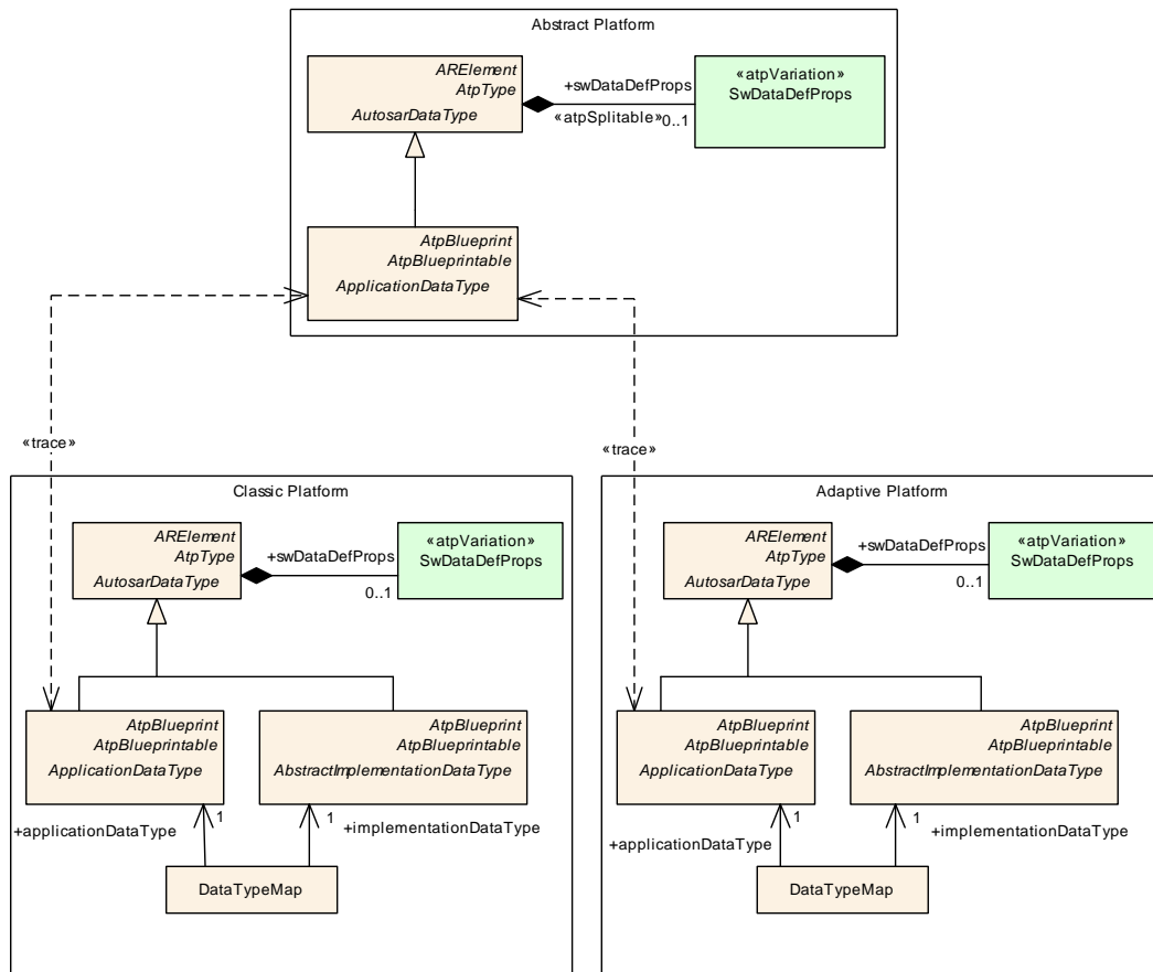
Figure A.1: Data type tracing
