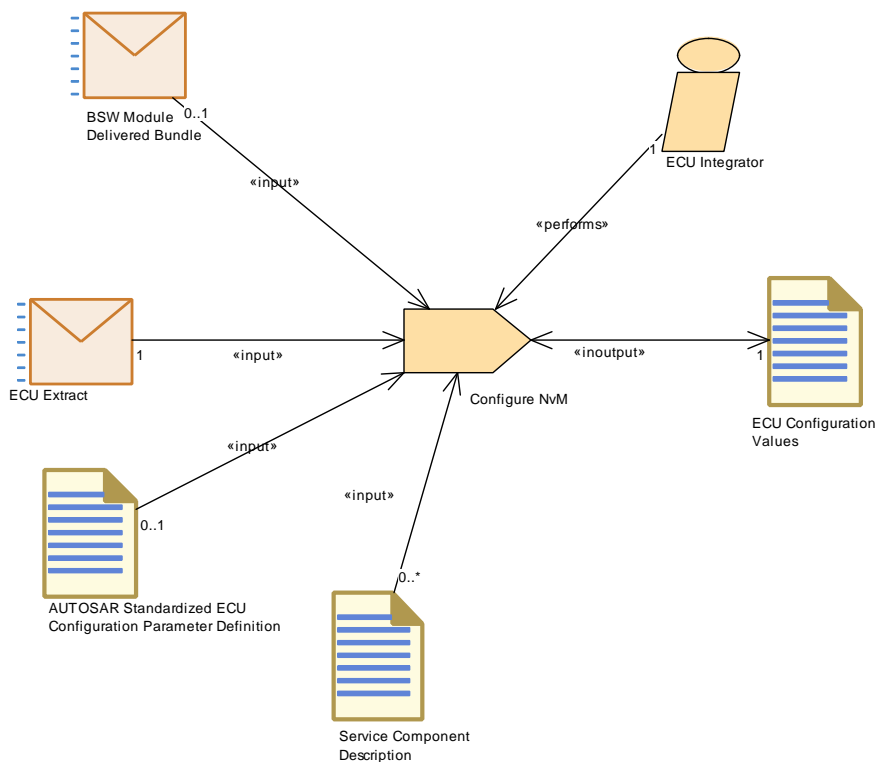
Figure 3.129: Configure NvM
