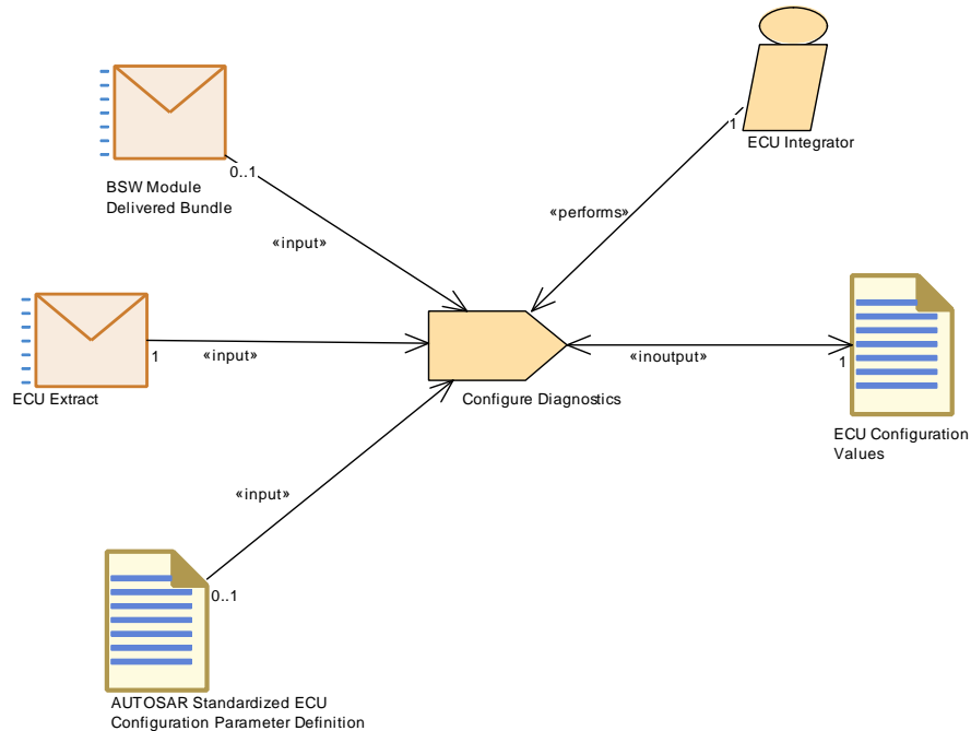
Figure 3.130: Configure Diagnostics
