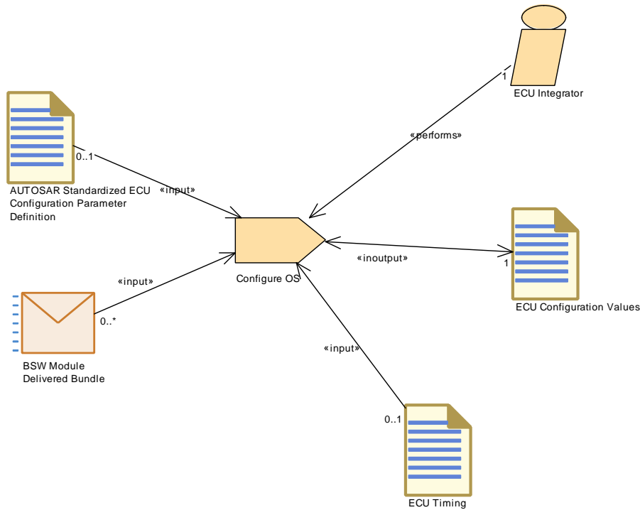
Figure 3.125: Configure OS
