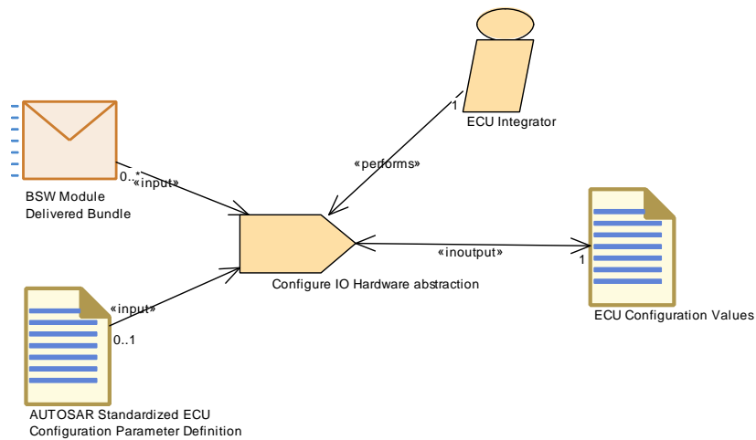
Figure 3.134: Configure IO Hardware Abstraction
