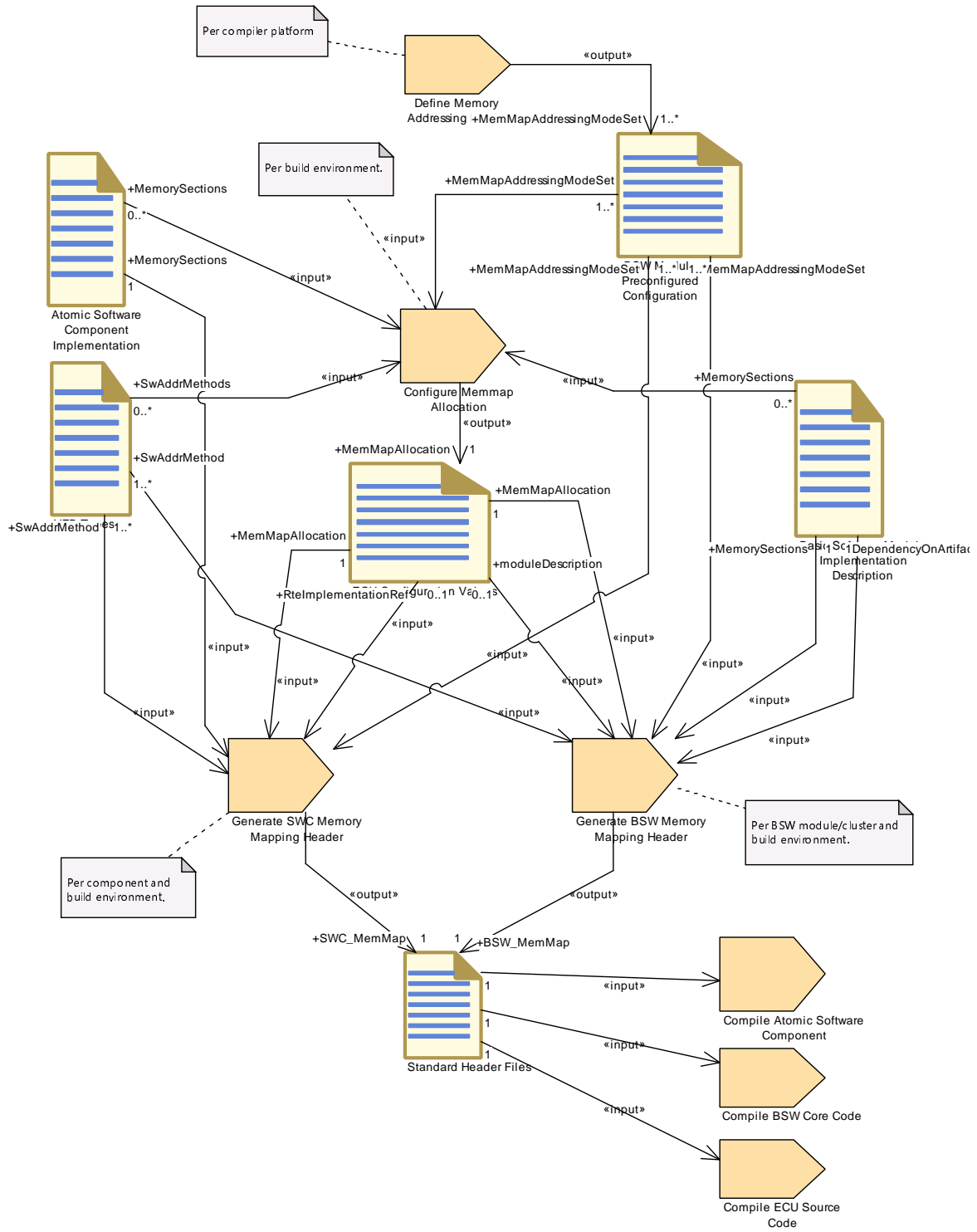
Figure 2.63: Memory Mapping - Detailed view with work products
