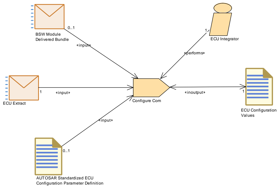
Figure 3.133: Configure COM
