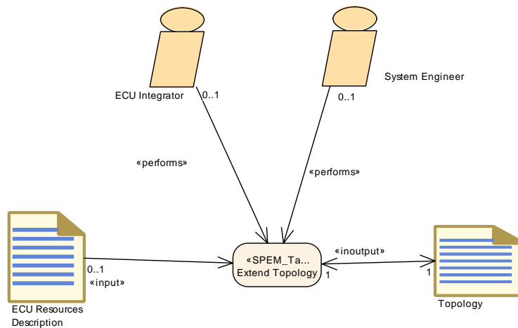
Figure 3.56: Extend Topology
