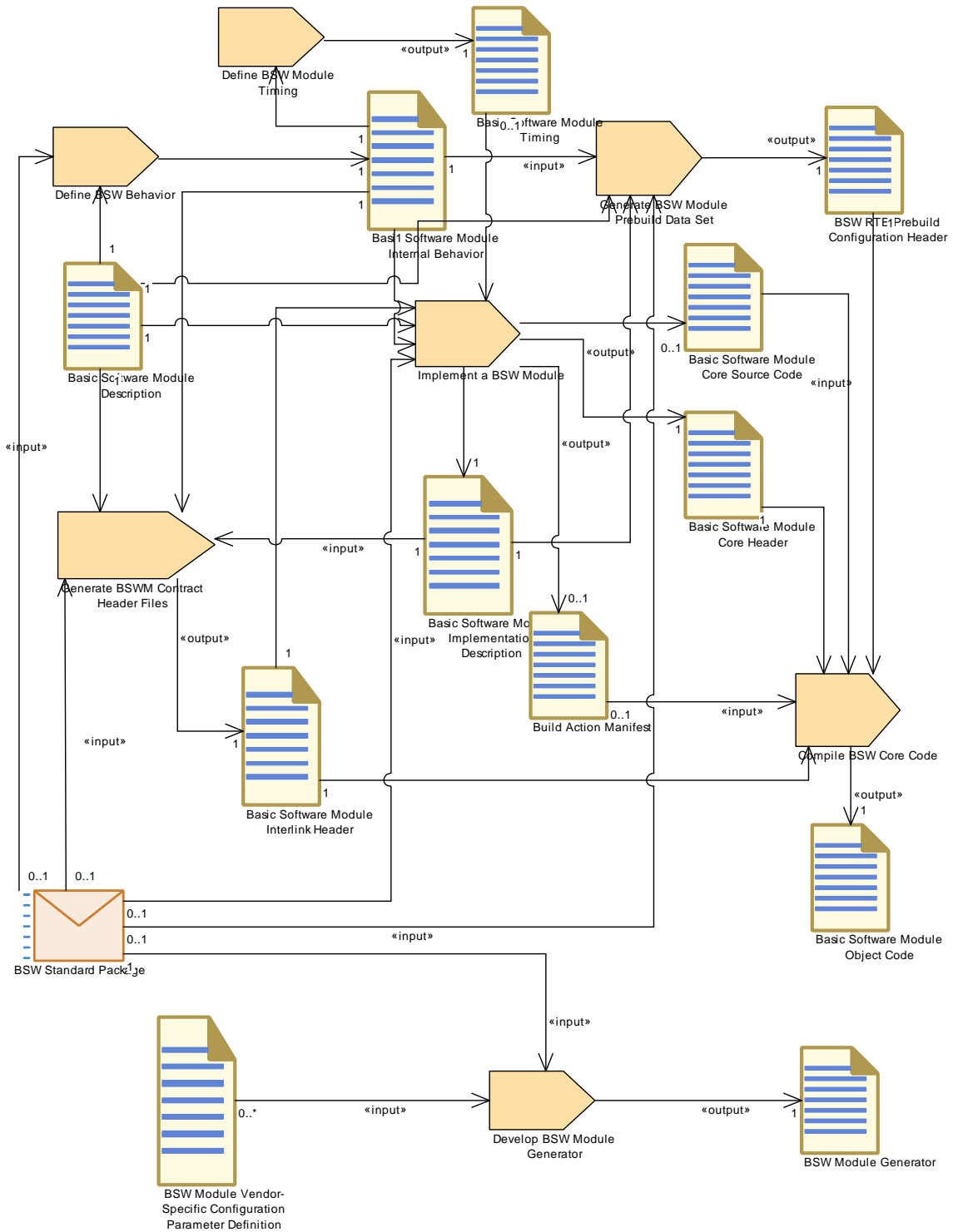
Figure 2.40: Develop Basic Software Module
