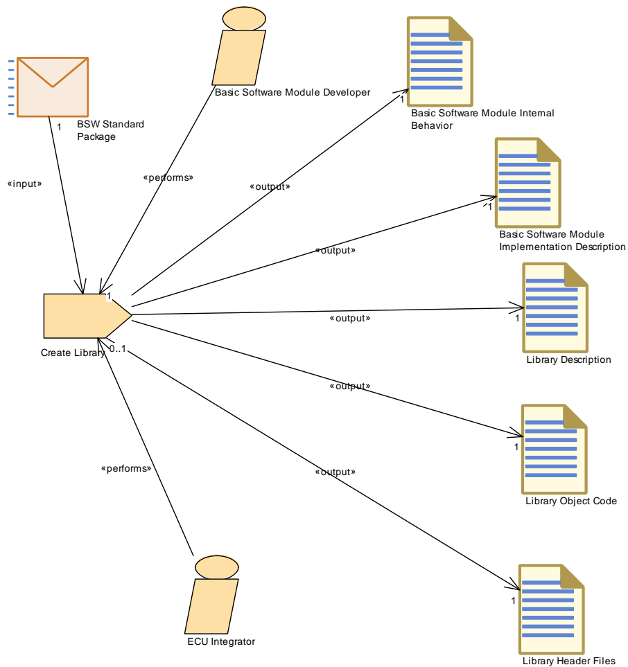
Figure 3.112: Create Library
