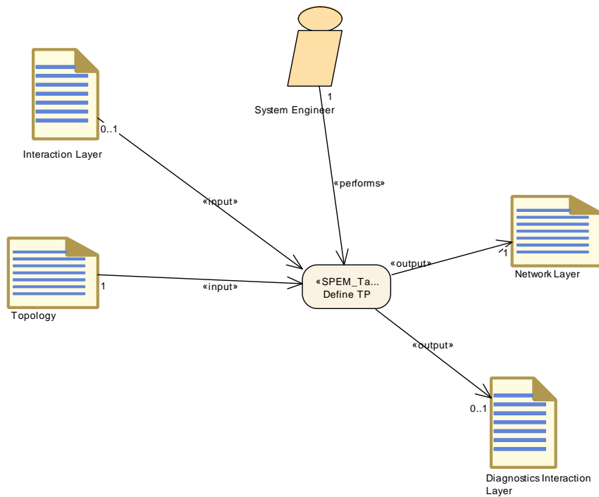
Figure 3.70: Define TP
