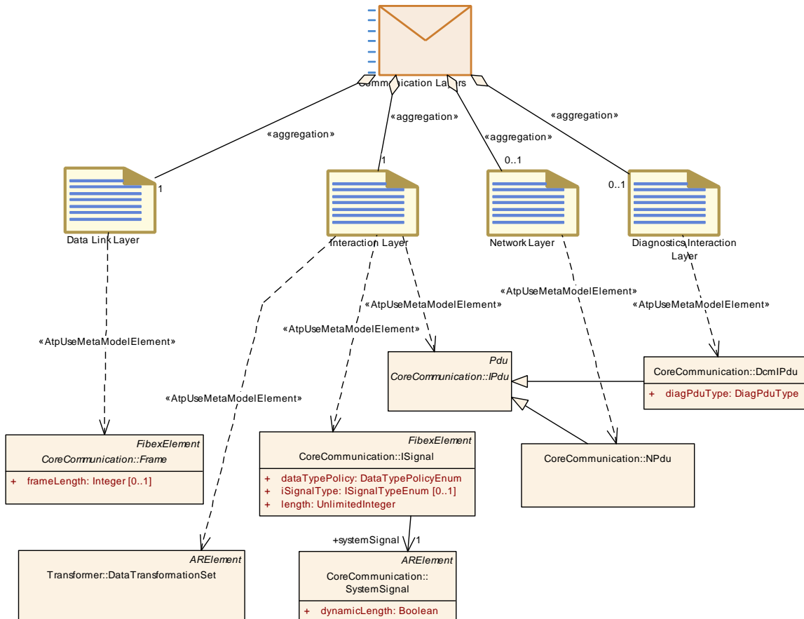
Figure 3.77: Communication Layers
