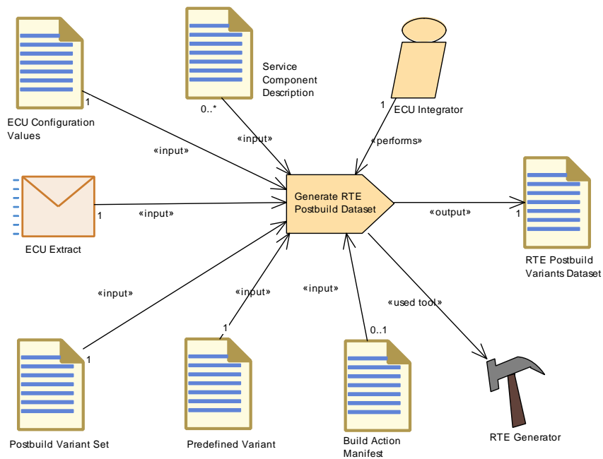
Figure 3.146: Generate RTE Postbuild Dataset
