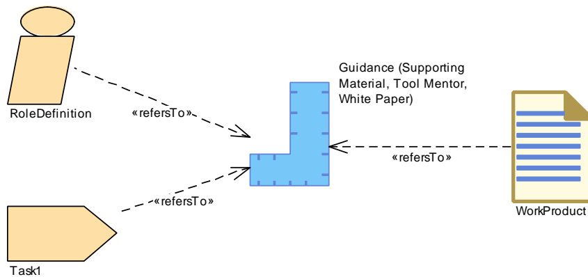
Figure 1.6: Guidance Overview
