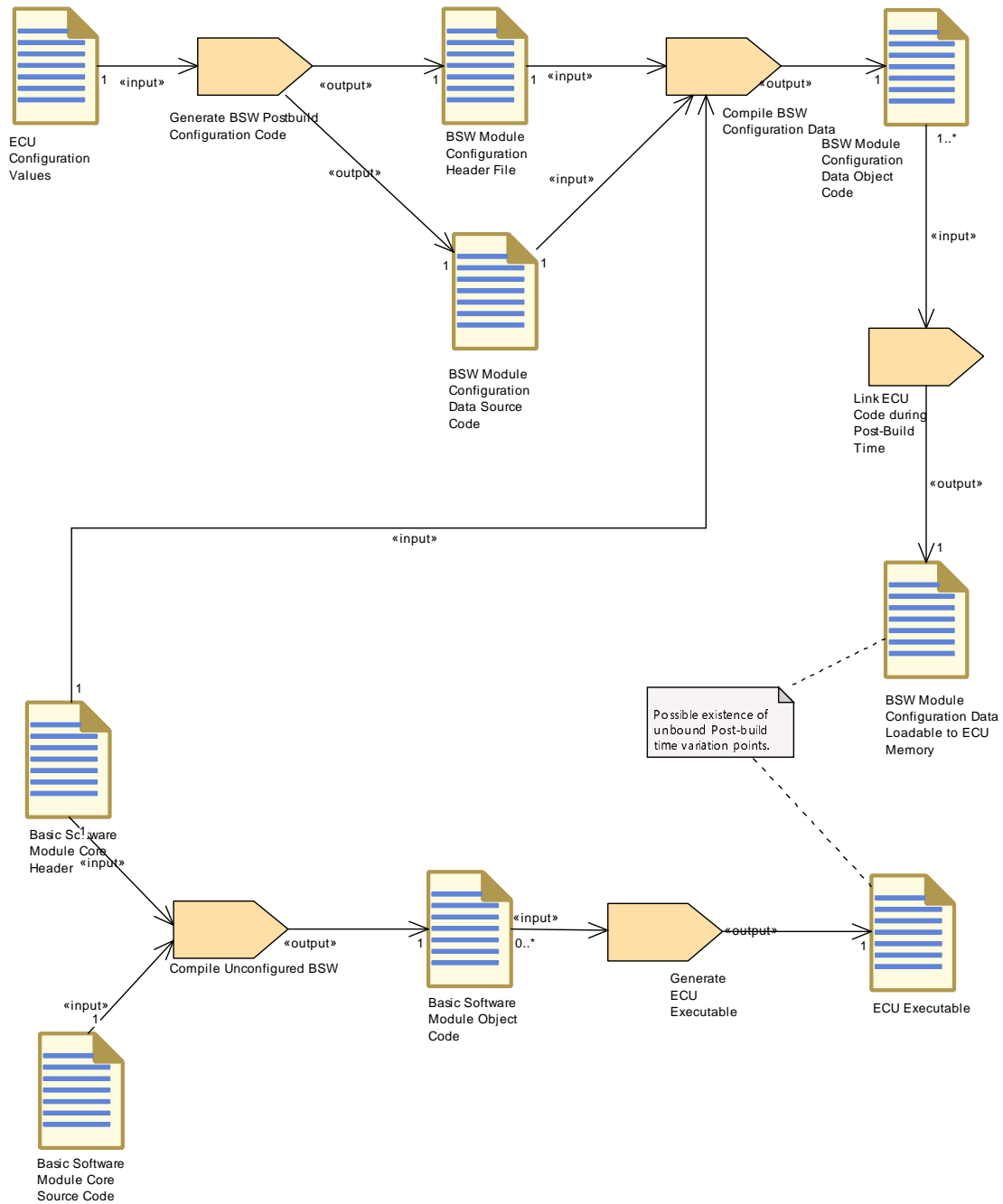
Figure 2.55: Overview of initial Post-Build Configuration
