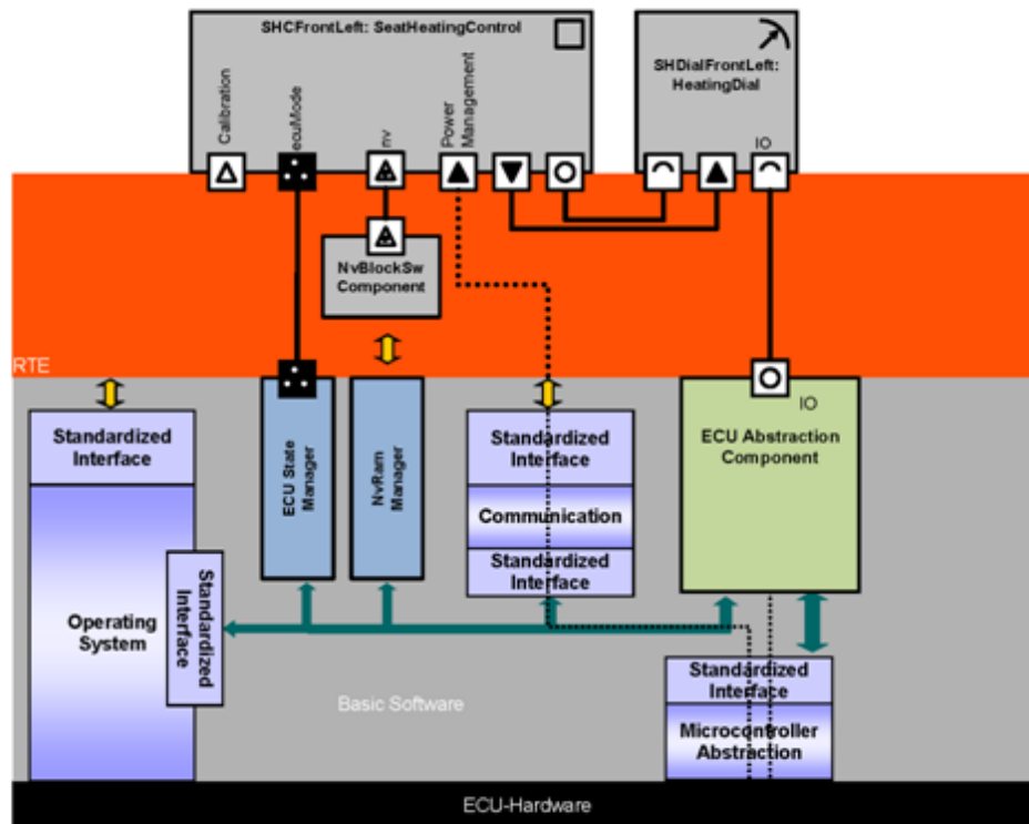
Figure 3.4: Access to ECU Abstraction
