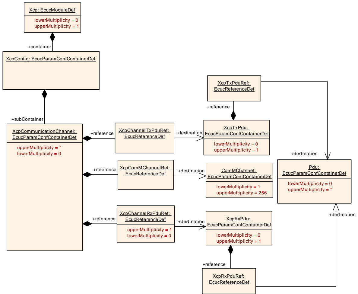
Figure 11: Diagram XcpCommunicationChannel
