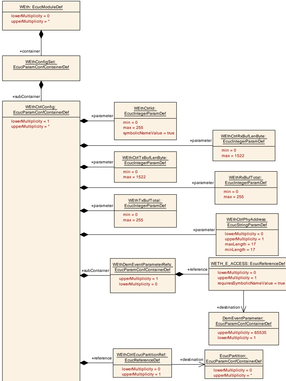
Figure 10.1: WEthCtrlConfig
