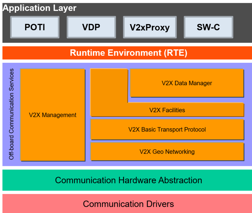
Figure 1 – AUTOSAR BSW software architecture – V2xBtp module scope
