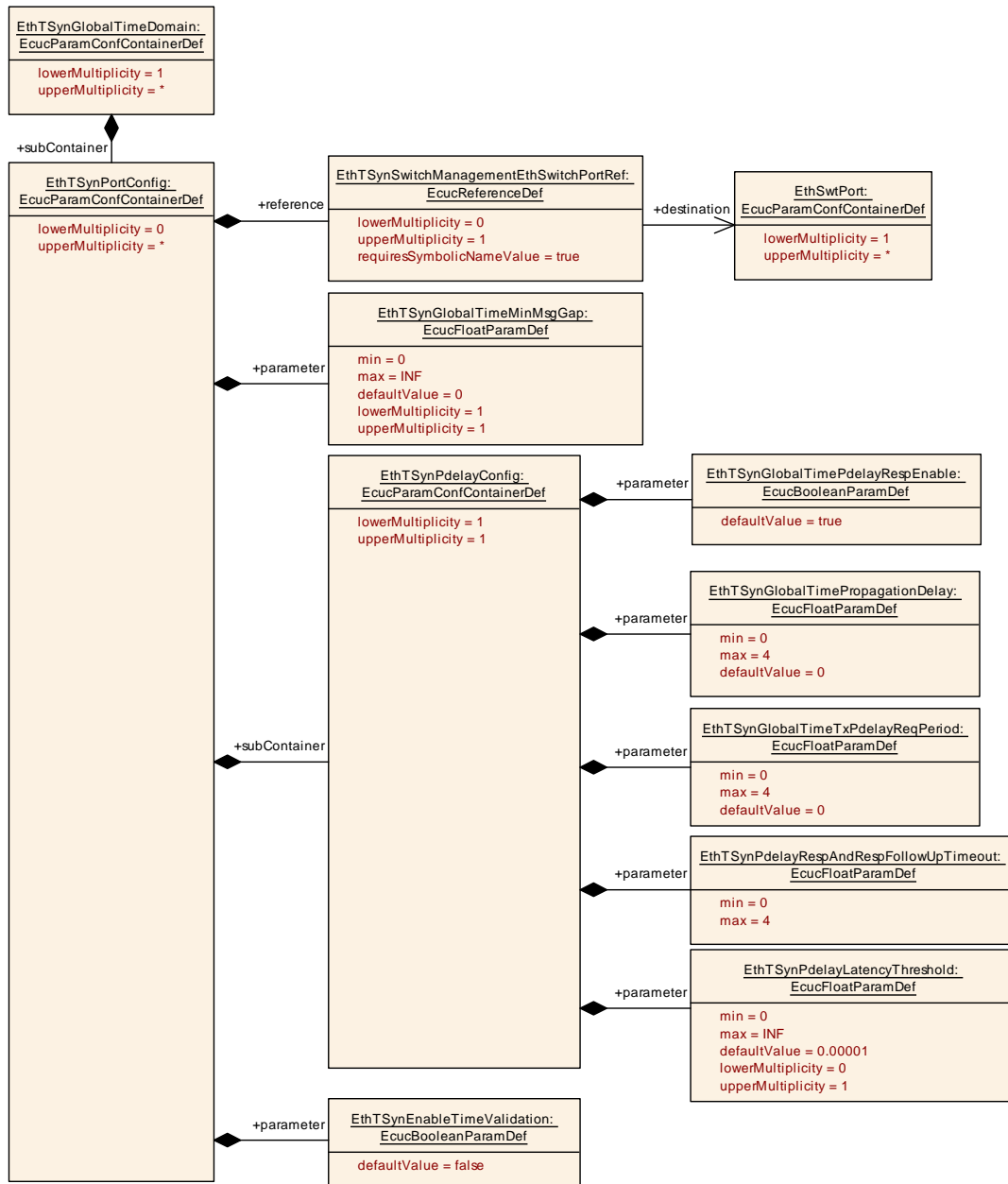
Figure 10.3: EthTSyn_PortConfig
