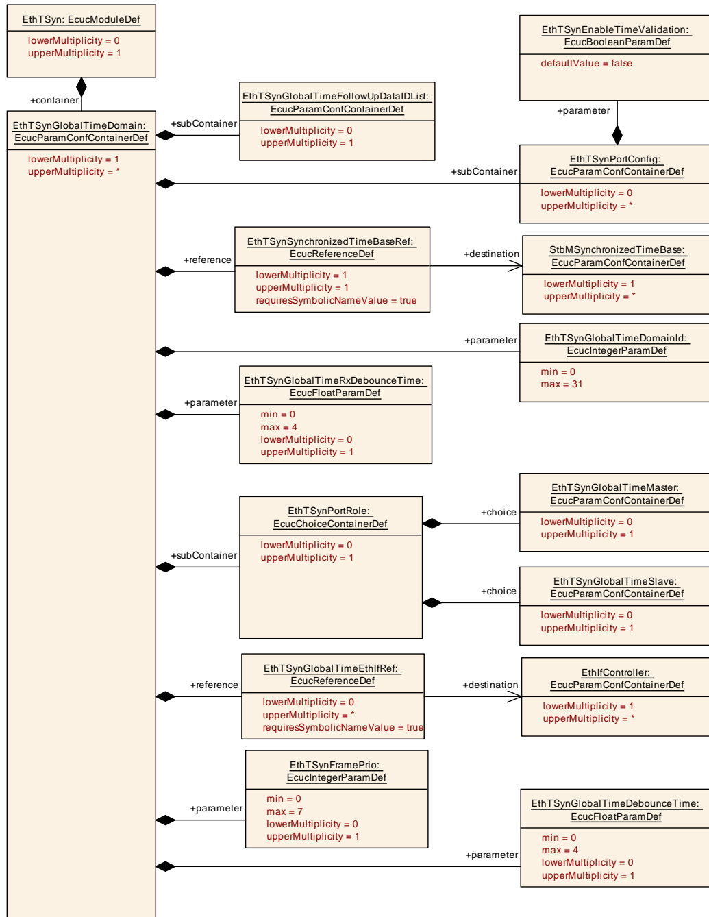
Figure 10.1: EthTSynGlobalTimeDomain
