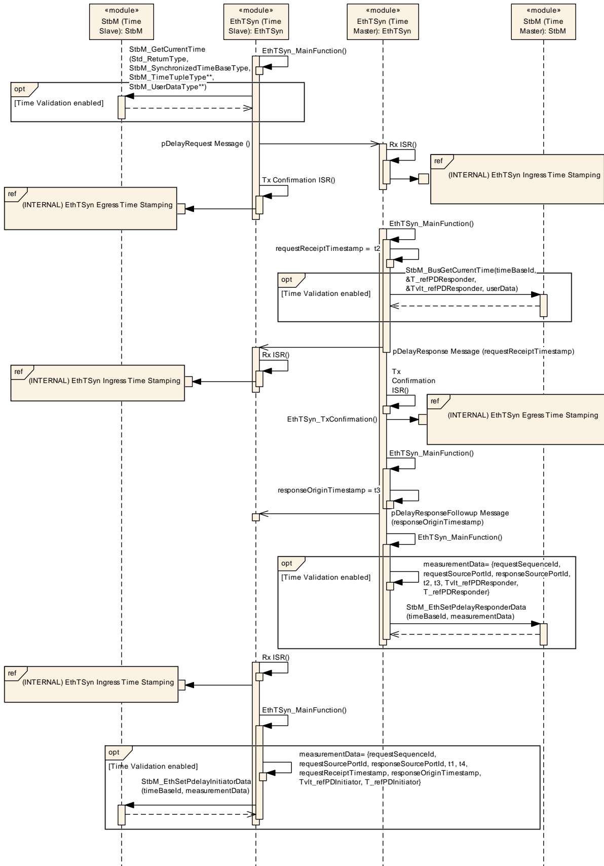
Figure 9.3: : Pdelay Sequence
