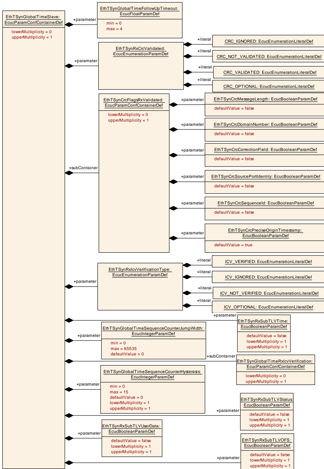
Figure 10.6: EthTsyn_GlobalTimeSlave
