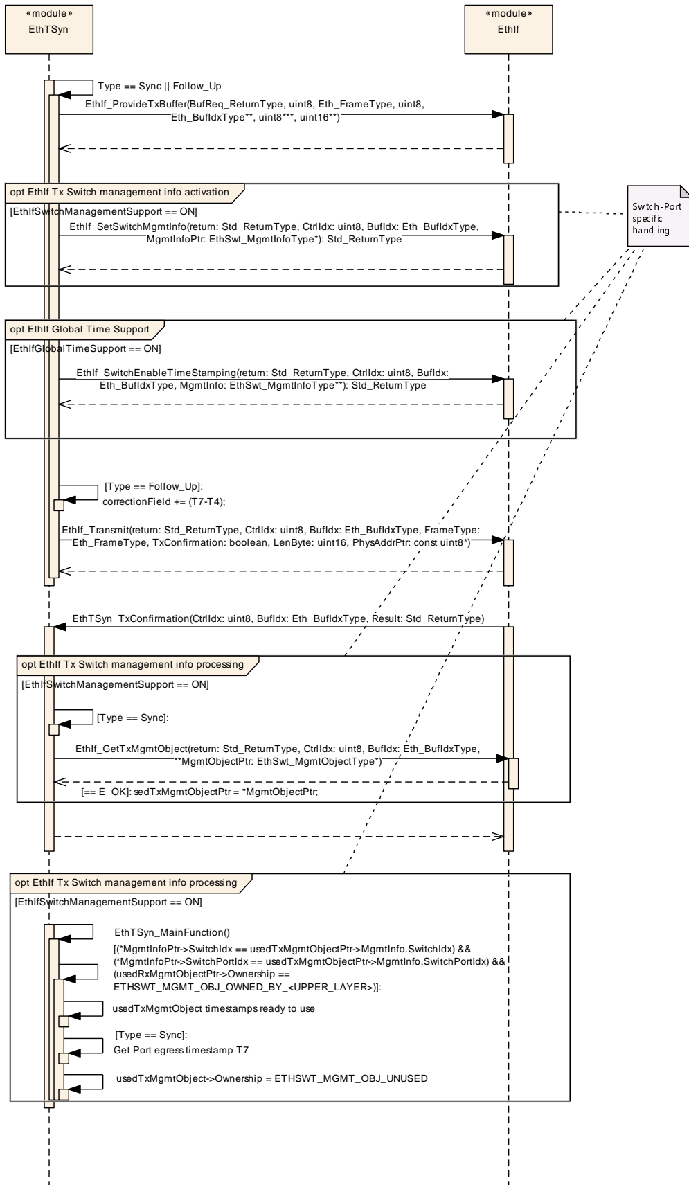
Figure 9.8: EthTSyn_SwitchWithoutGTM_Sync_Follow_Up_Tx
