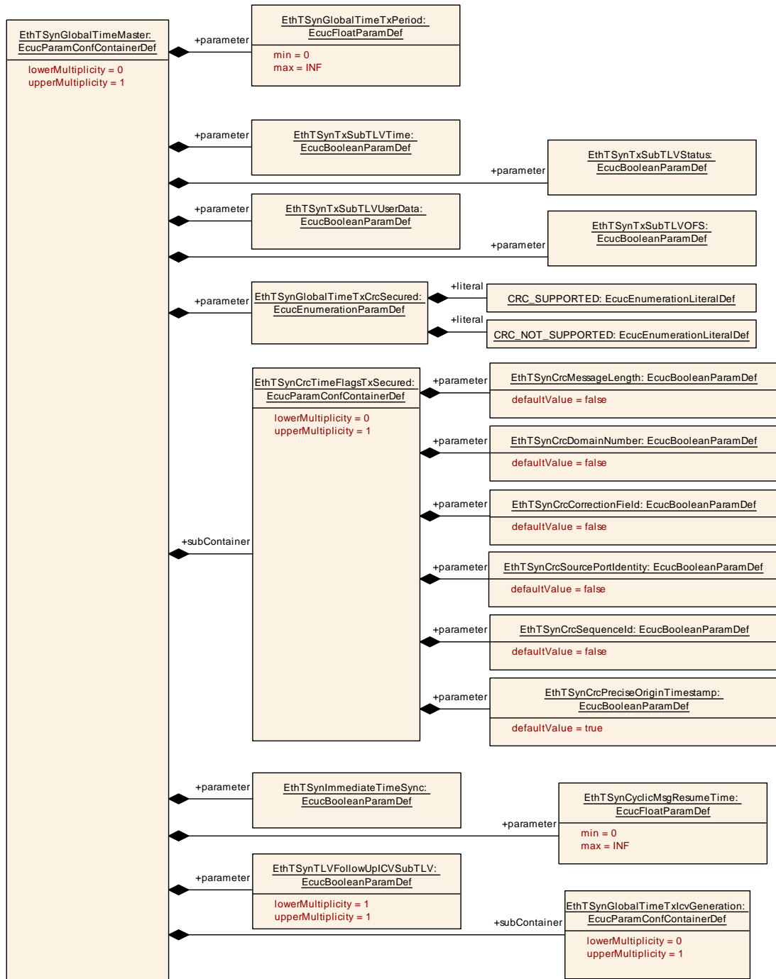
Figure 10.5: EthTSyn_GlobalTimeMaster
