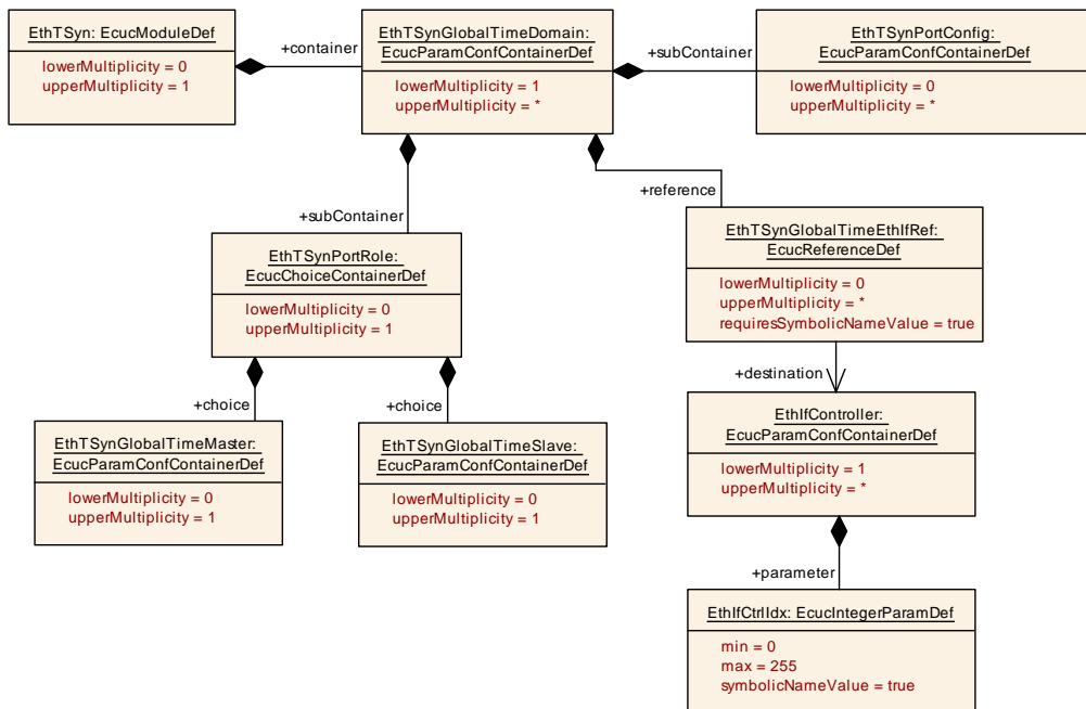
Figure 10.4: EthTSyn_GlobalTimePdu
