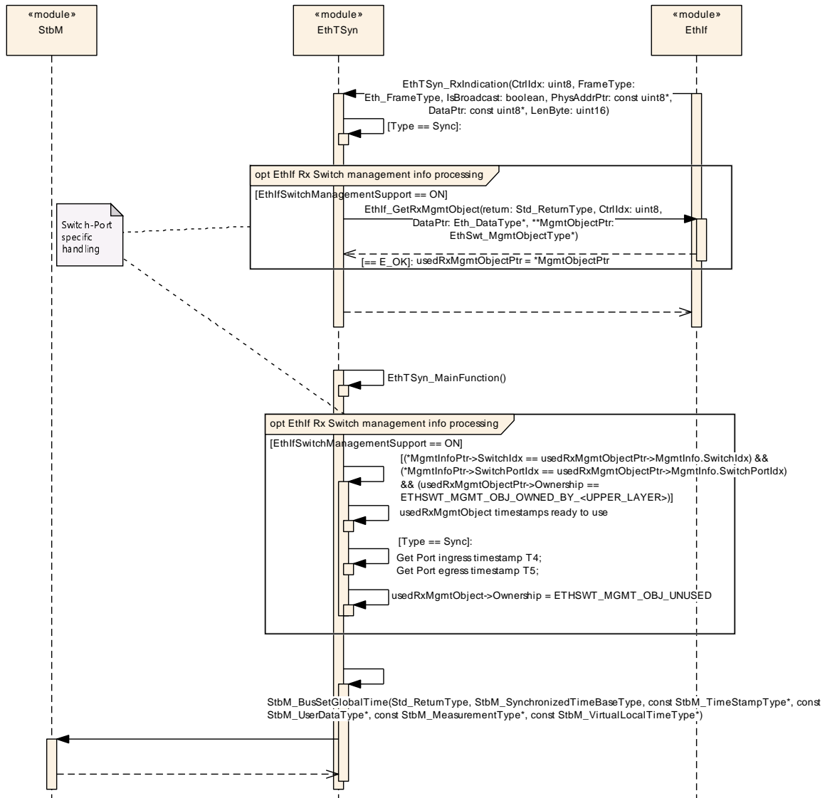
Figure 9.9: EthTSyn_SwitchWithoutGTM_Sync_Follow_Up_Rx
