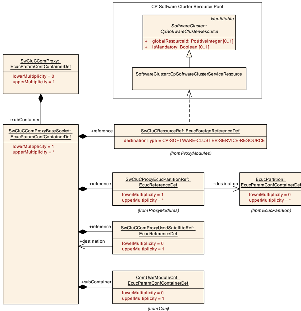
Figure 10.30: Com Proxy Base Socket
