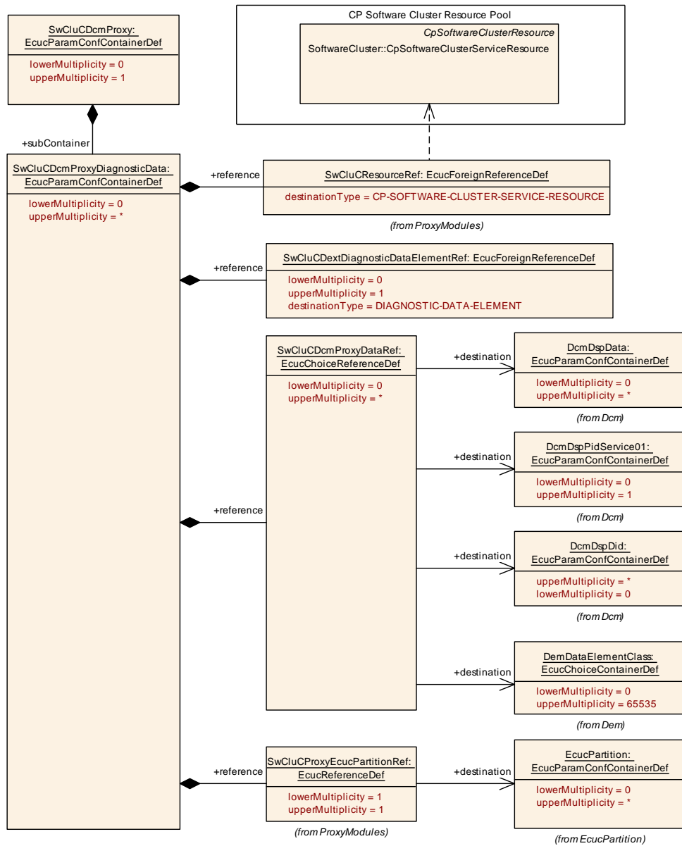
Figure 10.40: Dcm Proxy Diagnostic Data
