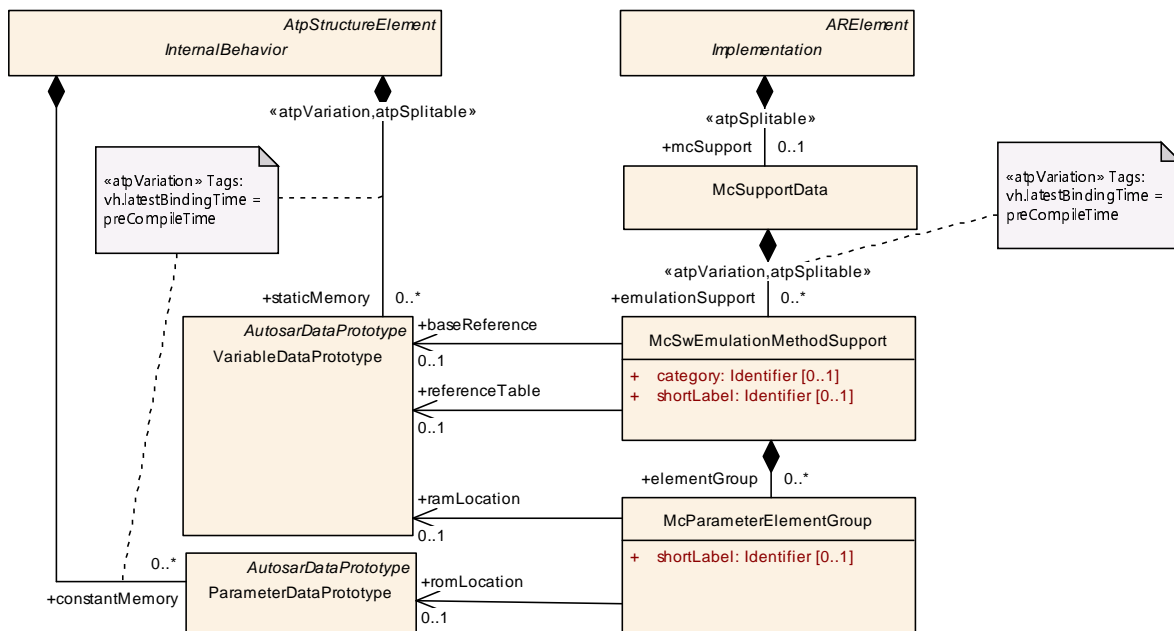
Figure 4.33: Structure of the McSwEmulationMethodSupport element
