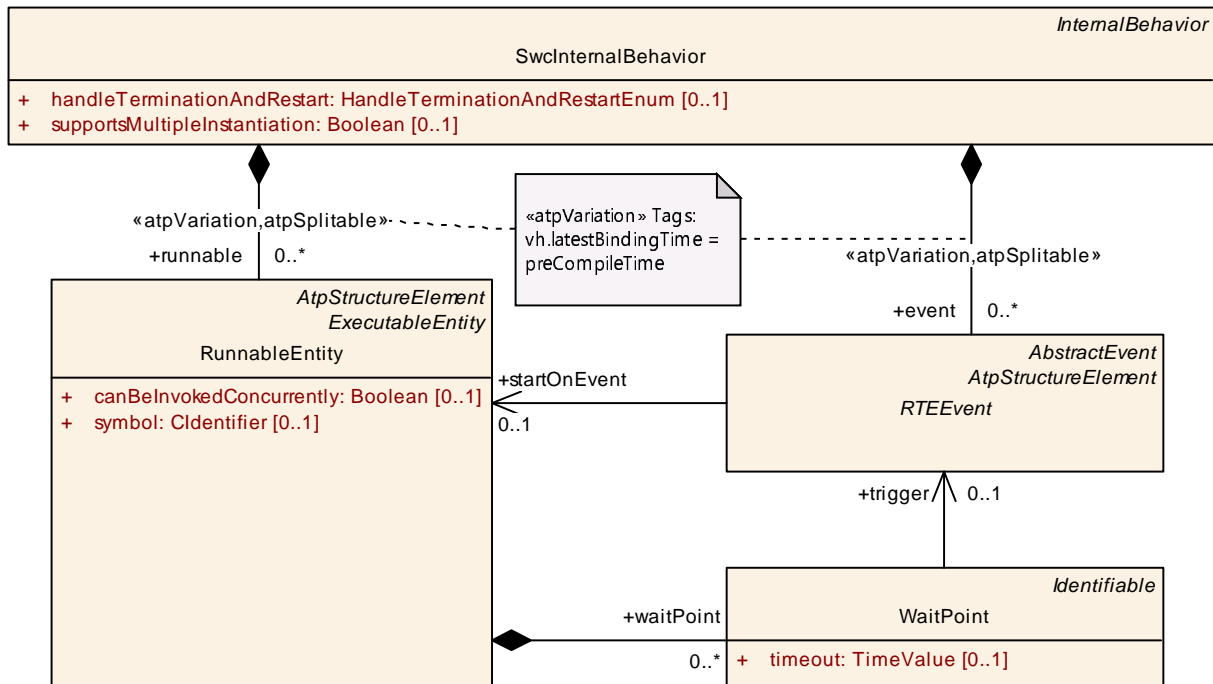
Figure 4.5: Software-component runnable entity, wait points and RTE Events
