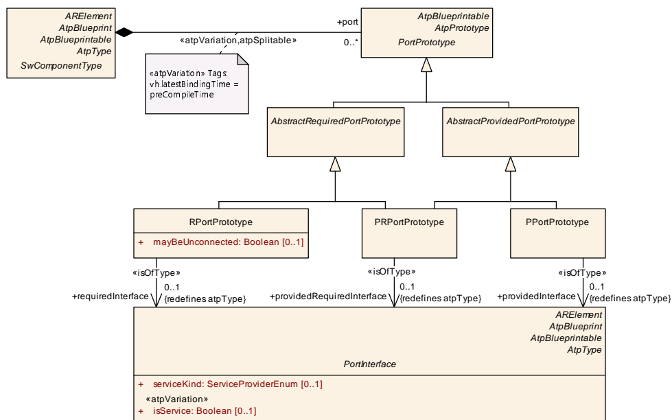
Figure 4.3: Software-Components and Ports
