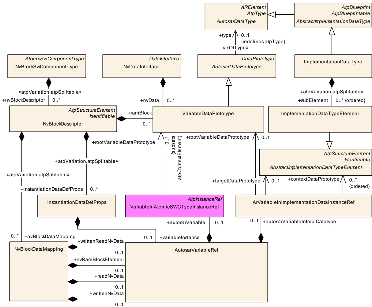
Figure 4.37: NvBlockDataMapping
