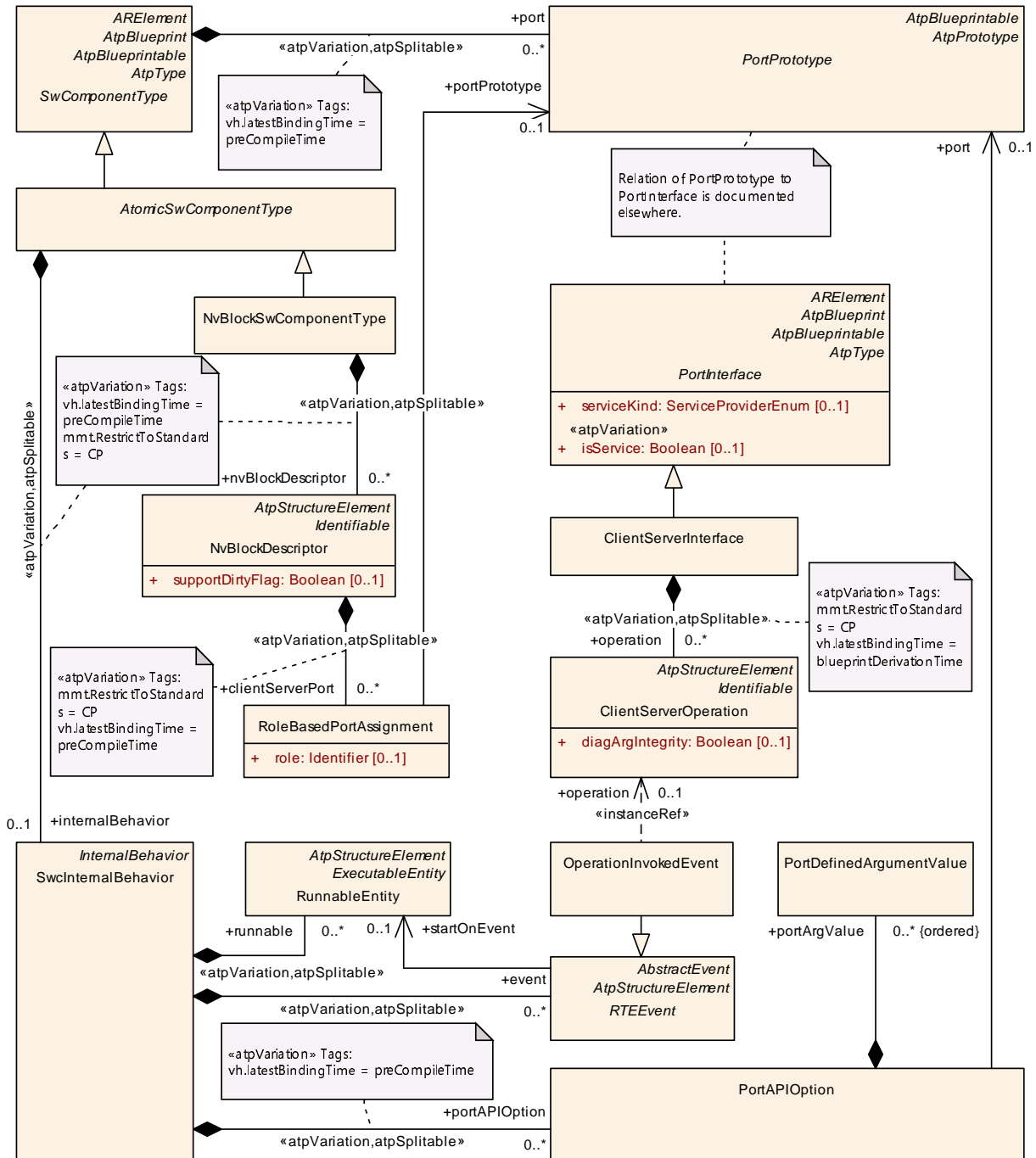
Figure 4.38: SwcInternalBehavior of NvBlockSwComponentTypes
