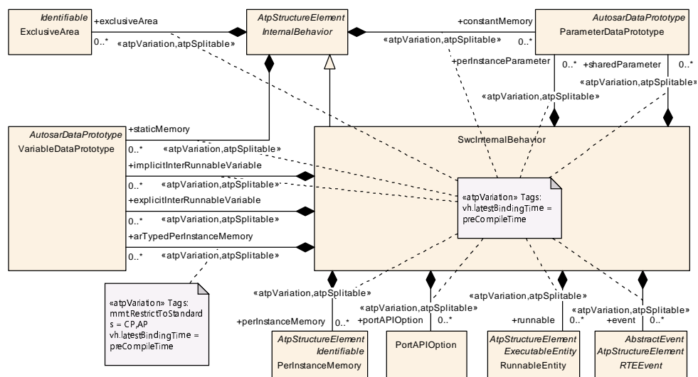
Figure 4.4: Software-component internal behavior
