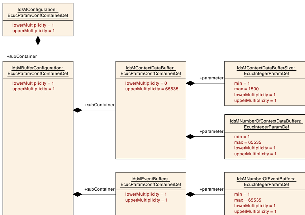
Figure 10.7: IdsM buffer configuration overview
