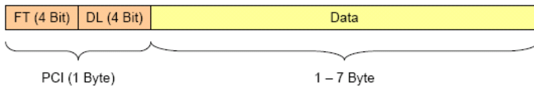
Figure 15: Single Frame ISO 15765-2 J ()
