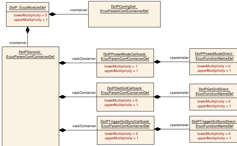
Figure 10.1: DoIPConfig
