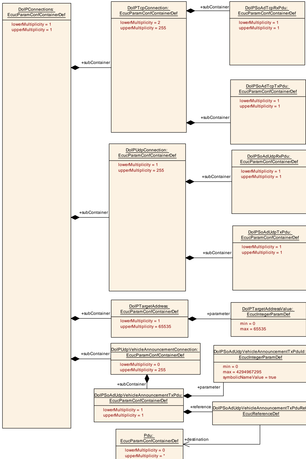
Figure 10.6: DoIPConnections
