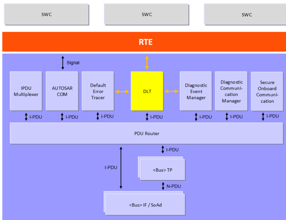
Figure 1 – Location of the Dlt module
