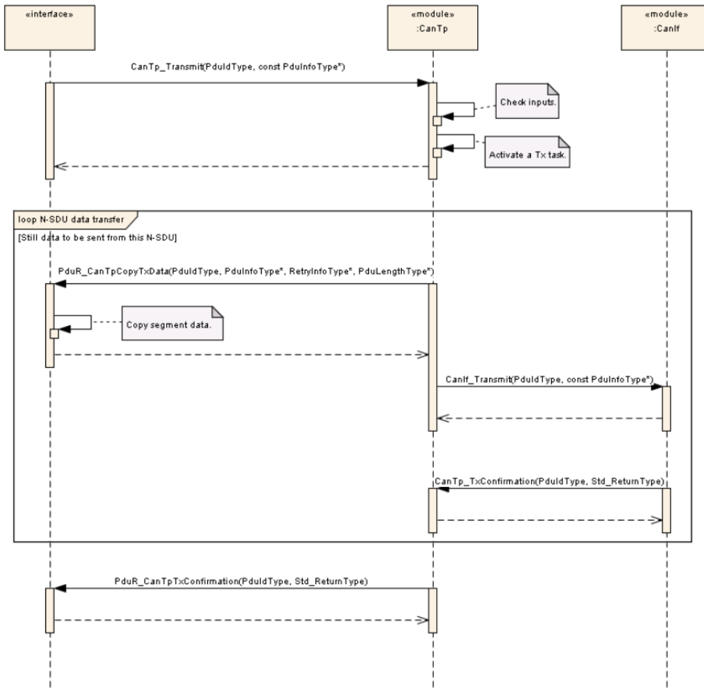
Figure 9.4: Transmit request of larger N-SDU
