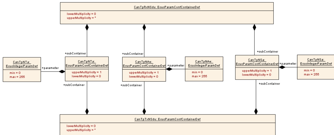
Figure 10.6: CanTpNTa, CanTpNSa and CanTpNAe configuration overview
