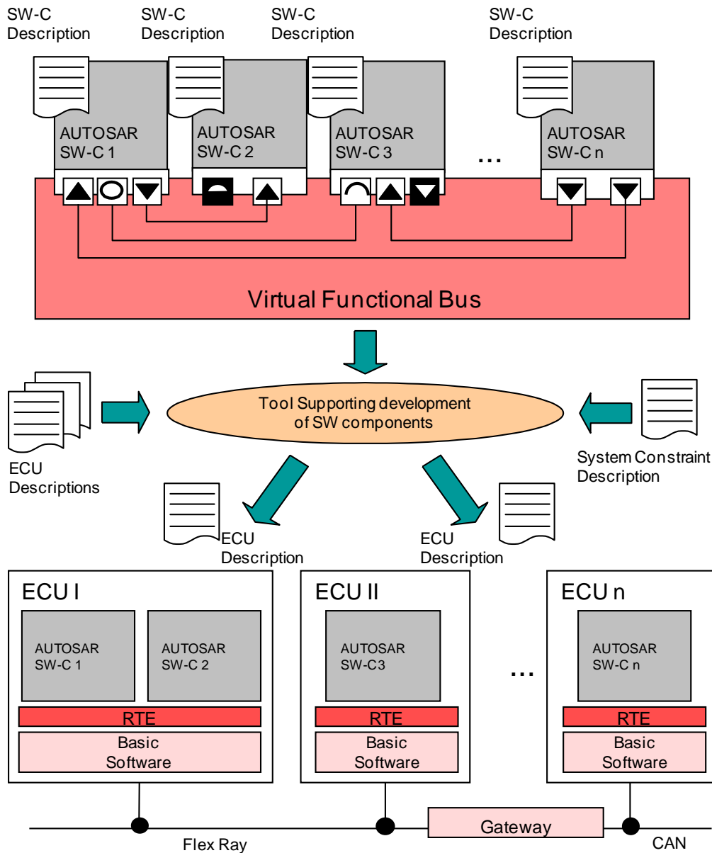
Figure 2.2: Concept of the virtual functional bus
