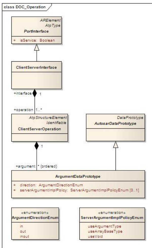
Figure 18: ClientServerInterface
