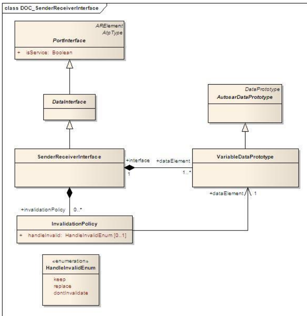
Figure 16: SenderReceiverInterface
