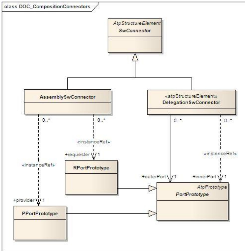
Figure 10: Composition - Connectors
