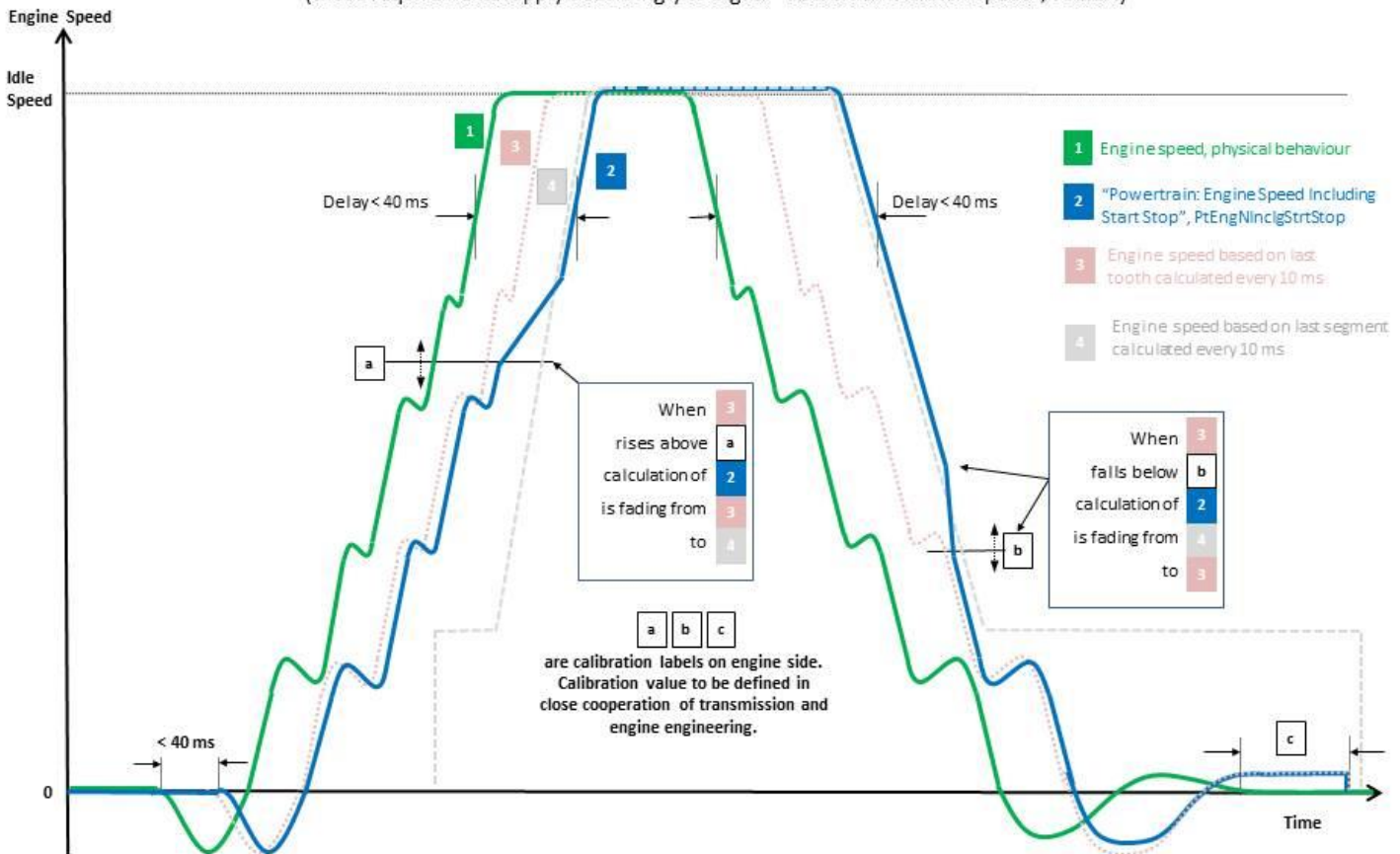
Engine Speed Including Start Stop Composition (these requirements apply accordingly to signal “Powertrain: Clutch Speed”, PtCluN)
