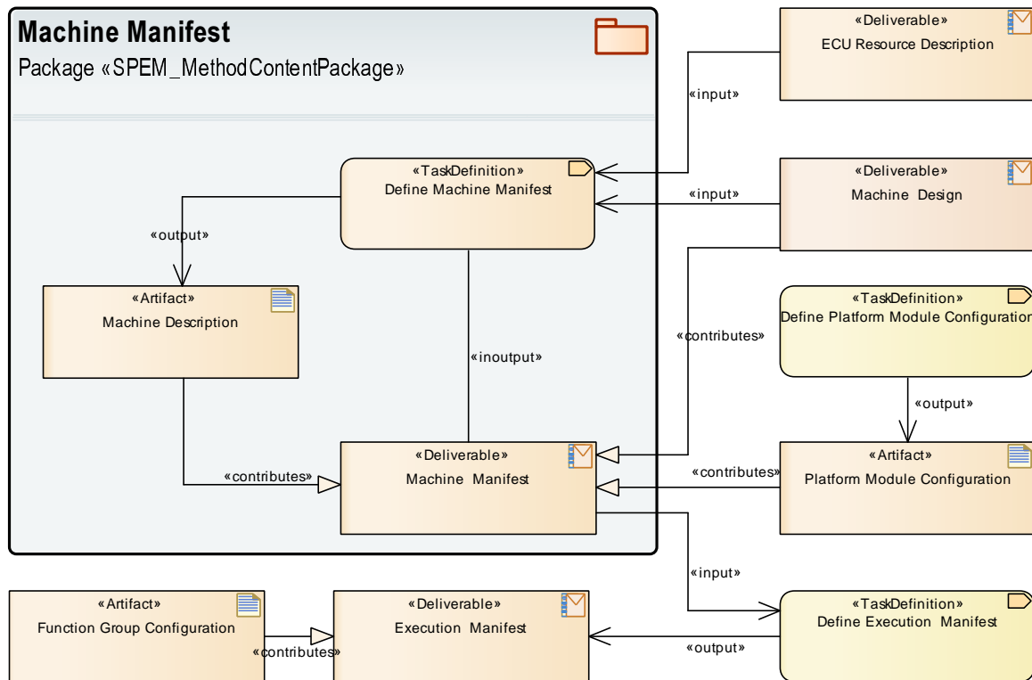
Figure 2.25: Machine Manifest
