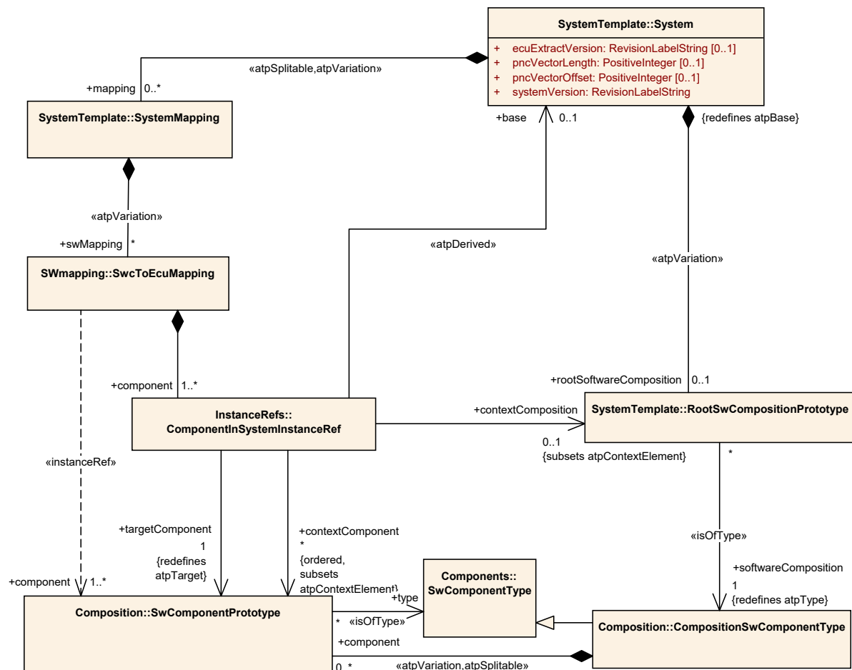
Figure 4.2: Example of an instanceRef association
