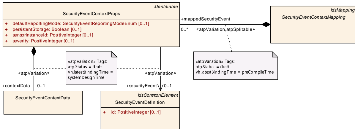
Figure 4.8: Modeling of SecurityEventContextProps
