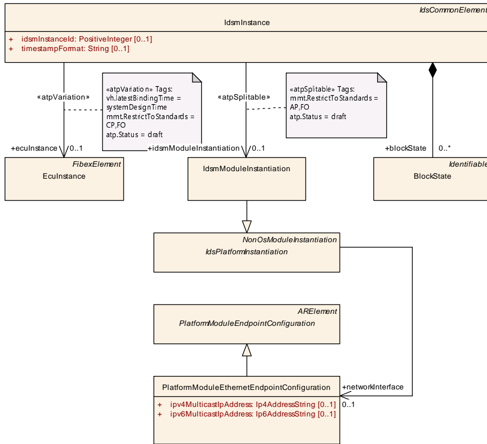
Figure 4.13: Modeling overview of IdsmInstance
