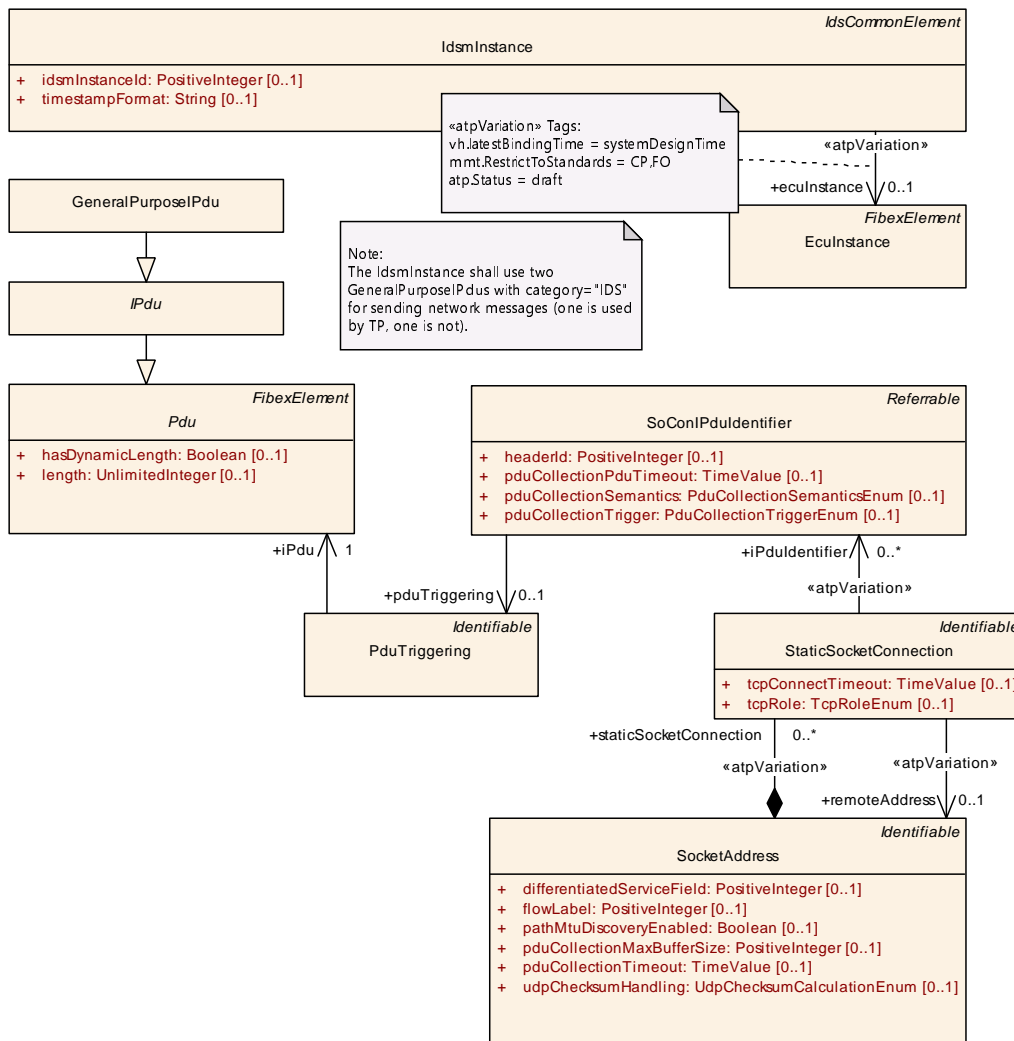
Figure 4.15: Modeling overview of the network configuration of an IdsmInstance on Classic Platform
