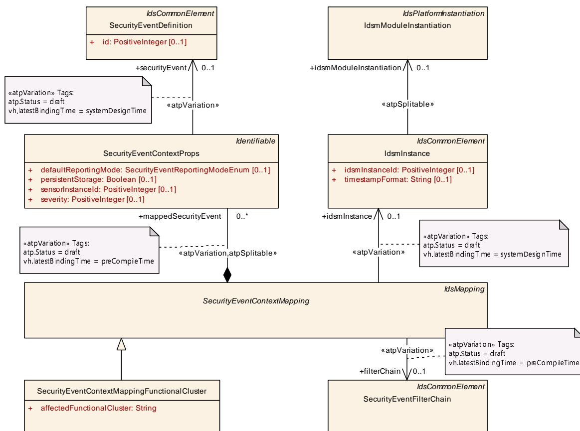
Figure 4.10: Modeling of SecurityEventContextMappingFunctionalCluster
