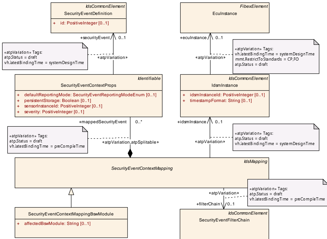
Figure 4.9: Modeling of SecurityEventContextMappingBswModule
