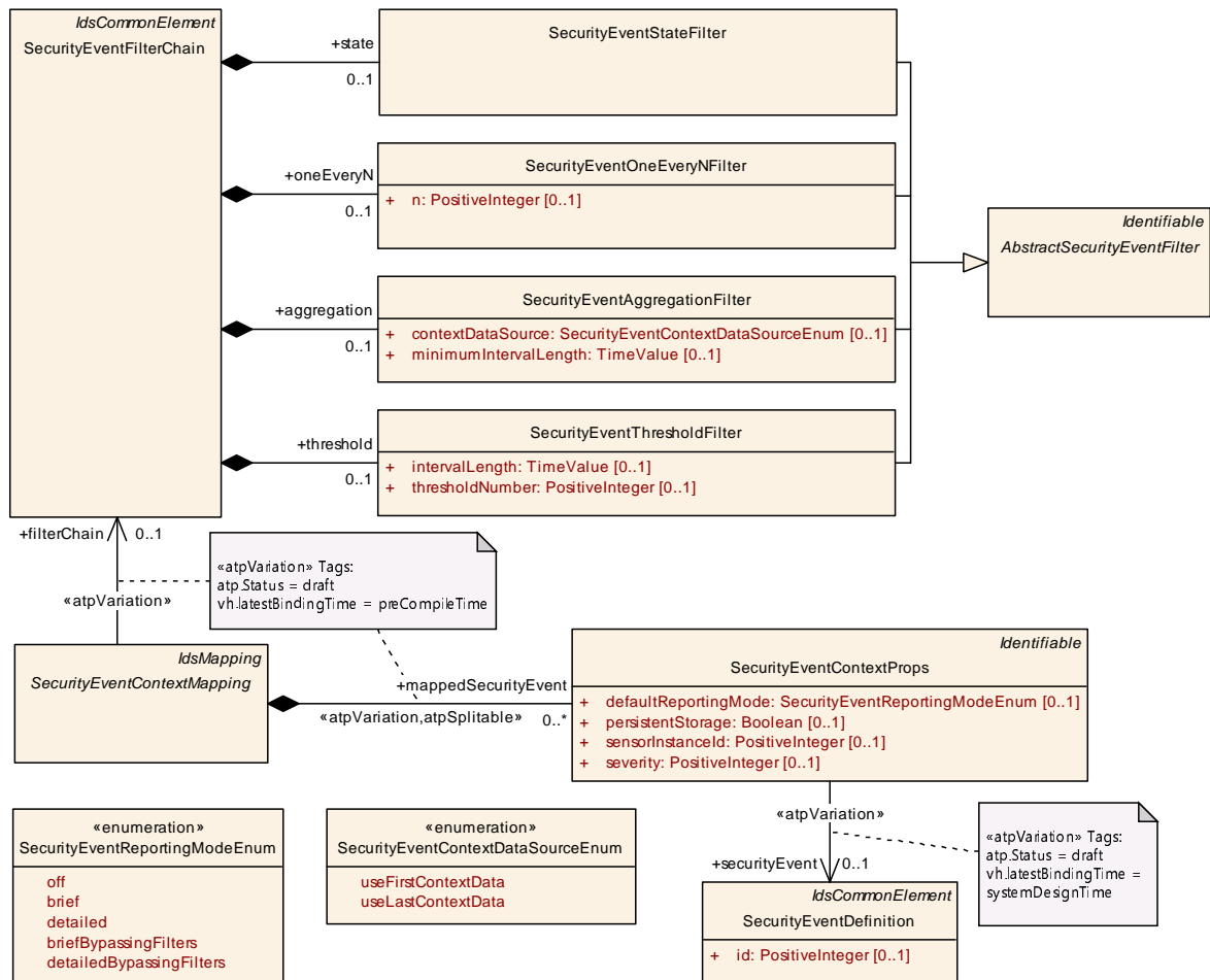
Figure 4.3: Modeling of SecurityEventFilterChain
