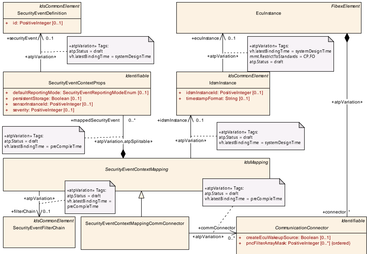
Figure 4.11: Modeling of SecurityEventContextMappingCommConnector
