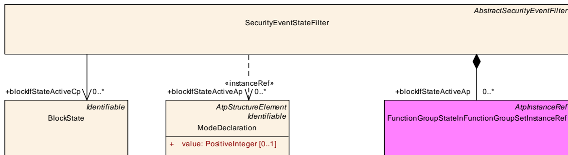
Figure 4.4: Modeling overview of the SecurityEventStateFilter
