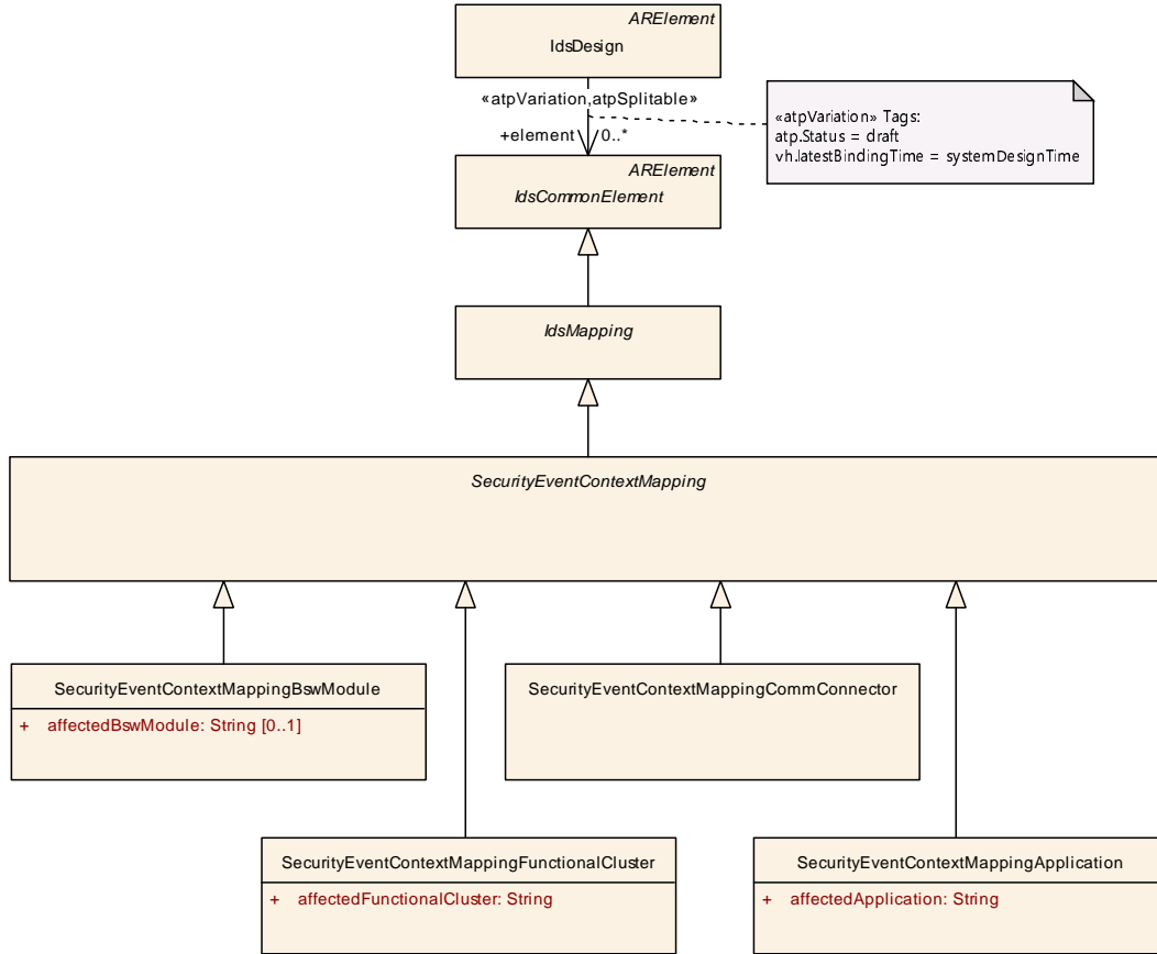
Figure 4.7: Meta-class hierarchy related to SecurityEventContextMapping
