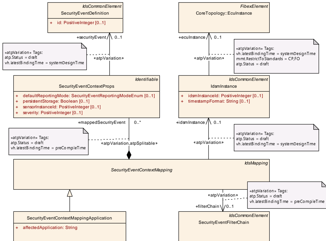
Figure 4.12: Modeling of SecurityEventContextMappingApplication
