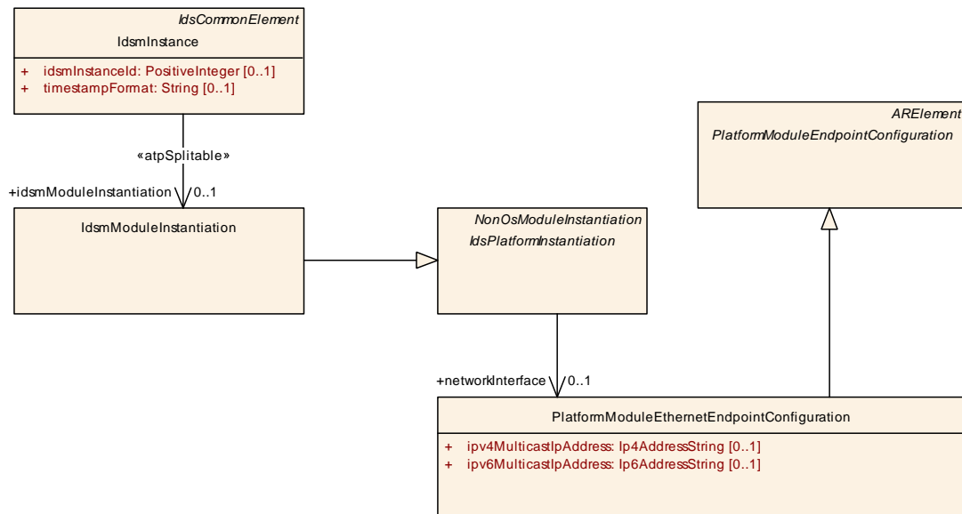
Figure 4.16: Modeling overview of the network configuration of an IdsmInstance on Adaptive Platform
