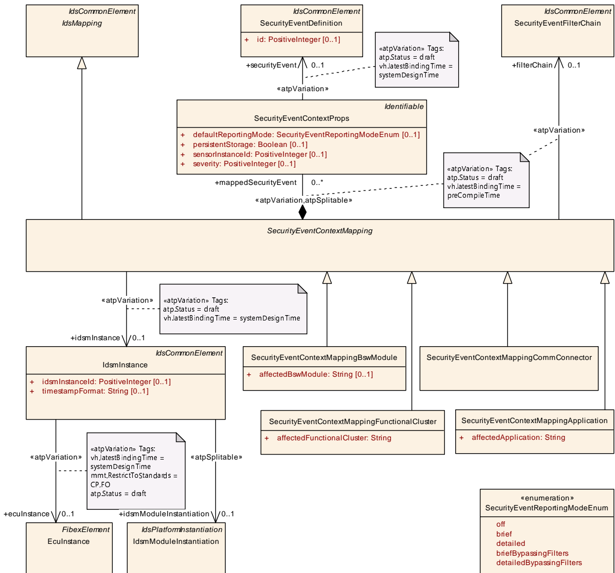
Figure 4.6: Modeling overview on mapping of security events
