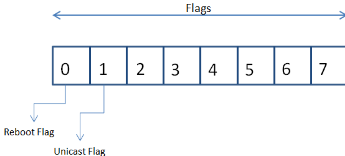
Figure 4.3: Flags in SOME/IP-SD
