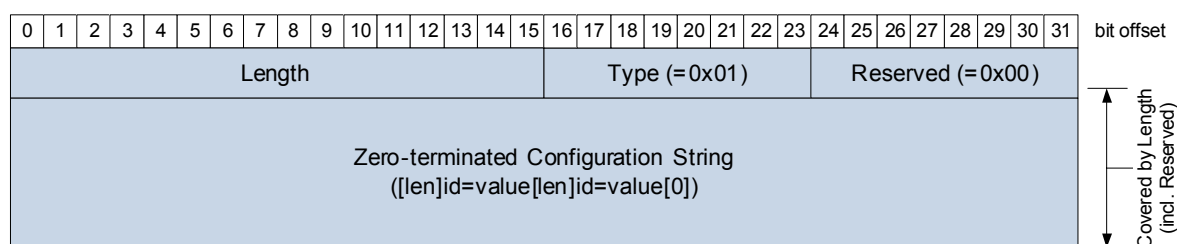
Figure 4.6: SOME/IP-SD Configuration Option
