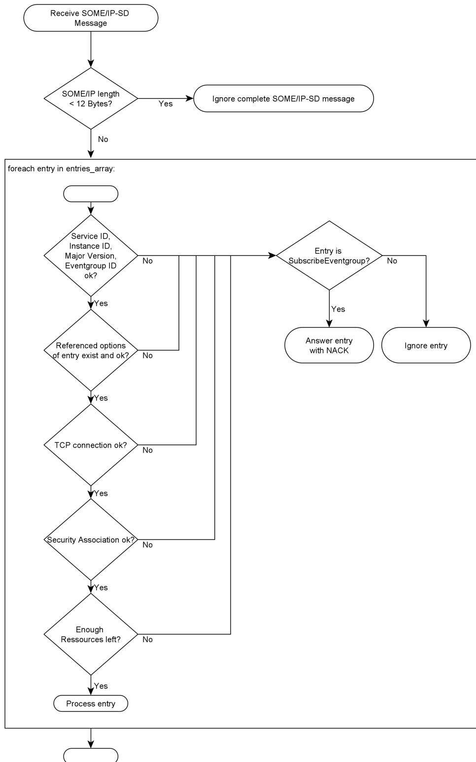
Figure 4.18: - SOME/IP-SD Error Handling
