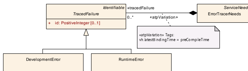
Figure 13.6: Modeling of ErrorTracerNeeds
