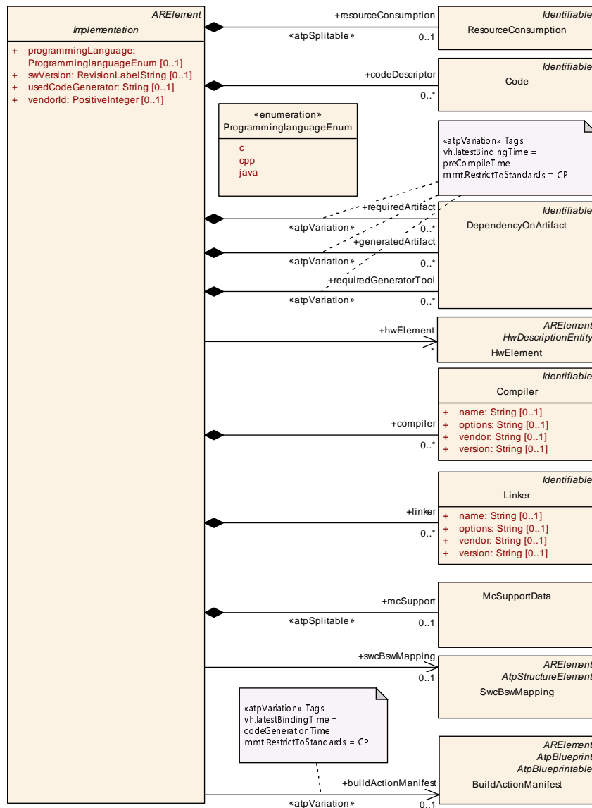
Figure 8.1: Overview of implementation description
