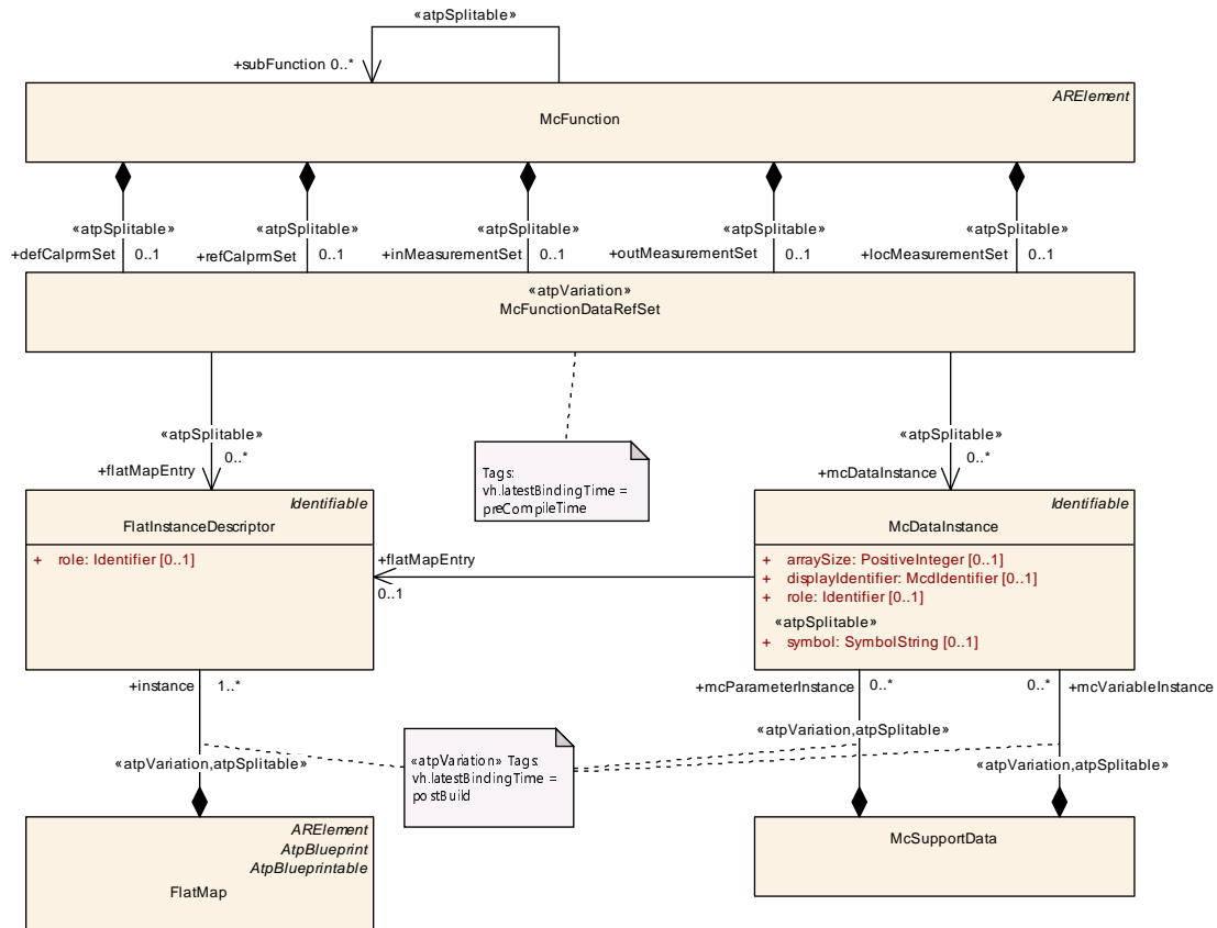
Figure 10.5: Meta-model for McFunction
