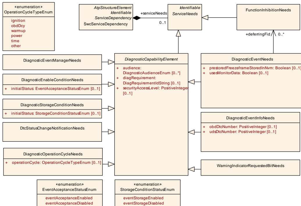
Figure 13.5: Class ServiceNeeds from CommonStructure and derived classes for diagnosis use cases
