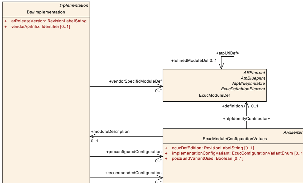
Figure 11.5: Variation points under BswImplementation
