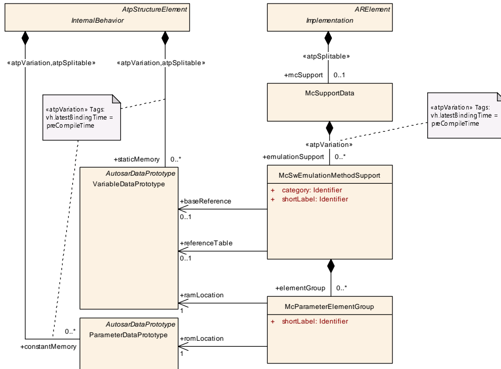
Figure 10.3: Describing the Software Emulation Method for Calibration Data
