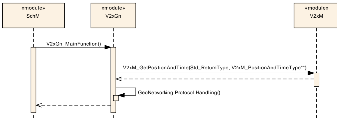
Figure 5 – V2xGn_MainFunction
